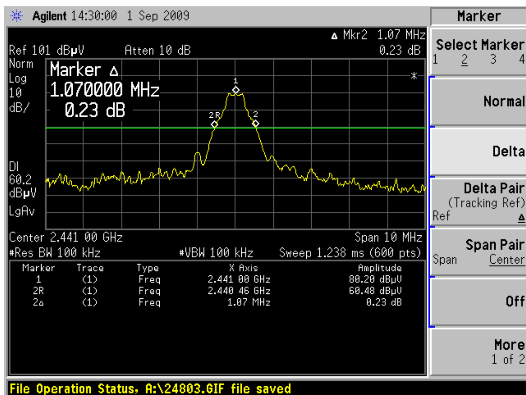
Channel 40_2441 MHz
