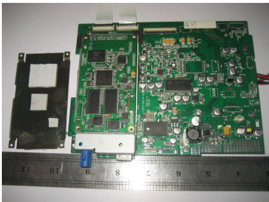
Uncovered the shielded of PCB 3
