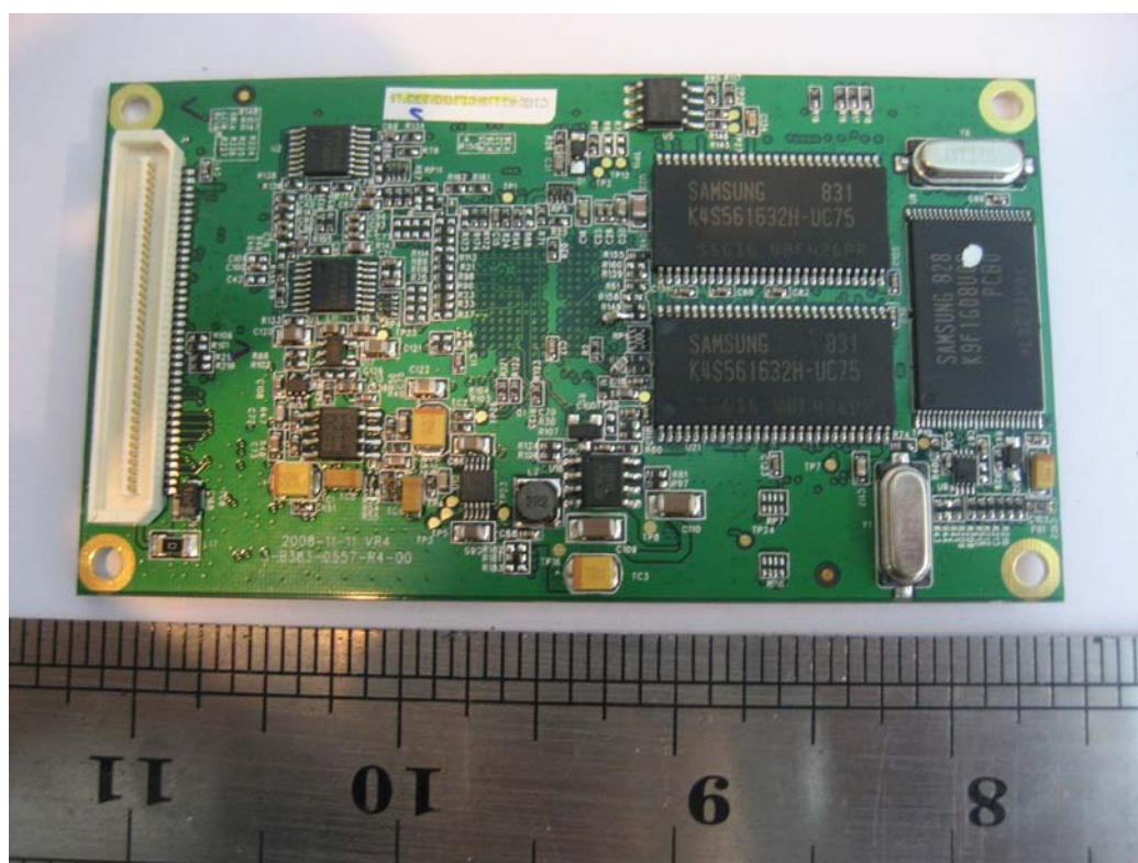
Back view of PCB4
