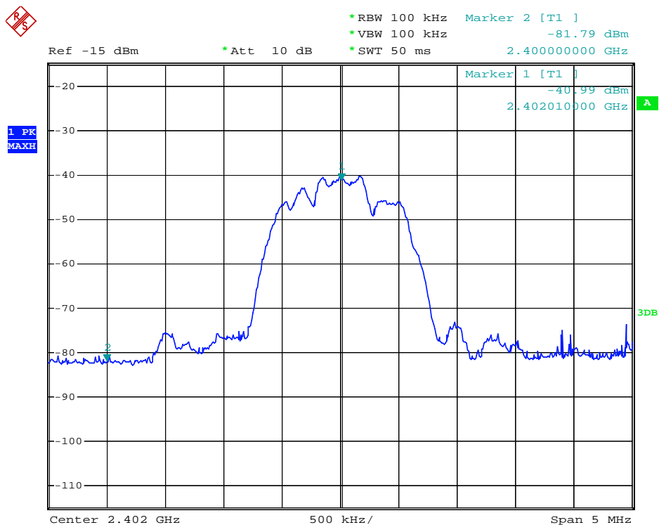
CH1_2402MHz
