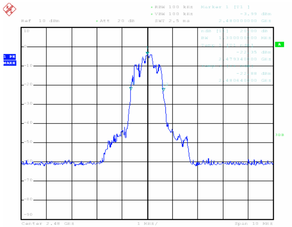
Channel 79_ 2480 MHz
