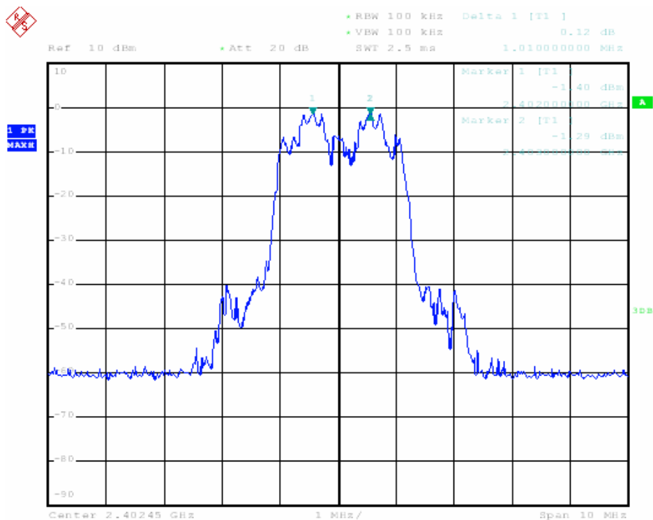
Channel 1_2402 MHz
