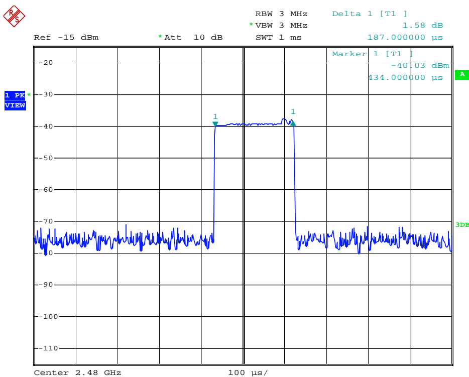
Channel 79_ 2480 MHz
