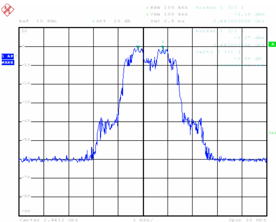
Channel 40_2441 MHz
