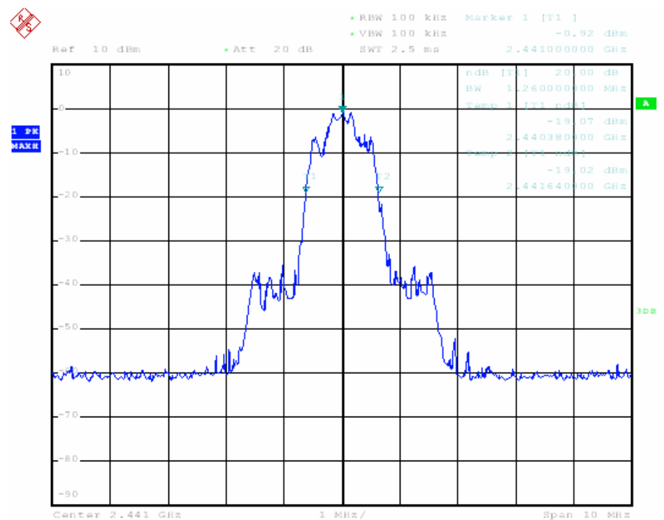
Channel 40_2441 MHz
