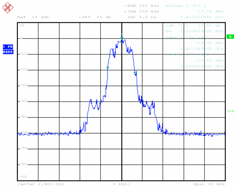
Channel 1_2402 MHz
