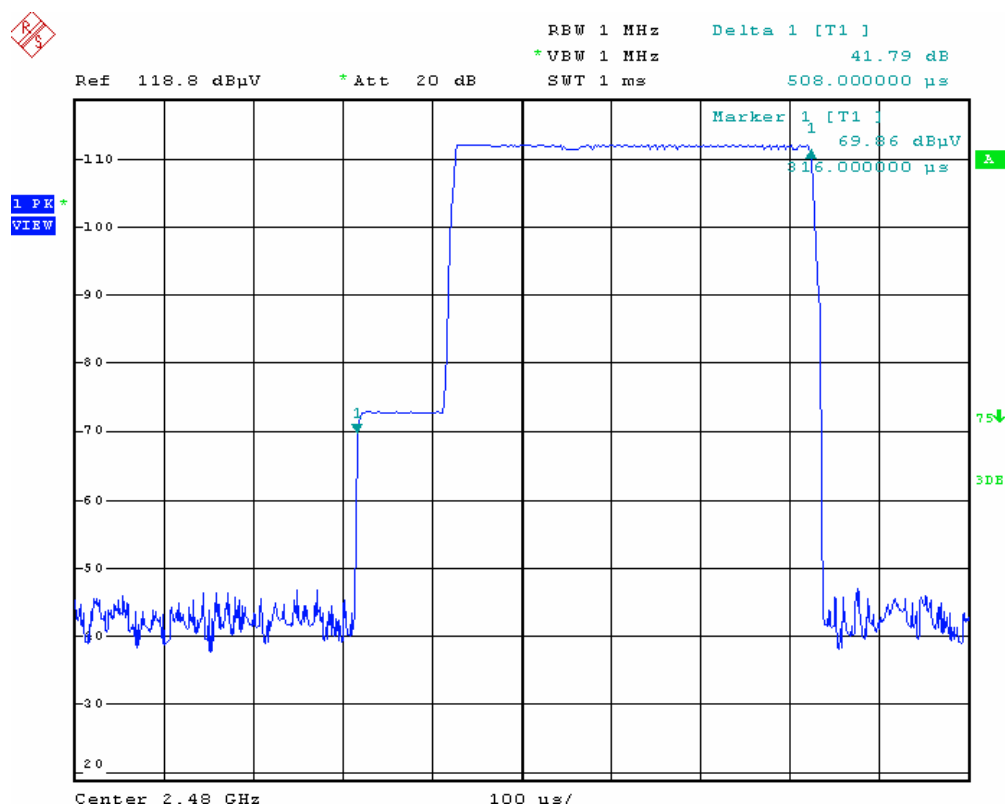
Channel 79_ 2480 MHz
