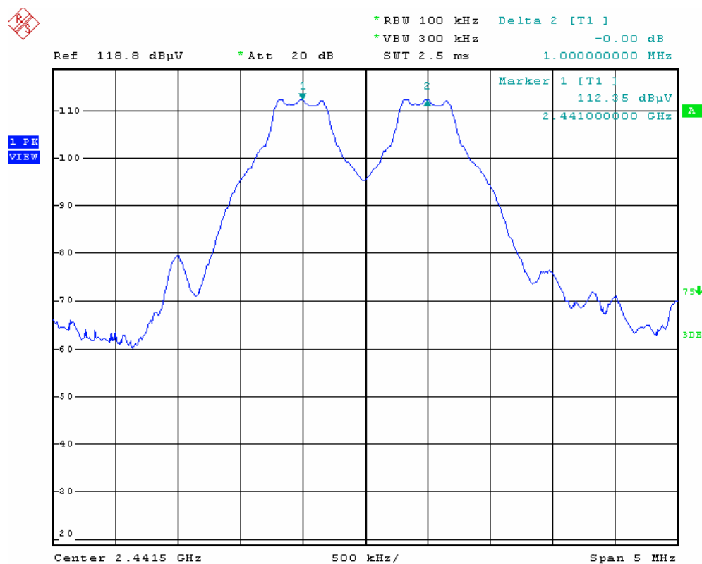
Channel 40_2441 MHz
