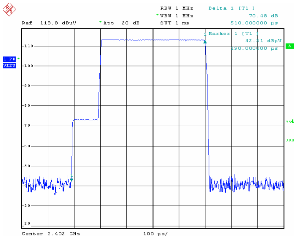
Channel 1_ 2402 MHz
