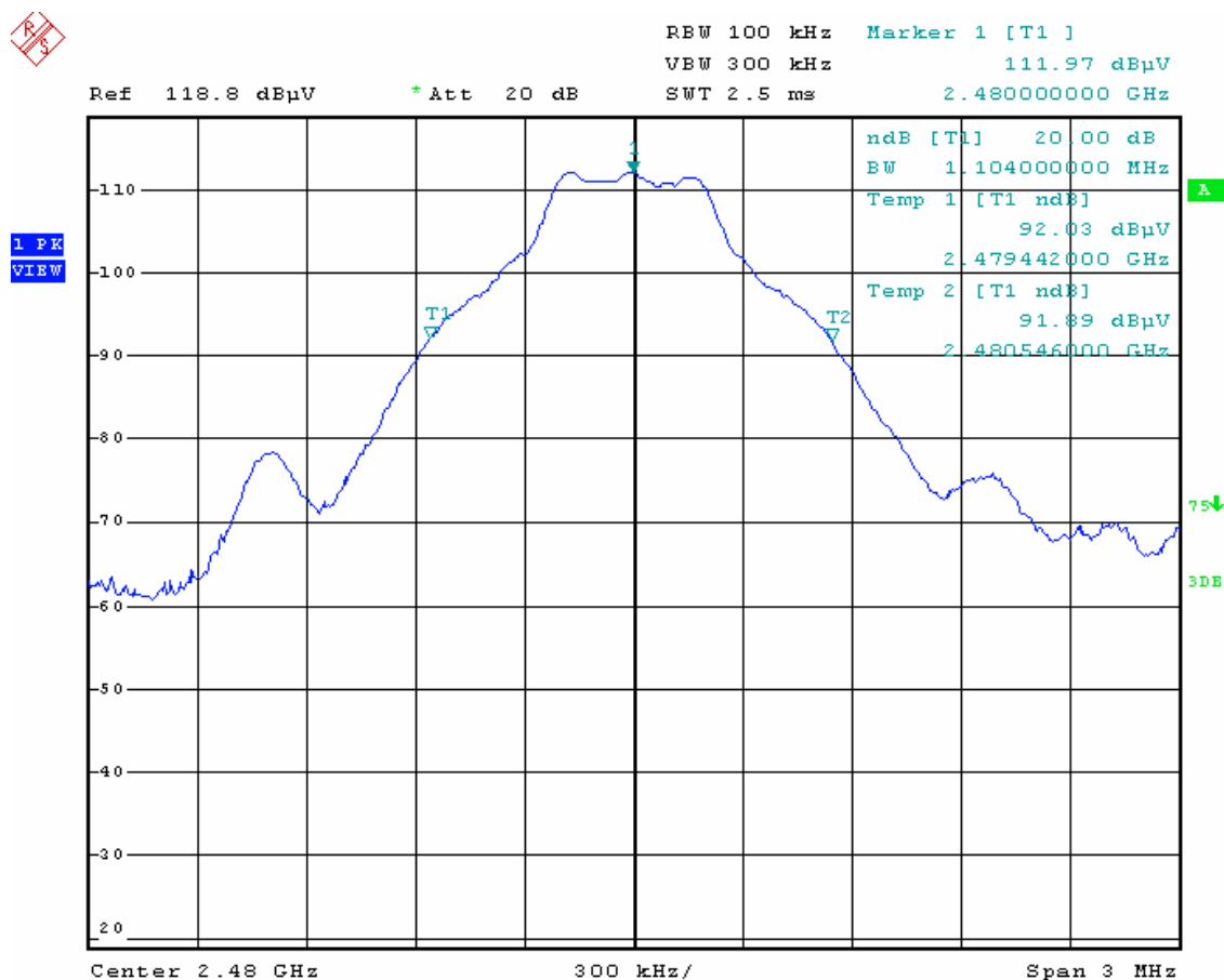
Channel 79_ 2480 MHz
