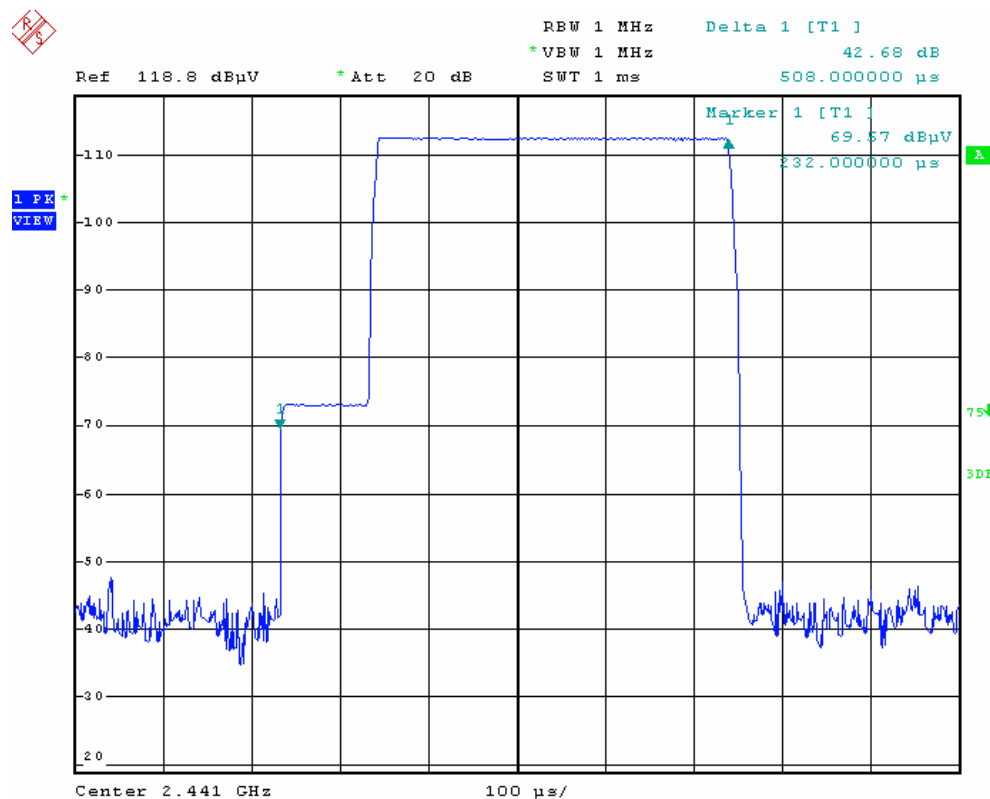
Channel 40_2441 MHz
