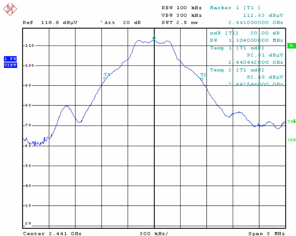
Channel 40_2441 MHz
