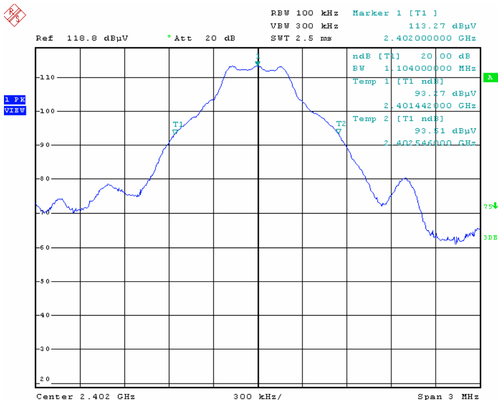
Channel 1_2402 MHz
