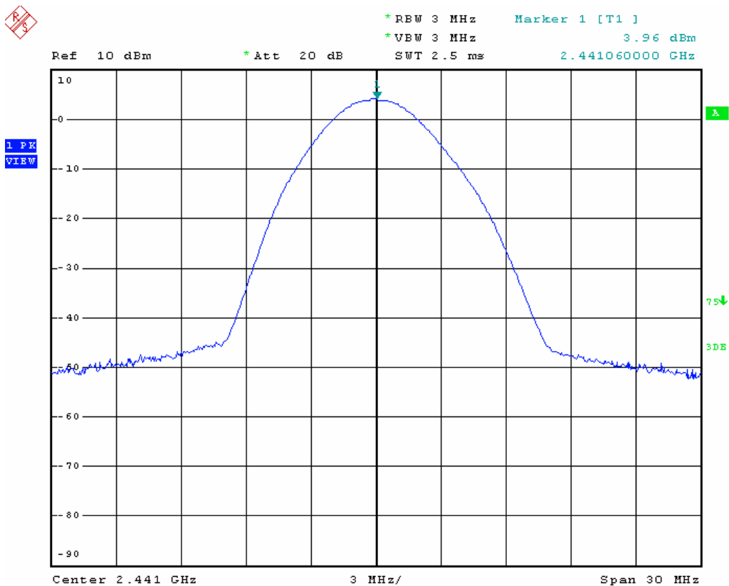
CH40_2441MHz
