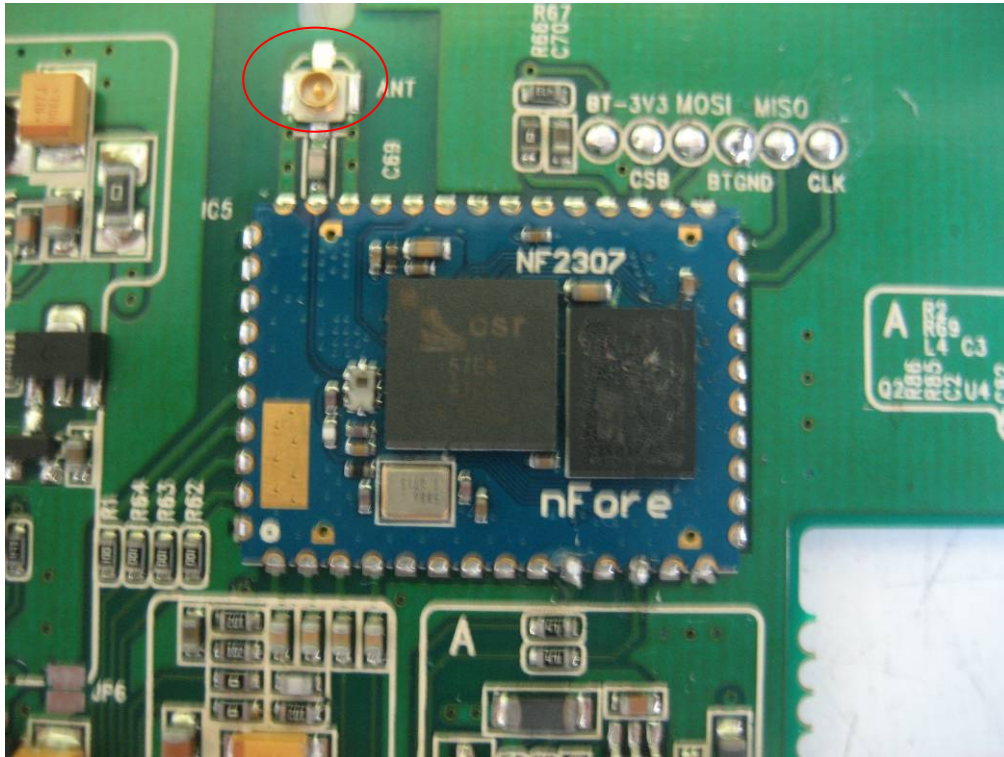
BT Antenna Location-1
