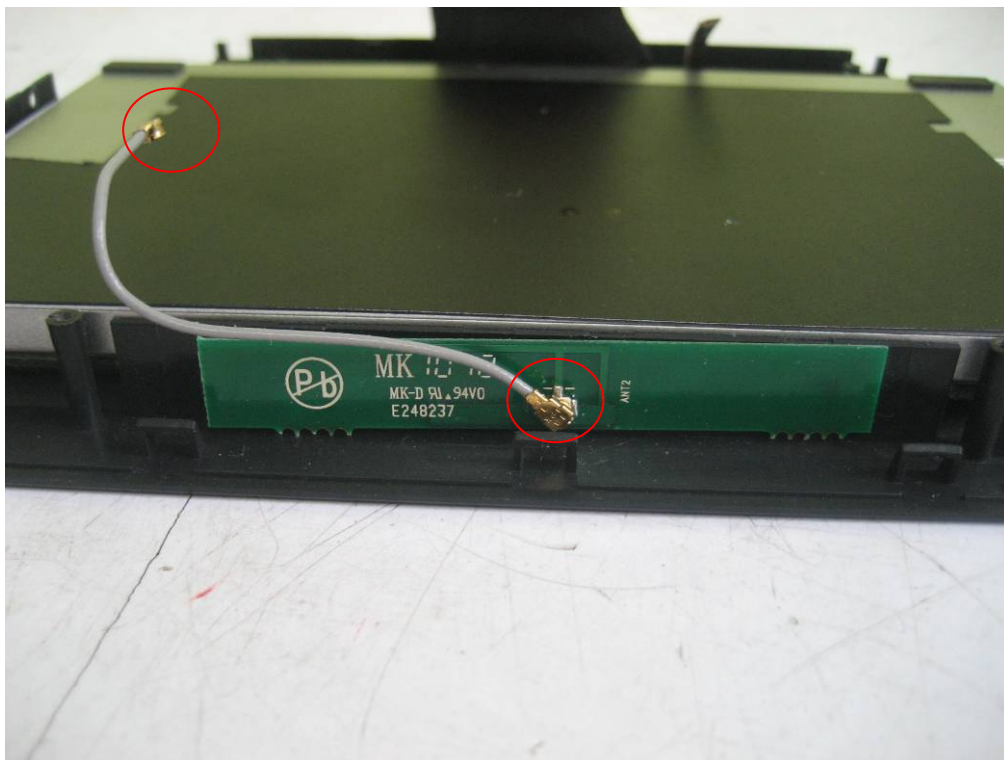
BT Antenna Location-2
