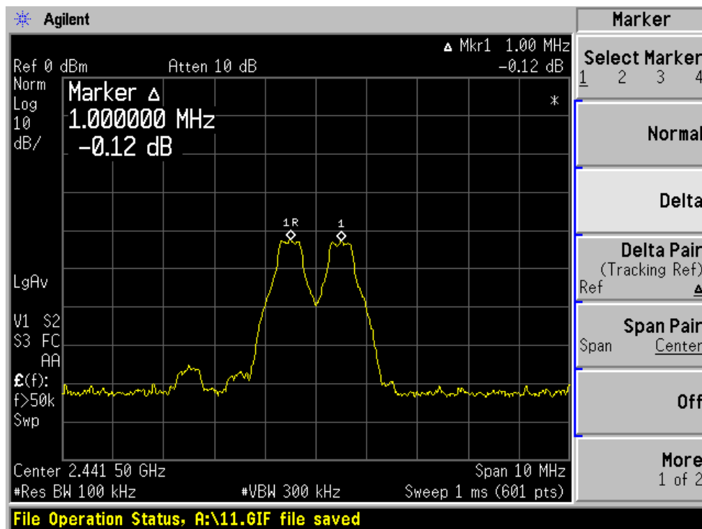
Channel 40_ 2441 MHz
