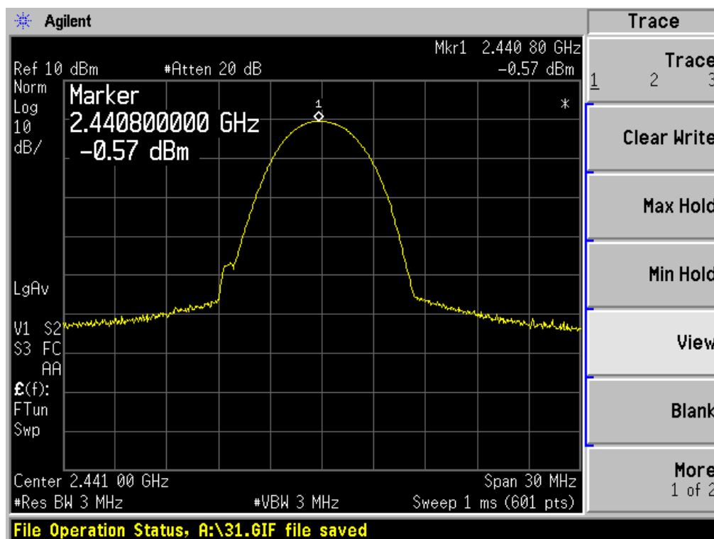
CH40 _ 2441MHz
