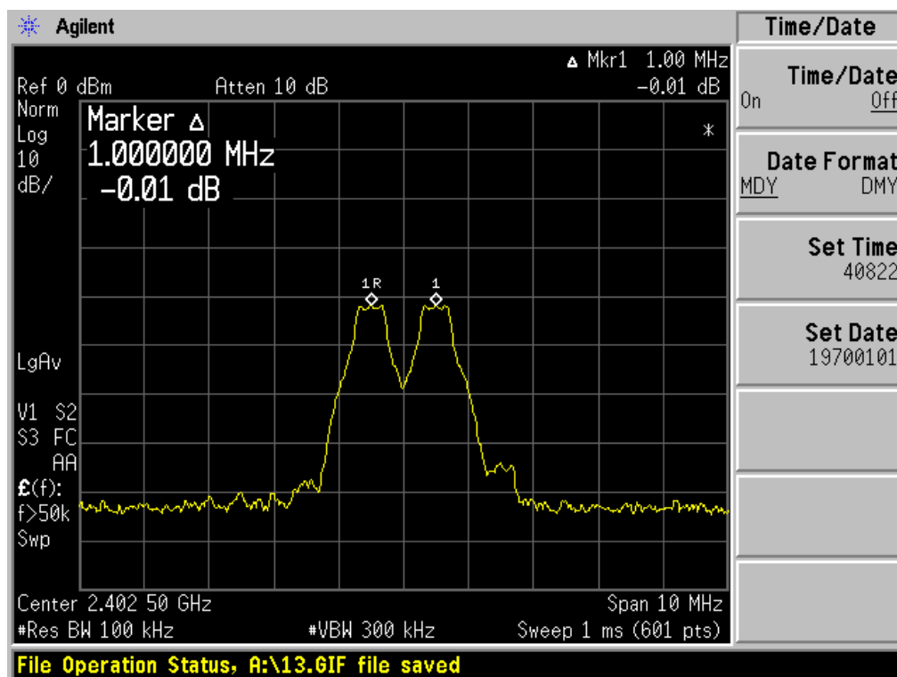
Channel 1_ 2402 MHz
