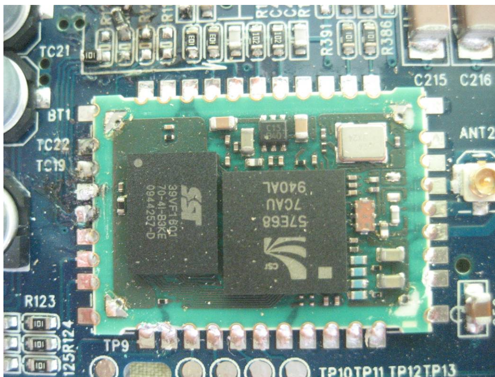
Internal View of Bluetooth Module
