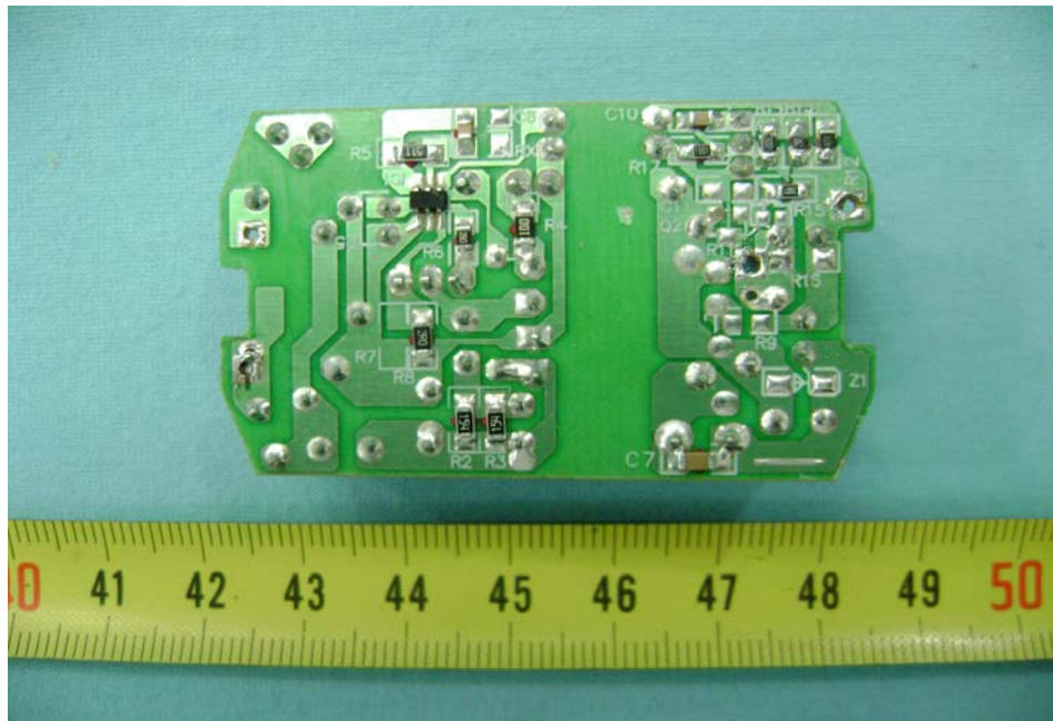
PCB(Adapter) - Back View
