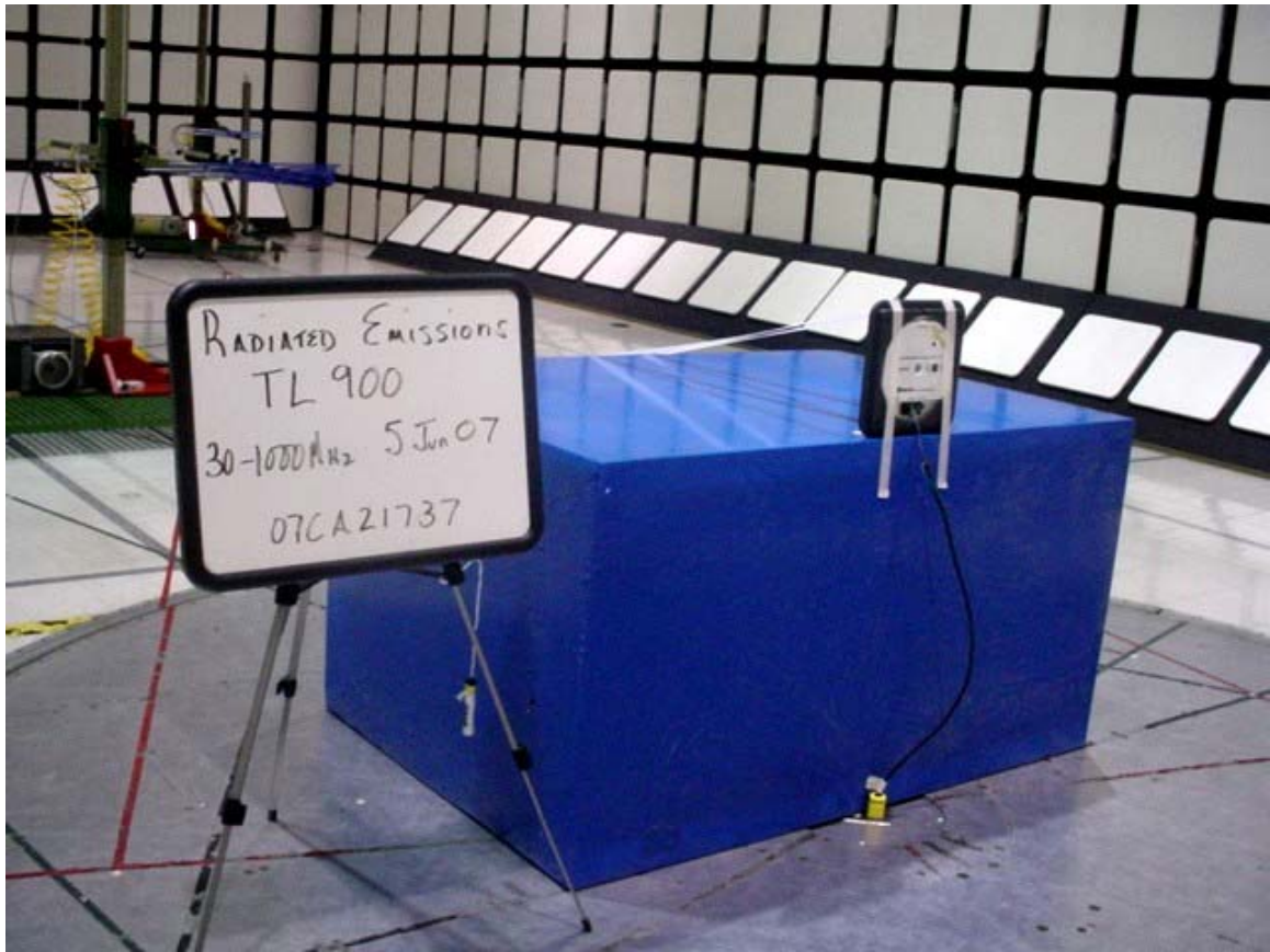
Radiated Emissions test set up 30MHz-1GHz Front View
