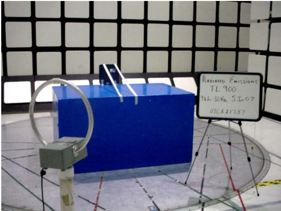
Radiated Emissions test set up 9KHz-30MHz Front View
