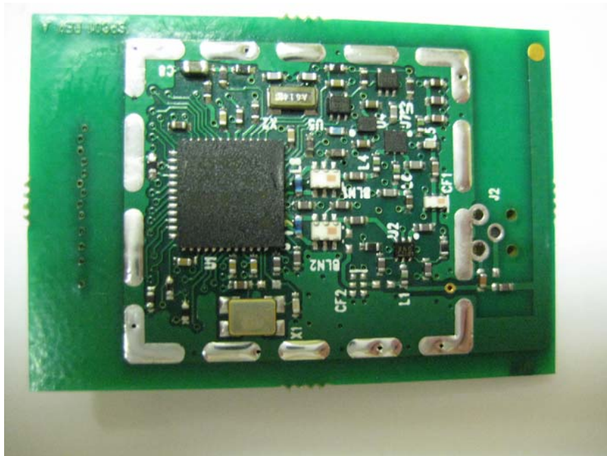
View #2, Close up of Module RF Section (Shield removed)
