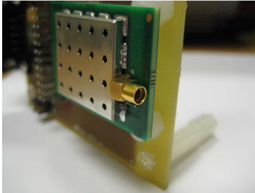
View #2 Close Up of Antenna Connector
