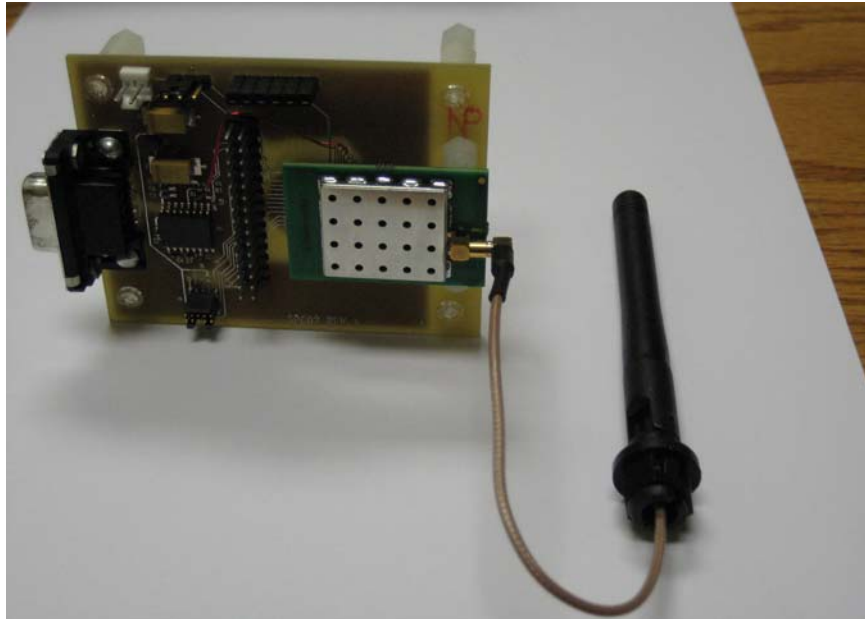
View of External Antenna connected to module
