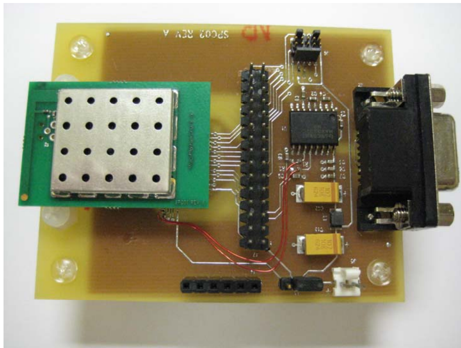
View #2 - Module attached to Board (note 1)
