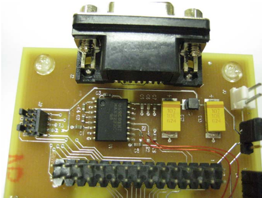
View of Front of Board – without Module (note 1)
