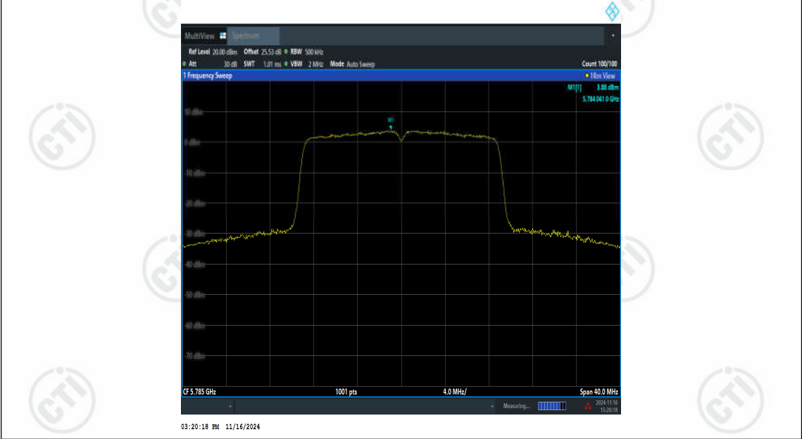
11AC20SISO-Ant2-5785-PASS
