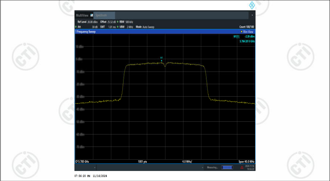
11AC20MIMO-Ant3-5785-PASS
