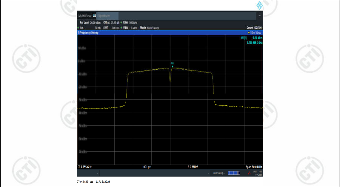
11N40MIMO-Ant3-5755-PASS
