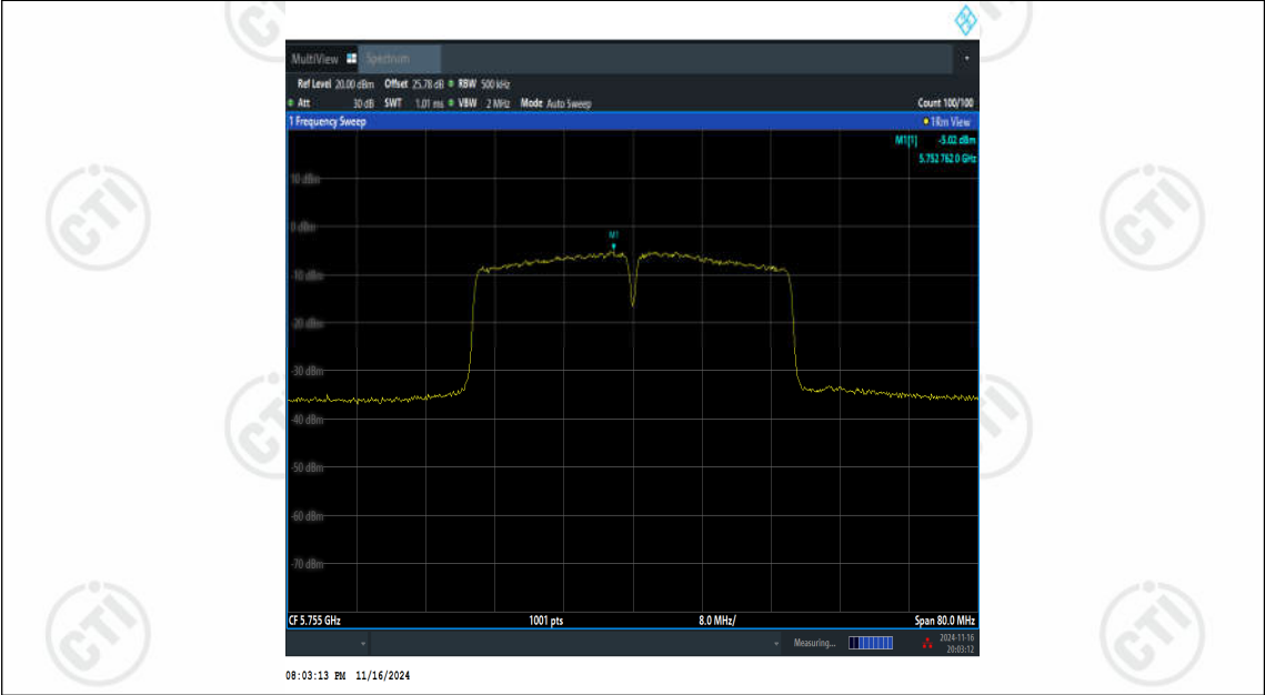
11AC40MIMO-Ant3-5755-PASS
