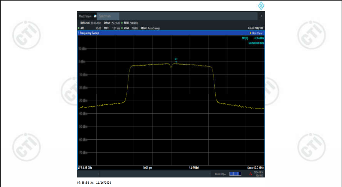
11N20MIMO-Ant3-5825-PASS
