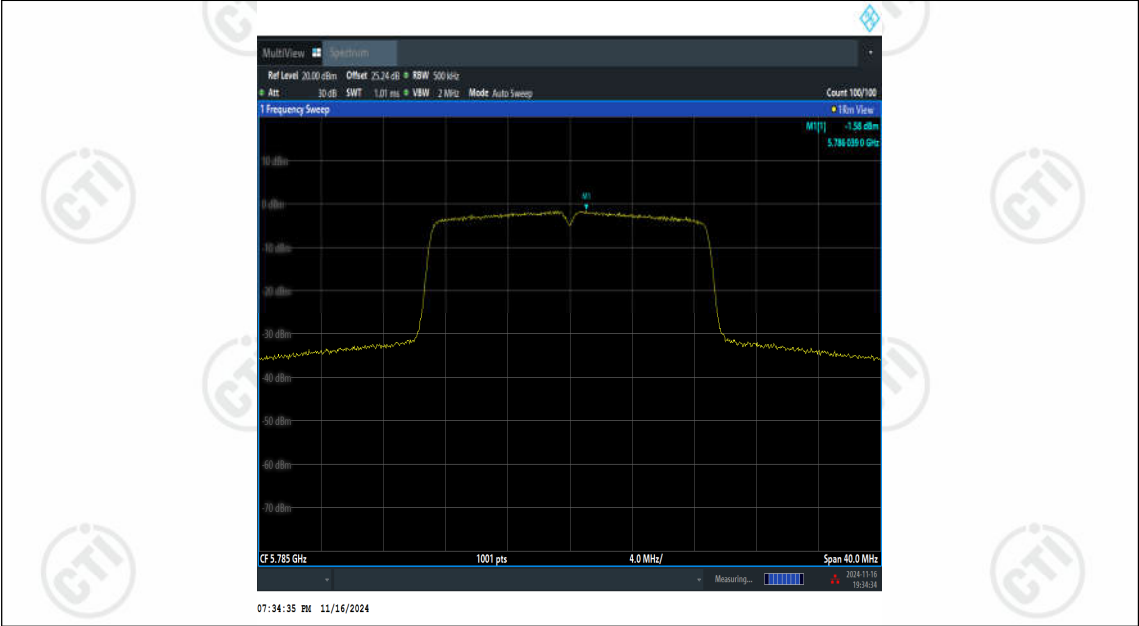
11N20MIMO-Ant3-5785-PASS
