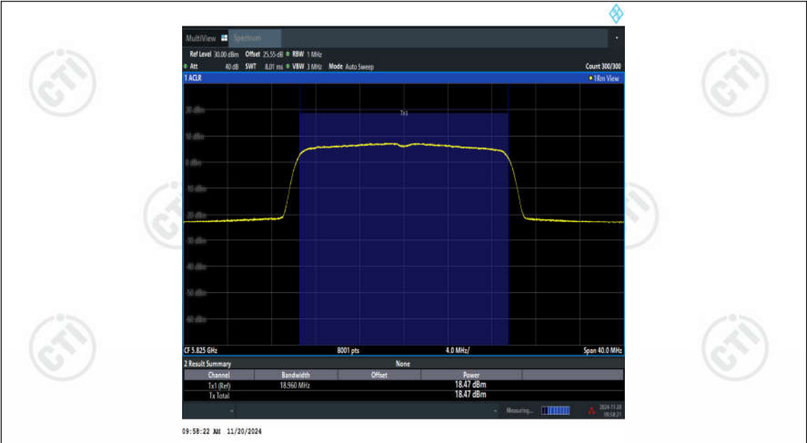
11BE20SISO-Ant2-5825-PASS
