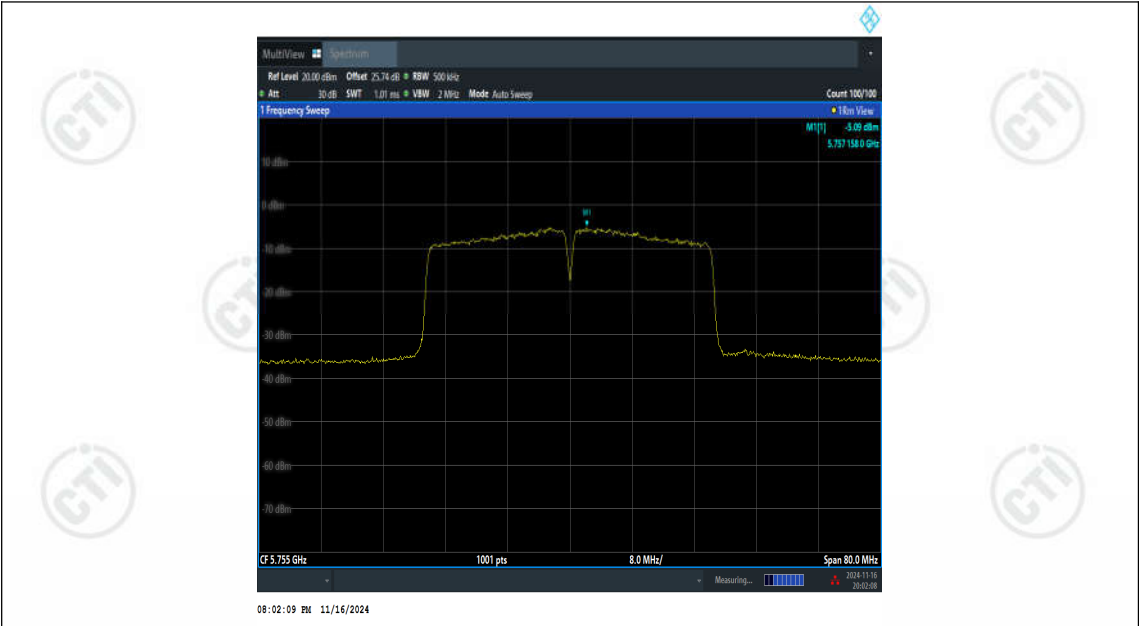
11AC40MIMO-Ant2-5755-PASS
