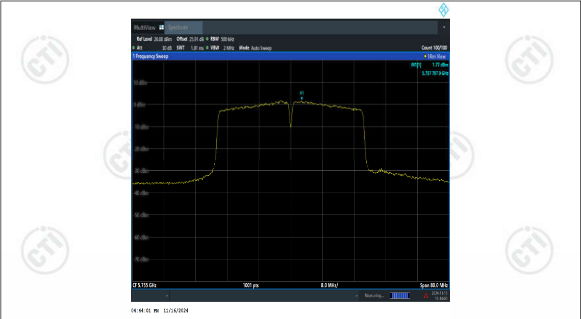
11AC40SISO-Ant2-5755-PASS
