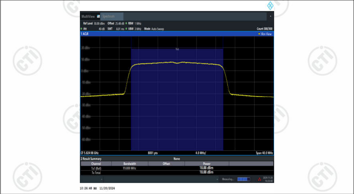
11BE20SISO-Ant3-5825-PASS
