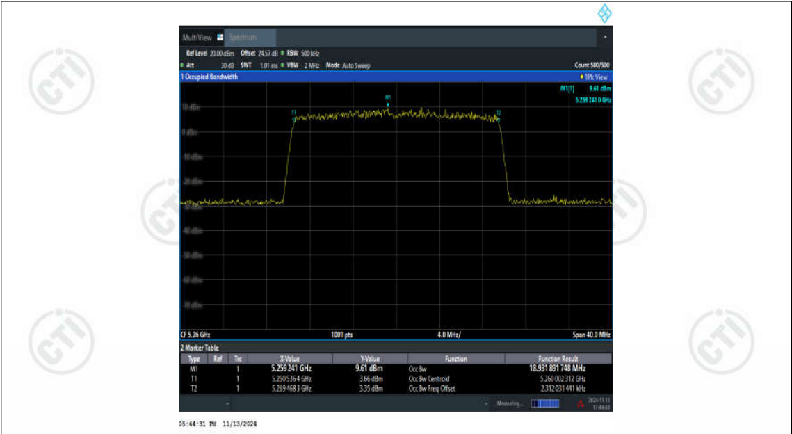
11AX20SISO-Ant1-5260
