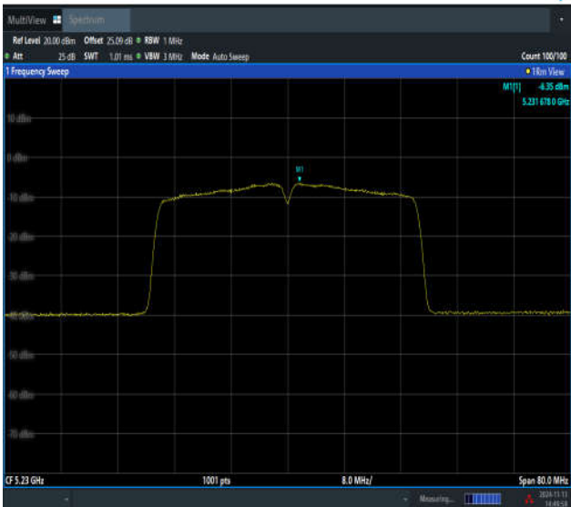
11N40MIMO-Ant2-5230-PASS
