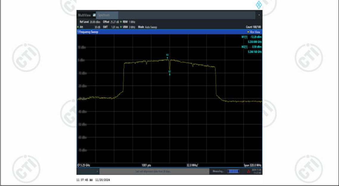
11BE160SISO-Ant3-5250_UNII-1-PASS
