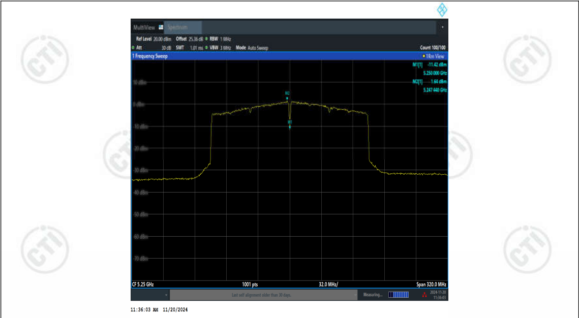
11BE160SISO-Ant2-5250_UNII-1-PASS
