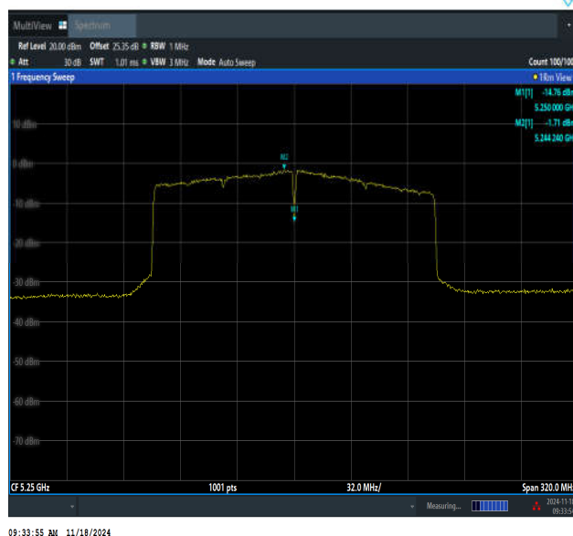
11AX160SISO-Ant1-5250 UNII-1-PASS
