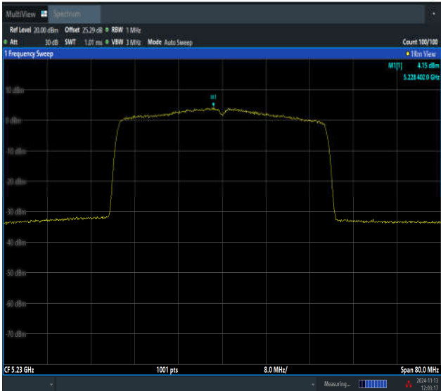
11AX40SISO-Ant3-5230-PASS
