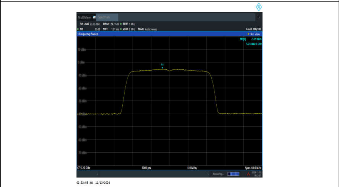
11N20MIMO-Ant1-5220-PASS
