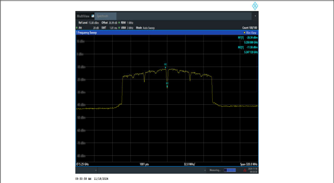
11AC160MIMO-Ant2-5250_UNII-1-PASS
