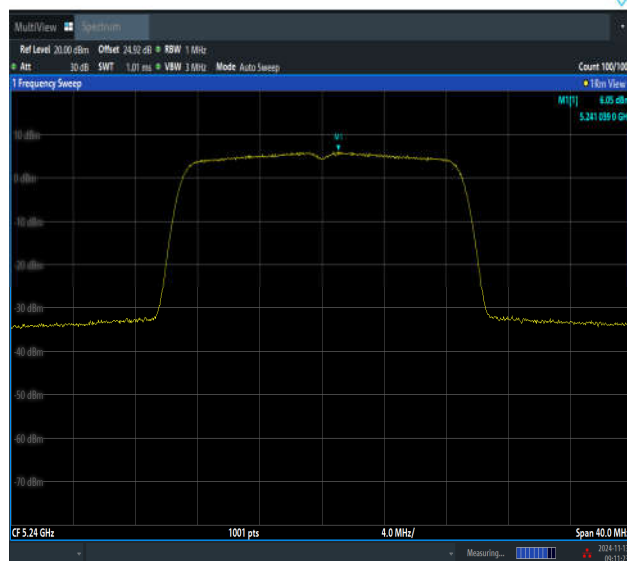
11N20SISO-Ant2-5240-PASS
