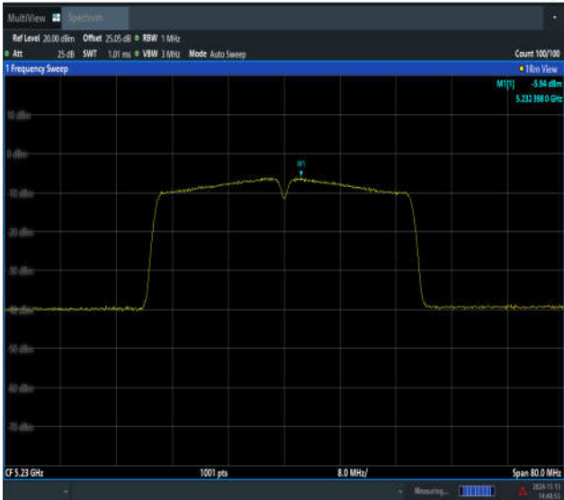
11N40MIMO-Ant1-5230-PASS
