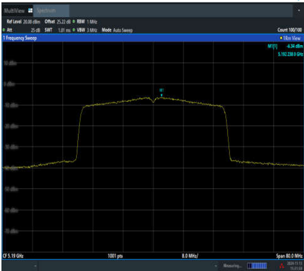
11AX40MIMO-Ant1-5190-PASS
