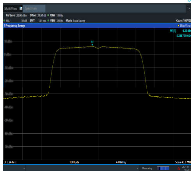
11N20SISO-Ant3-5240-PASS
