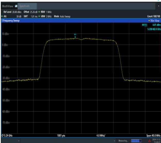
11AC20SISO-Ant3-5240-PASS
