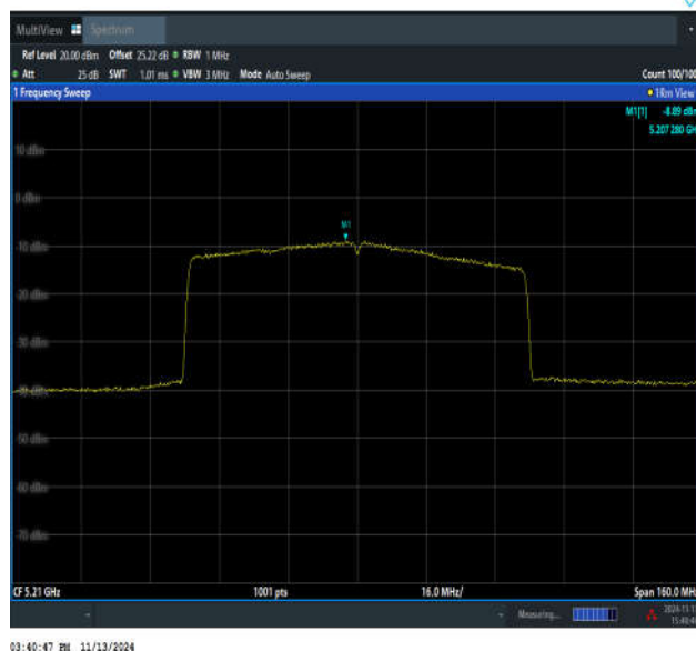
11AX80MIMO-Ant3-5210-PASS
