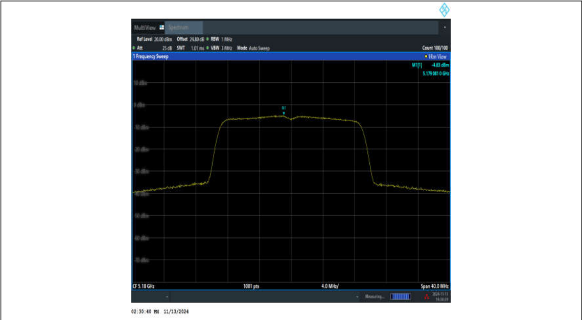
11N20MIMO-Ant3-5180-PASS
