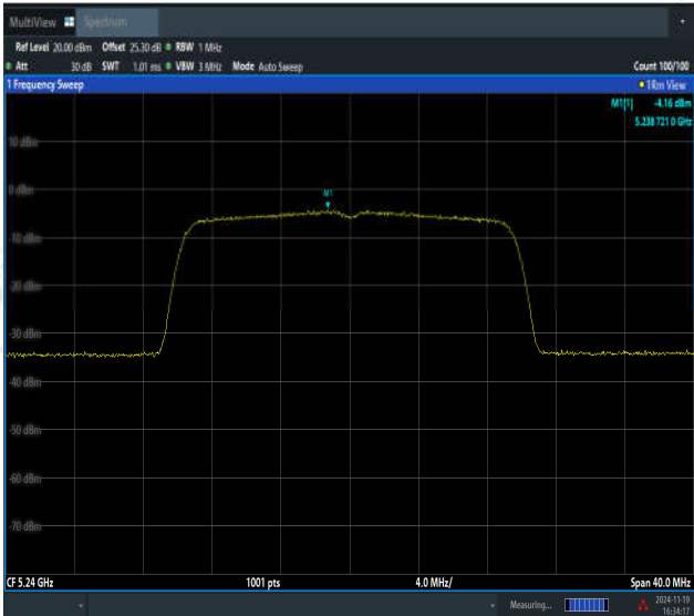
11BE20MIMO-Ant1-5240-PASS
