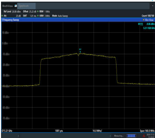
11AX80MIMO-Ant2-5210-PASS
