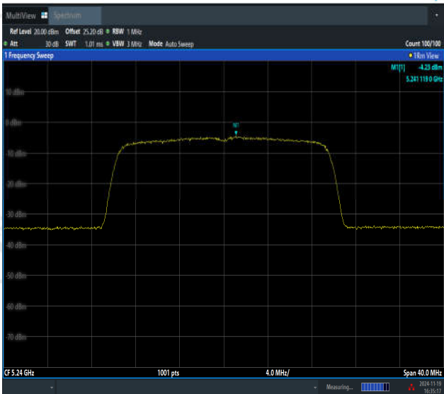
11BE20MIMO-Ant2-5240-PASS
