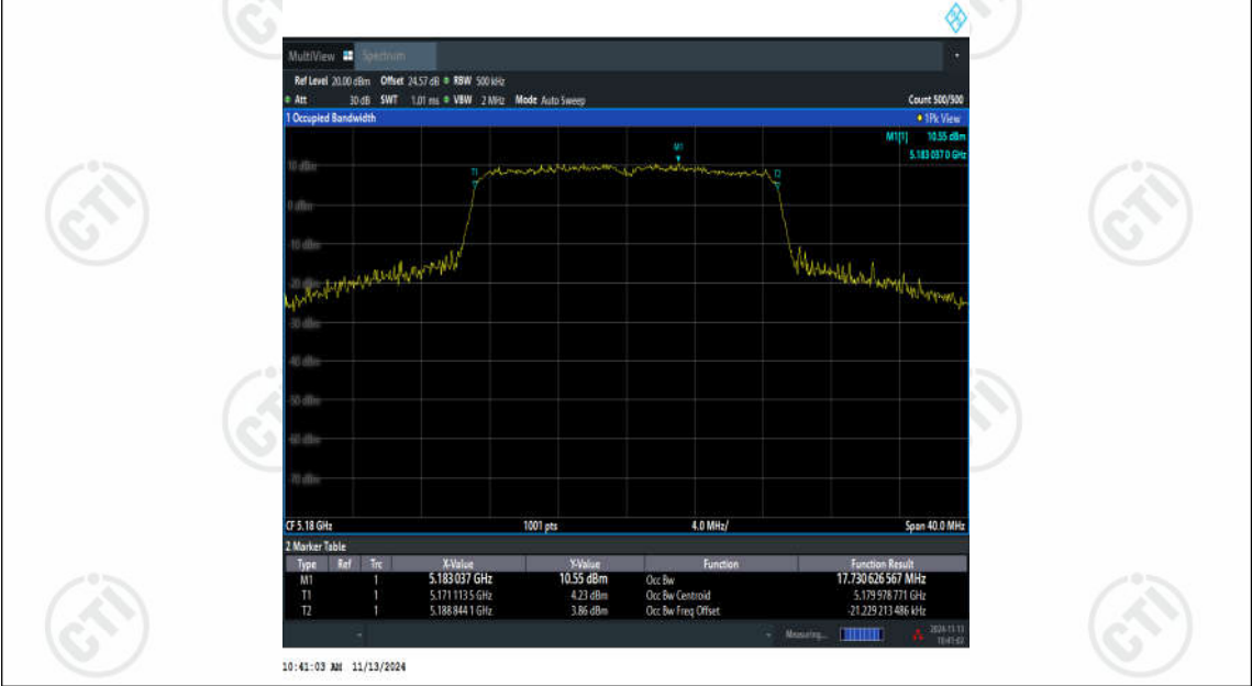
11N20SISO-Ant3-5180
