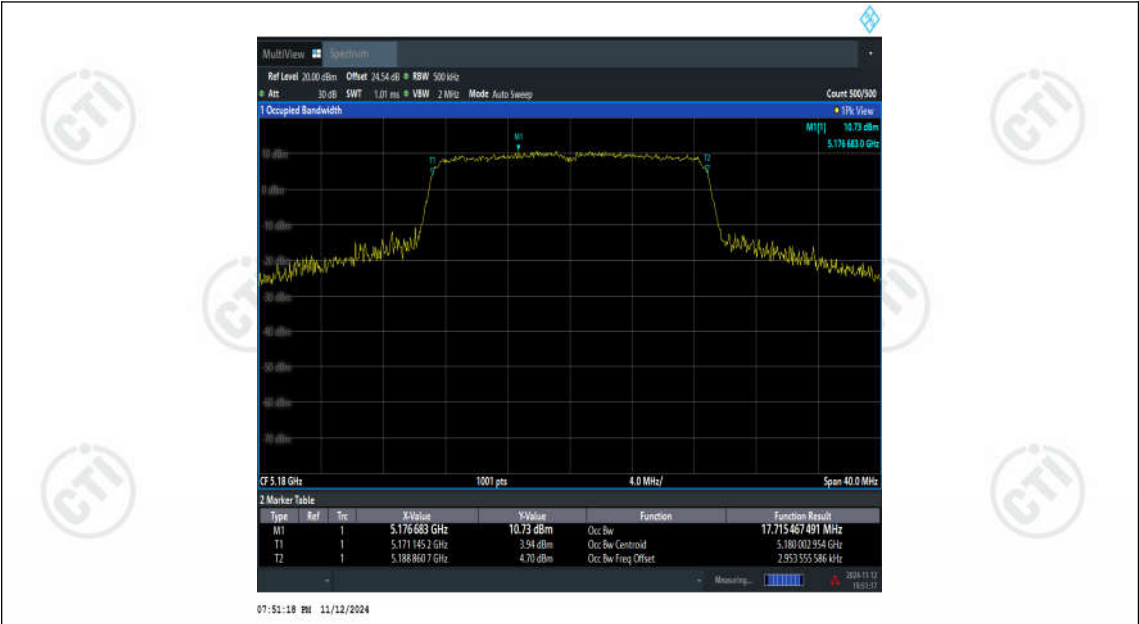
11N20SISO-Ant2-5180
