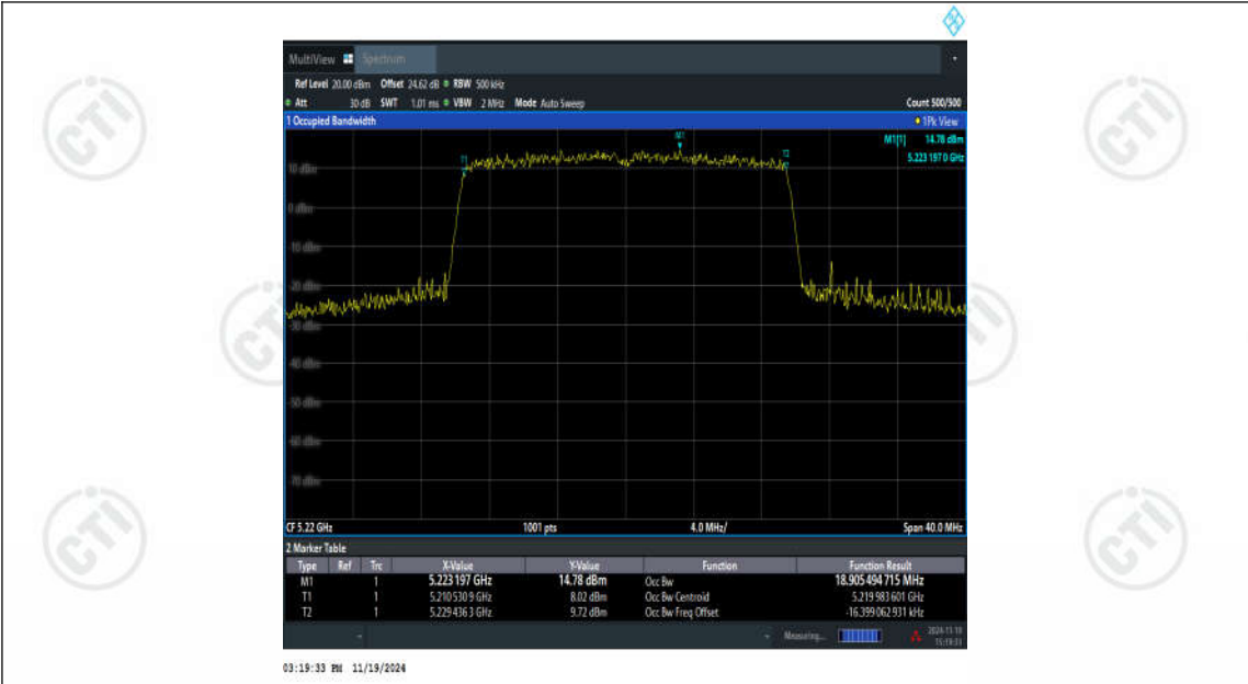
11BE20SISO-Ant2-5220
