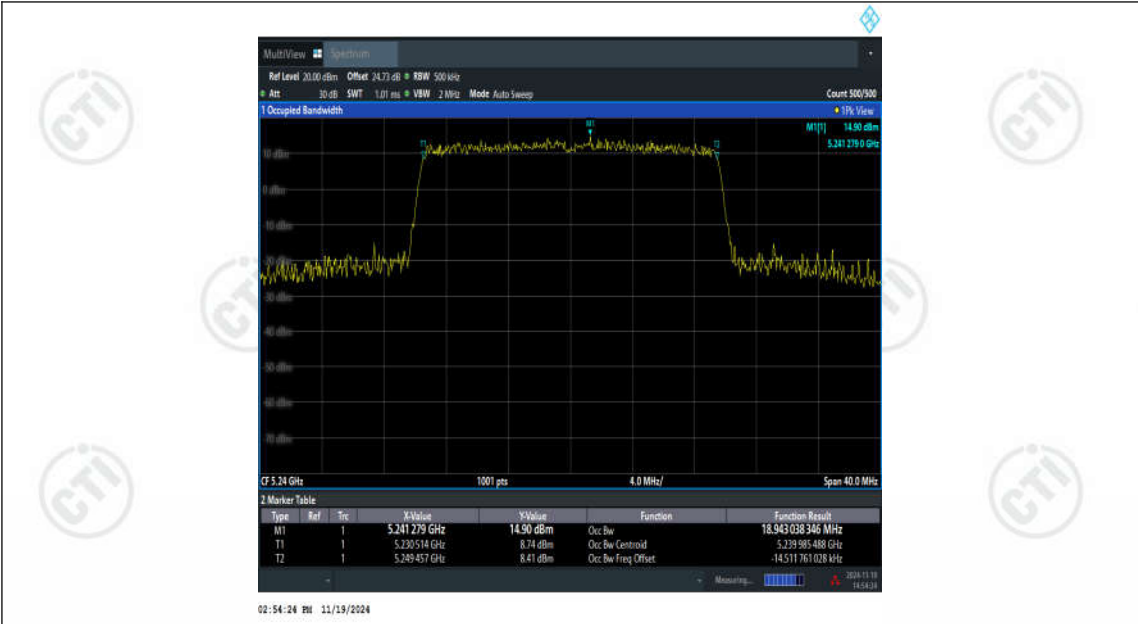
11BE20SISO-Ant1-5240
