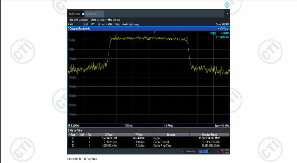
11BE20SISO-Ant3-5220
