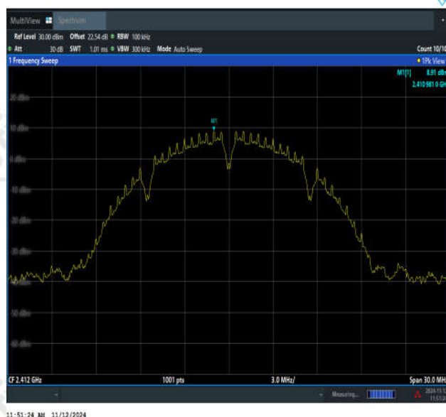
11B-Ant1-2412-0~Reference-PASS
