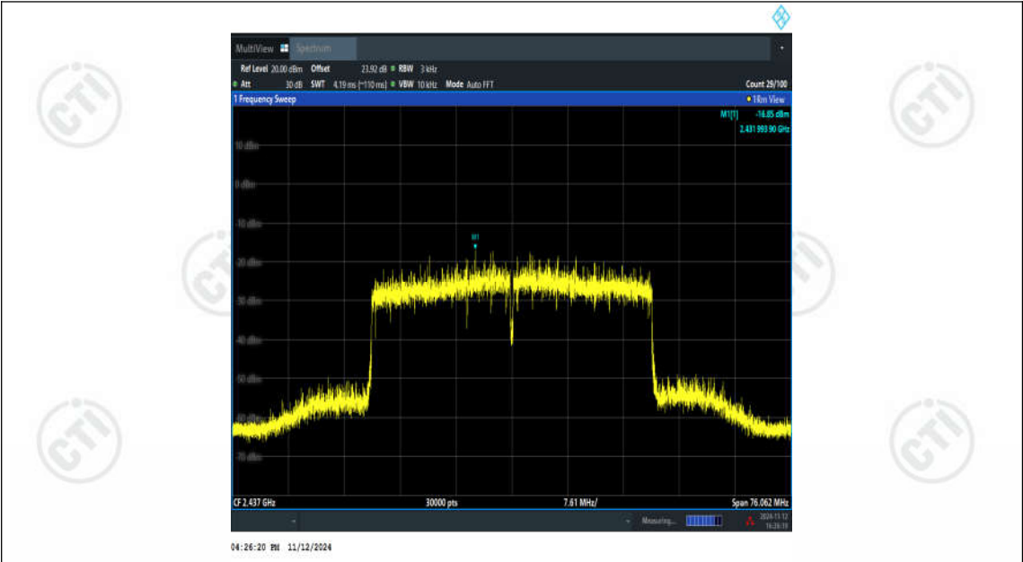
11BE40SISO-Ant1-2437-PASS
