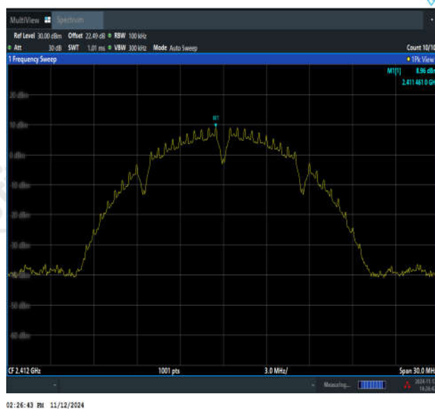
11B-Ant2-2412-0~Reference-PASS
