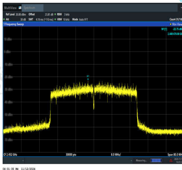
11AX40MIMO-Ant1-2452-PASS
