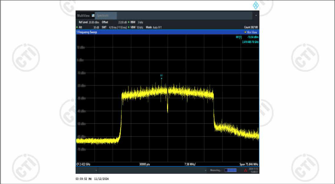
11AX40SISO-Ant2-2422-PASS
