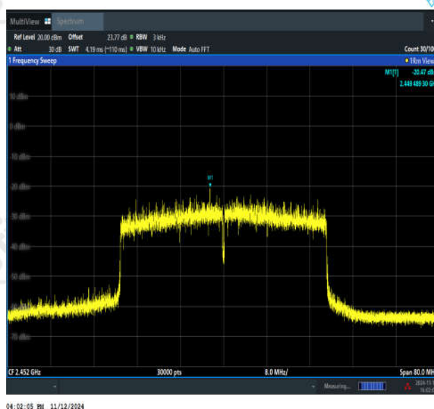
11AX40MIMO-Ant2-2452-PASS
