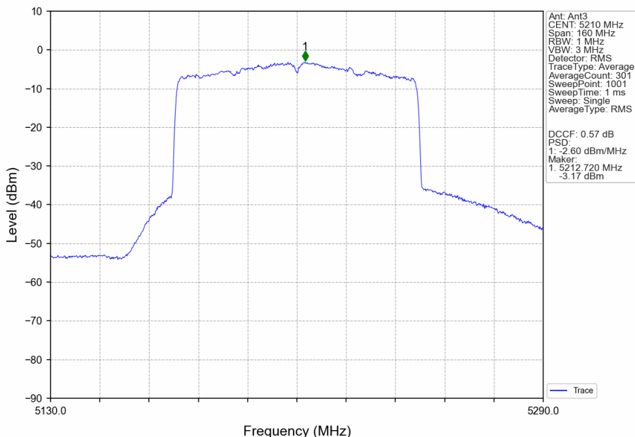
802.11ax(HEW80)_MCH_5210MHz_SU_/_MIMO_NTNV
