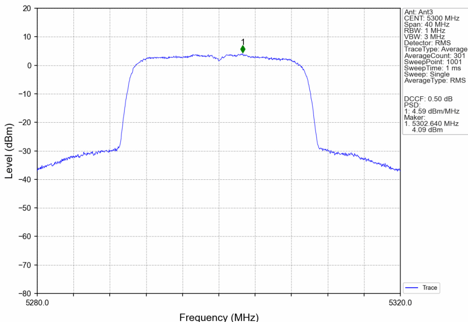
802.11ax(HEW20)_MCH_5300MHz_SU_/_MIMO_NTNV
