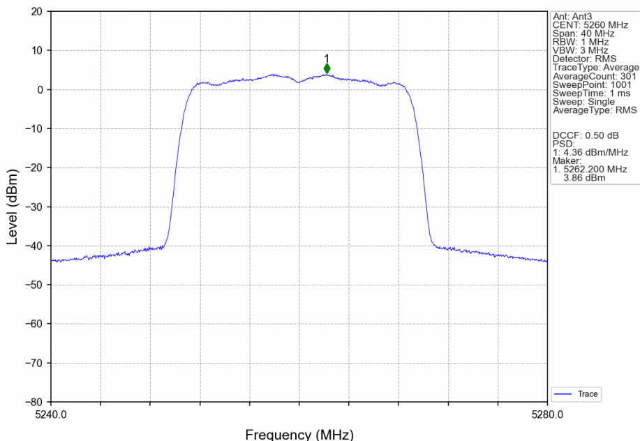
802.11ac(VHT20)_LCH_5260MHz_MIMO_NTNV
