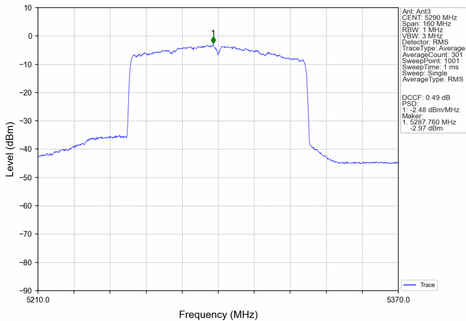
802.11ax(HEW80)_MCH_5290MHz_SU_ / _Ant3_NTNV
