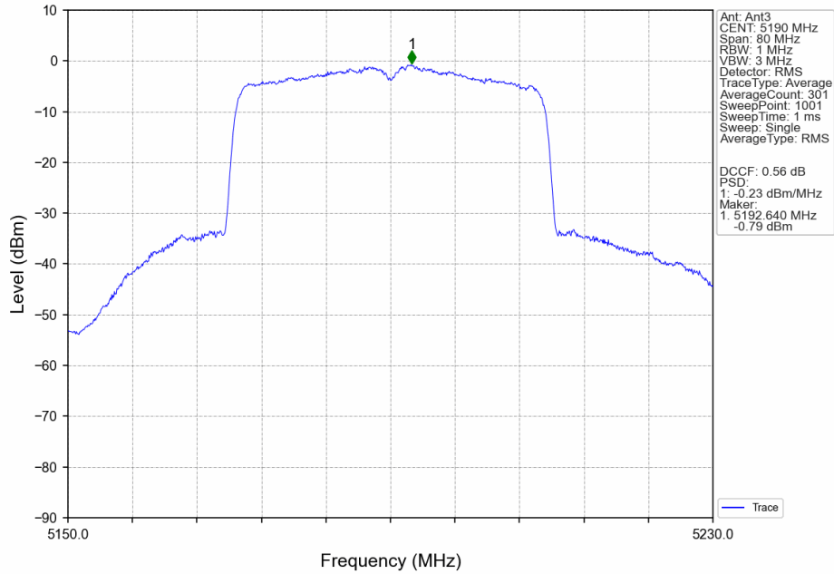
802.11ax(HEW40)_LCH_5190MHz_SU_ / _MIMO_NTNV
