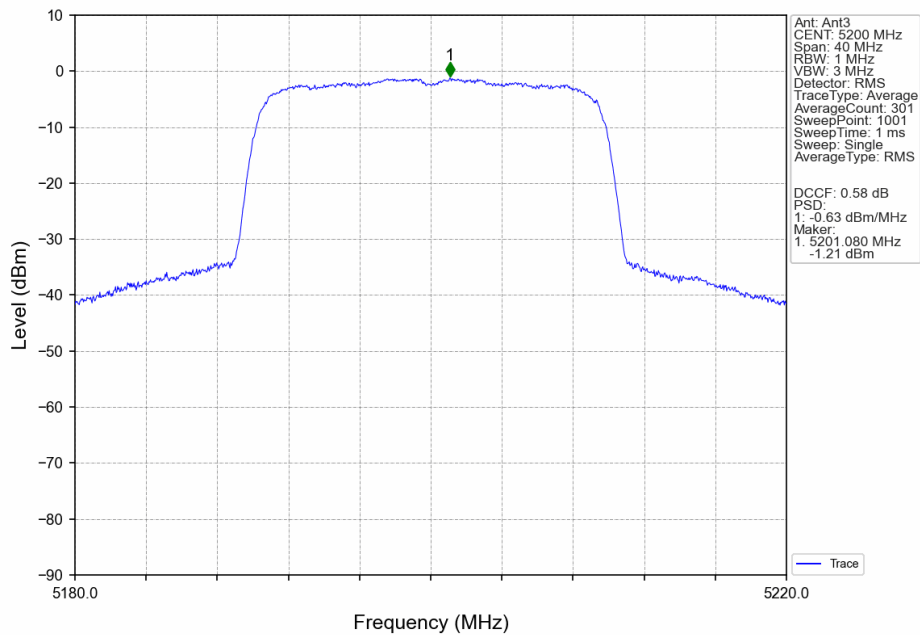
802.11ax(HEW20)_MCH_5200MHz_SU_ / _Ant3_NTNV
