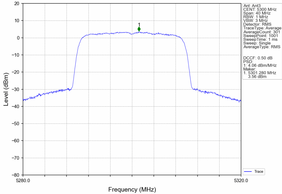
802.11ax(HEW20)_MCH_5300MHz_SU_ / _MIMO_NTNV
