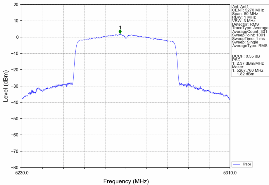
802.11ax(HEW40)_LCH_5270MHz_SU_/_Ant1_NTNV
