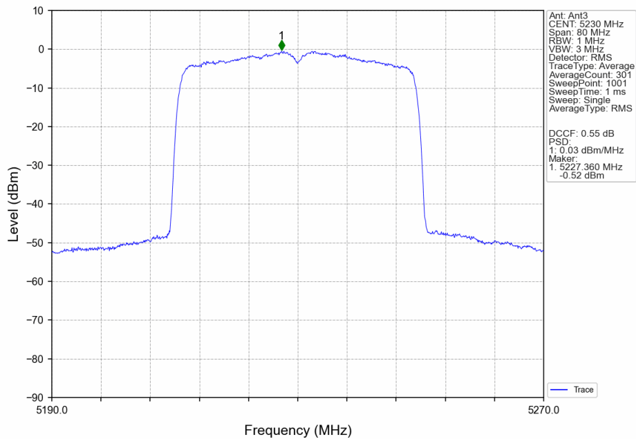
802.11ax(HEW40)_HCH_5230MHz_SU_ / _Ant3_NTNV
