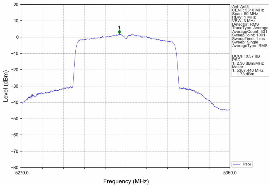
802.11ax(HEW40)_HCH_5310MHz_SU_ / _Ant3_NTNV
