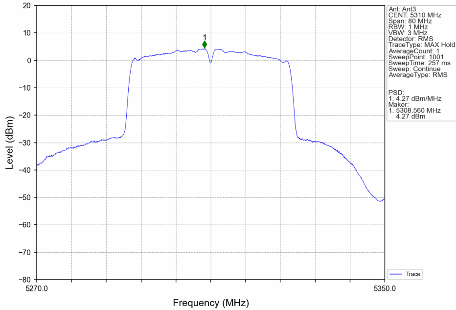
802.11ac(VHT40)_HCH_5310MHz_MIMO_NTNV
