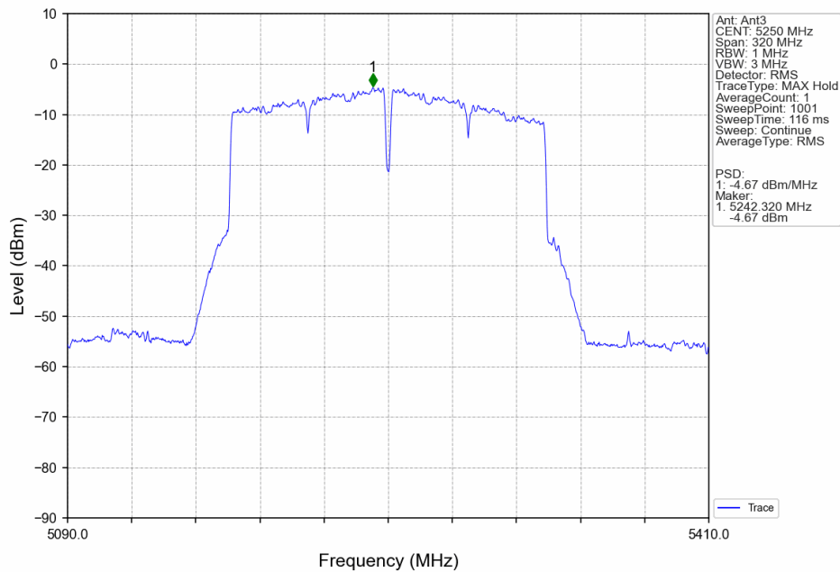
802.11ac(VHT160)_MCH_5250MHz_Ant3_NTNV
