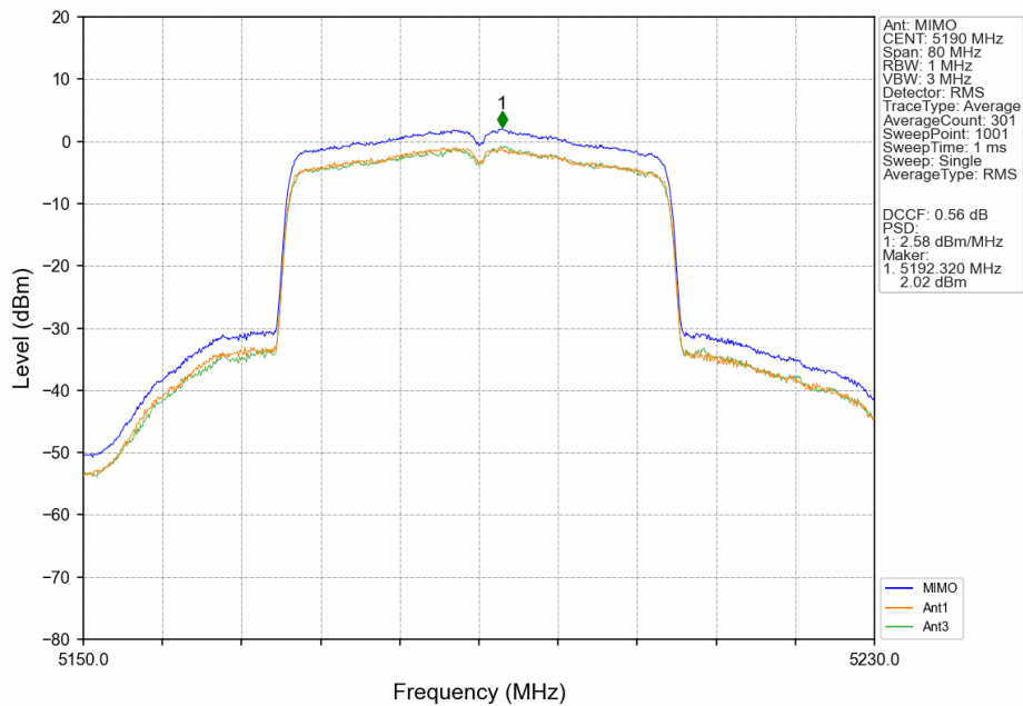
802.11ax(HEW40)_LCH_5190MHz_SU_ / _MIMO_NTNV
