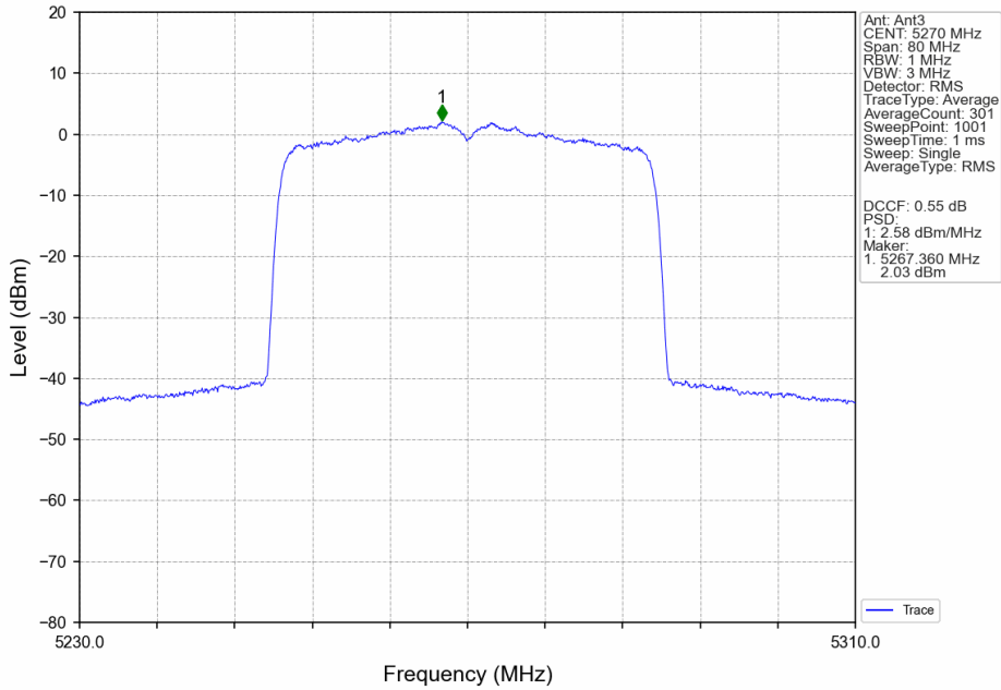
802.11ax(HEW40)_LCH_5270MHz_SU_ / _MIMO_NTNV
