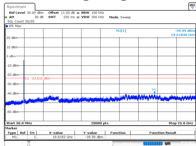
802.11n40_2437MHz_Chain 1
