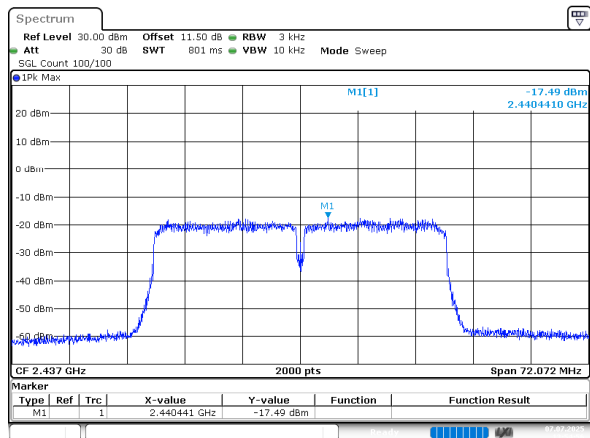
802.11n40_2437MHz_Chain 1
