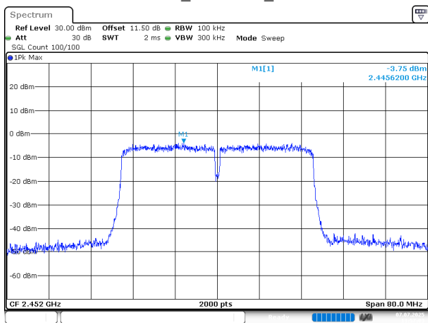
802.11n40_2452MHz_Chain 1
