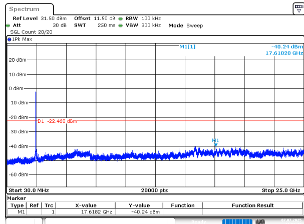
802.11n40_2452MHz_Chain 0
