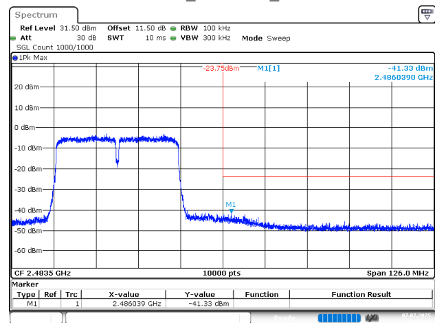
802.11n40_2452MHz_Chain 1
