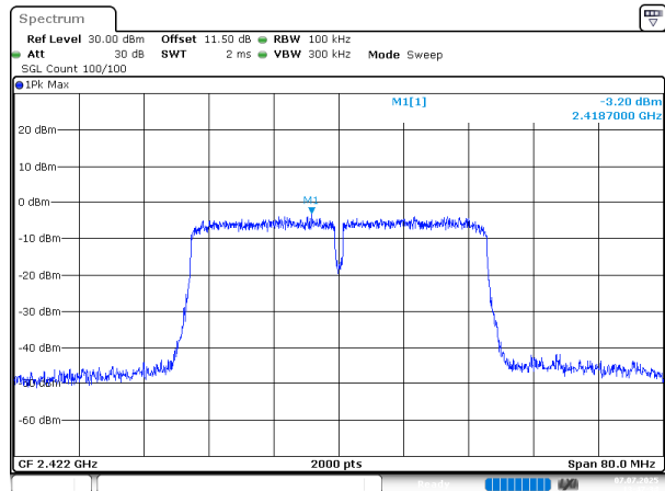
802.11n40_2422MHz_Chain 1
