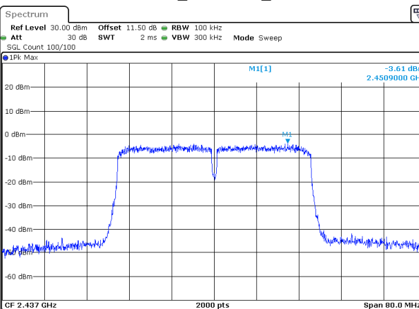
802.11n40_2437MHz_Chain 1
