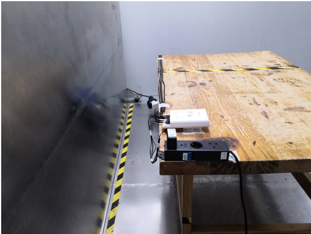
Conducted Emissions Side View-Adapter Power Mode
