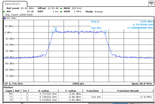
n20_5745MHz_Chain 0
