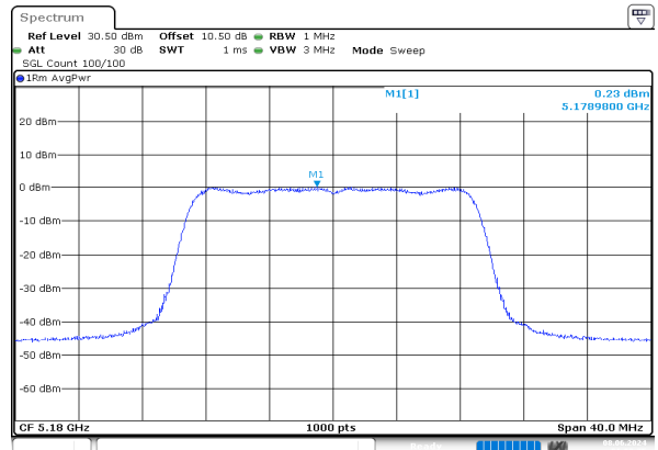
n20_5180MHz_Chain 1
