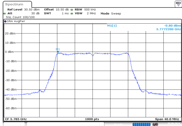
a_5785MHz_Chain 1
