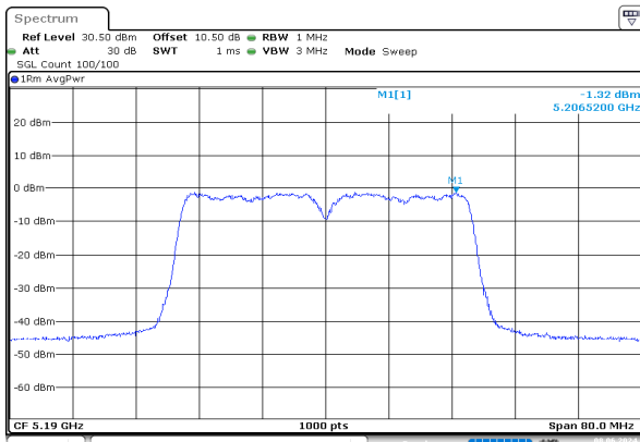
ac40_5190MHz_Chain 0
