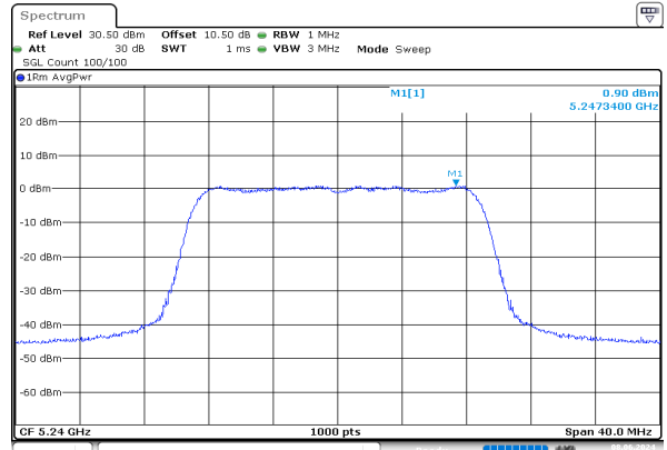
ac20_5240MHz_Chain 1
