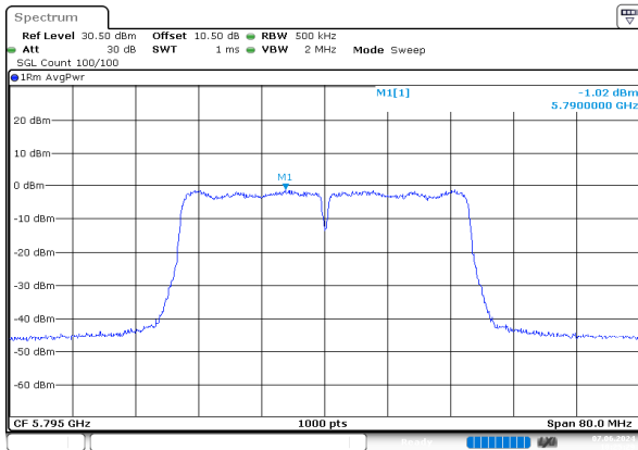
n40_5795MHz_Chain 0
