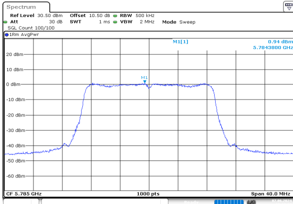
n20_5785MHz_Chain 0
