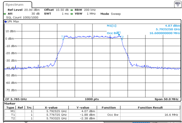
a_5785MHz_Chain 0
