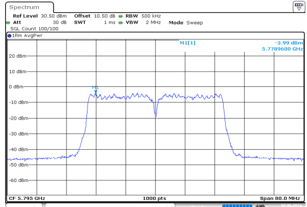
ac40_5795MHz_Chain 1
