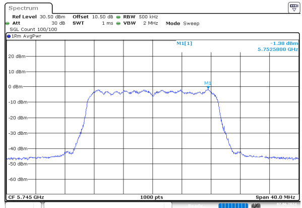
ac20_5745MHz_Chain 1
