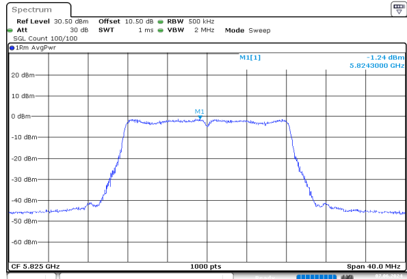
a_5825MHz_Chain 1
