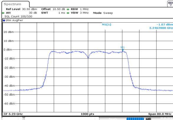
ac40_5230MHz_Chain 0
