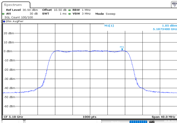
n20_5180MHz_Chain 0
