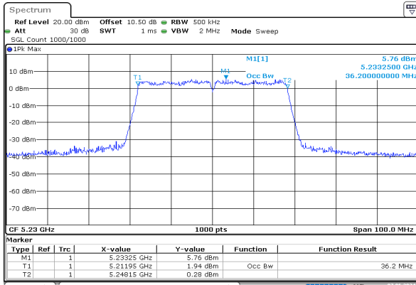
ac40_5230MHz_Chain 0
