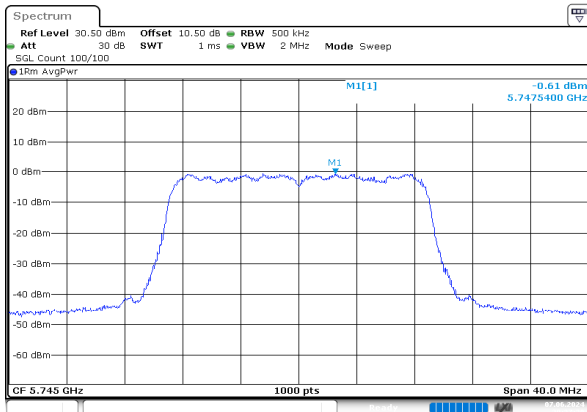
ac20_5745MHz_Chain 0
