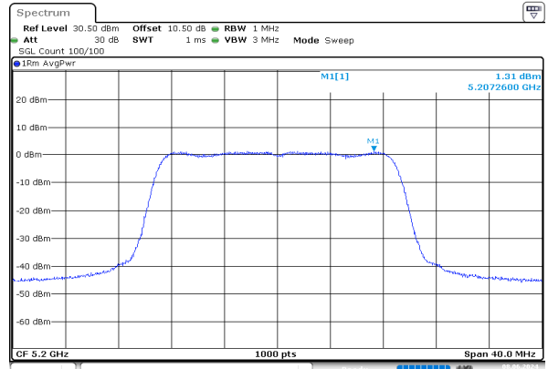
n20_5200MHz_Chain 1
