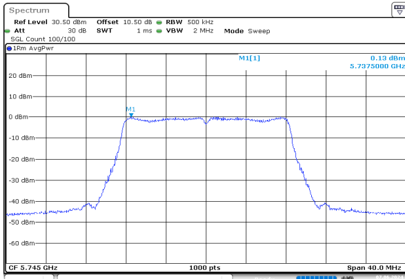
a_5745MHz_Chain 0
