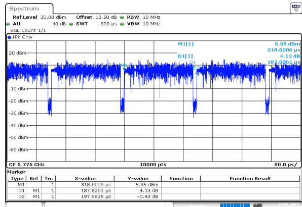
ac80_5775MHz_Chain 0
