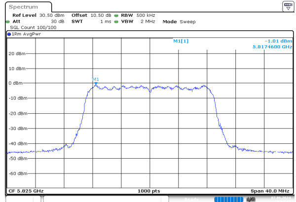
ac20_5825MHz_Chain 1
