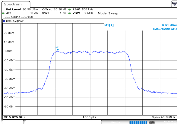
ac20_5825MHz_Chain 0
