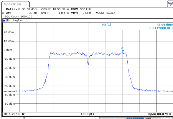
ac40_5795MHz_Chain 0
