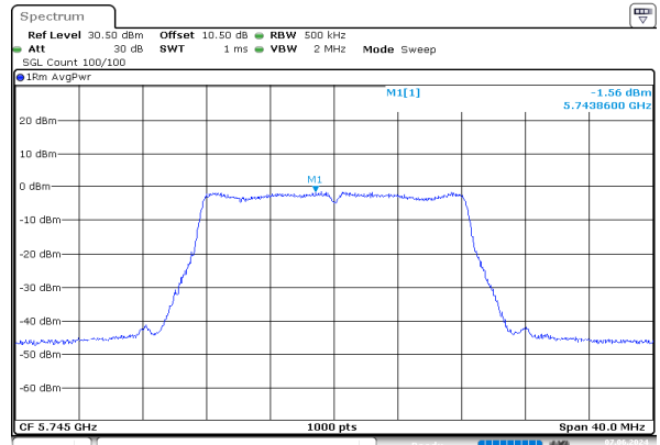
a_5745MHz_Chain 1
