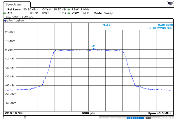
a_5180MHz_Chain 1
