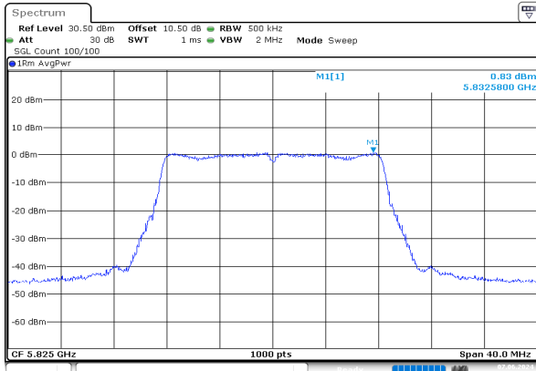
a_5825MHz_Chain 0
