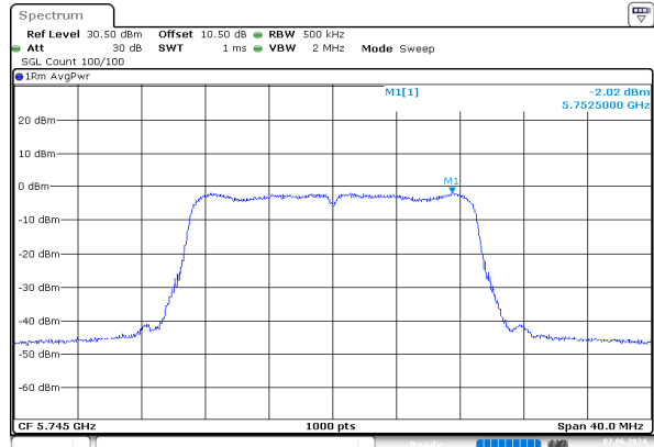
n20_5745MHz_Chain 1
