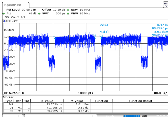
ac40_5755MHz_Chain 0
