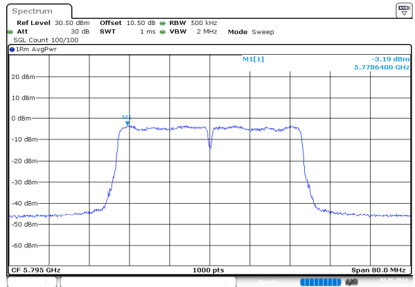
n40_5795MHz_Chain 1
