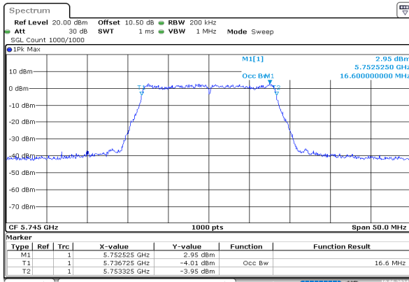
a_5745MHz_Chain 0
