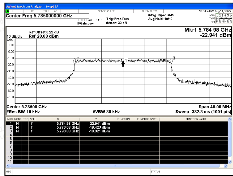
Freq. Stability NVNT be20 5785MHz Ant1
