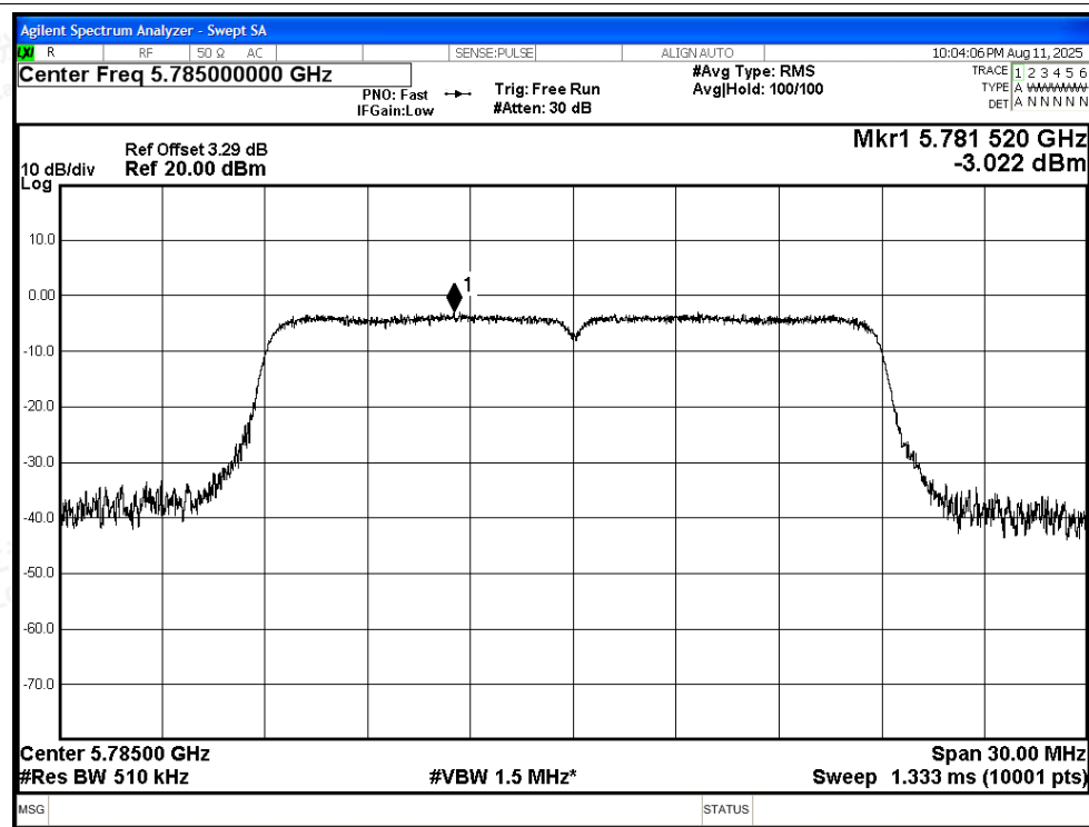
PSD NVNT be20 5785MHz Ant1
