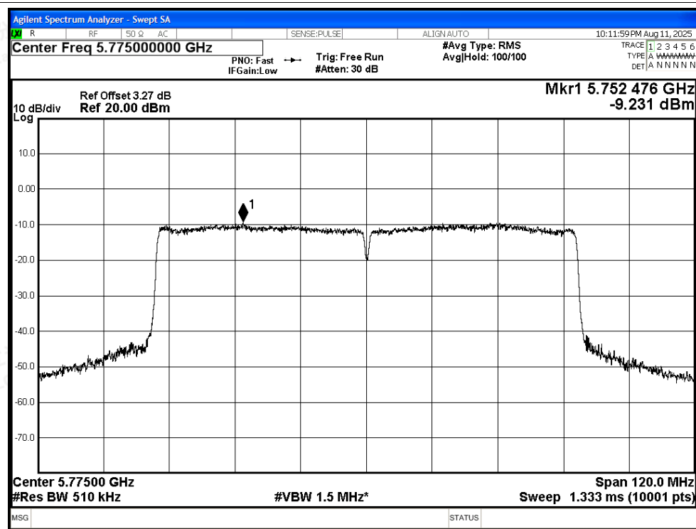
PSD NVNT be80 5775MHz Ant1
