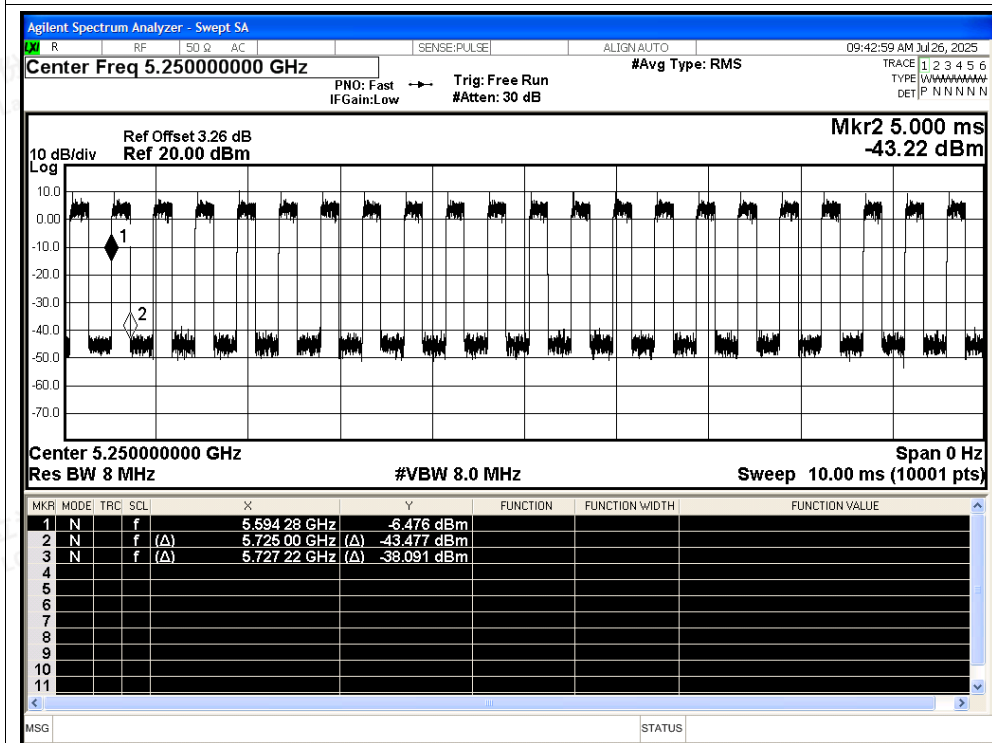
Duty Cycle NVNT be160 5250MHz Ant3
