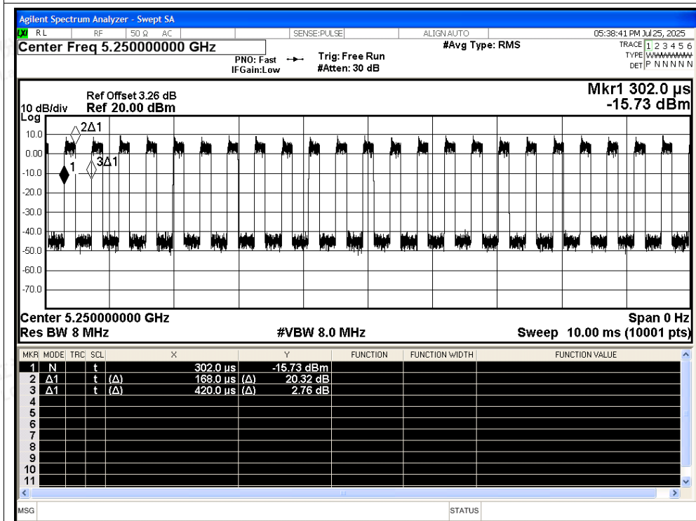
Duty Cycle NVNT be160 5250MHz Ant2
