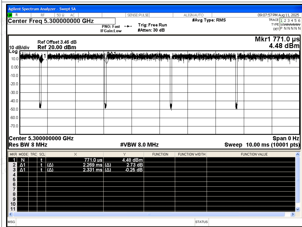
Duty Cycle NVNT be20 5300MHz Ant1
