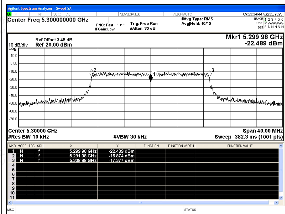
Freq. Stability NVNT be20 5300MHz Ant2
