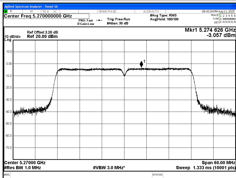
PSD NVNT be40 5270MHz Ant3
