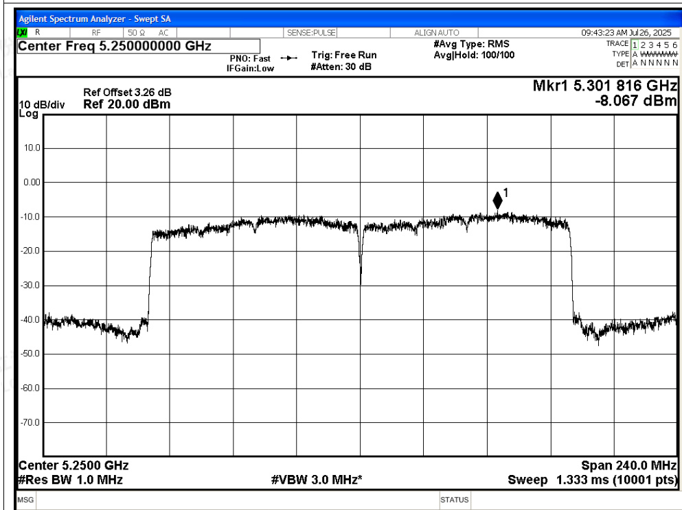
PSD NVNT be160 5250MHz Ant3
