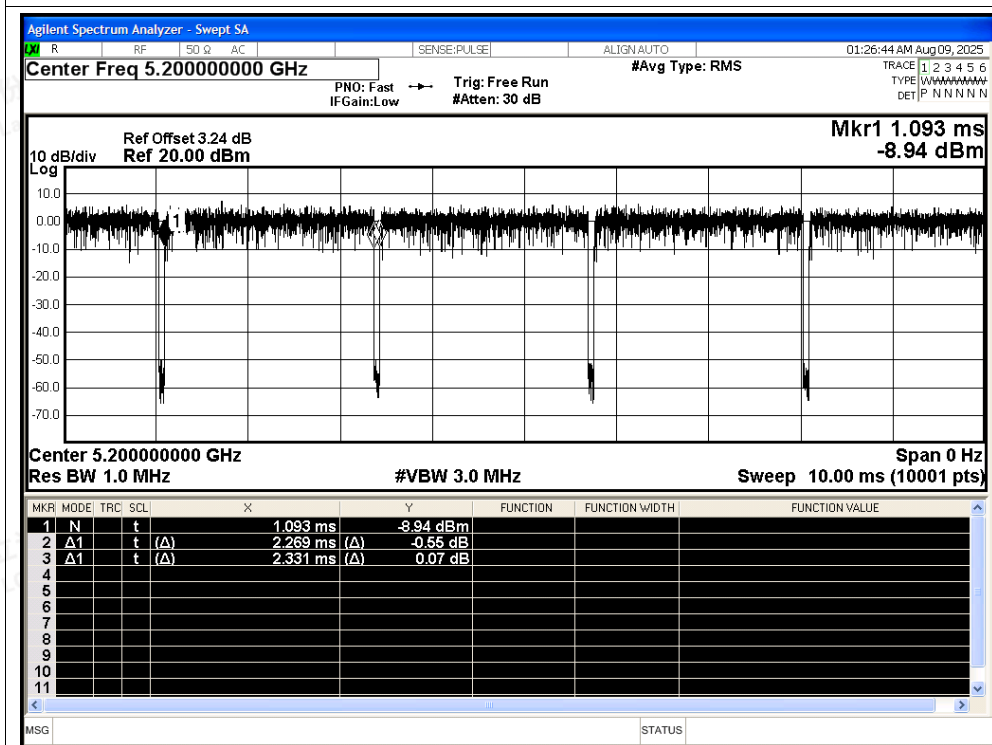
Duty Cycle NVNT be20 5200MHz Ant2
