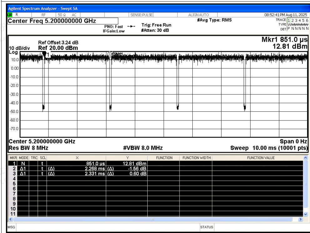
Duty Cycle NVNT be20 5200MHz Ant3
