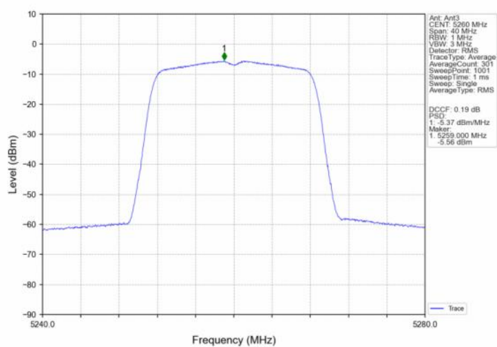
802.11a LCH_5260MHz_Ant3_NTNV
