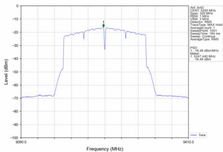
802.11ac(VHT160) MCH 5250MHz MIMO_NTNV
