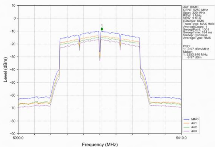
802.11ac(VHT160) MCH 5250MHz MIMO_NTNV
