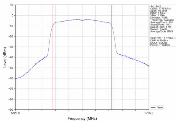
802.11n(HT20)_LCH_5745MHz_Ant1_NTN
