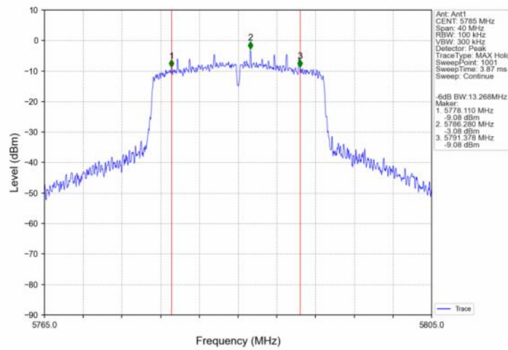
802.11ac(VHT20)_MCH_5785MHz_Ant1_NTNV
