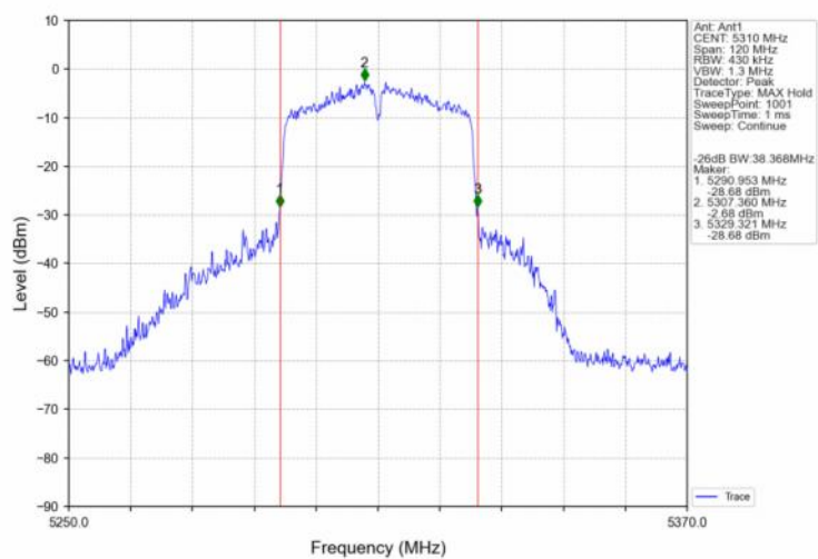
802.11ac(VHT40)_HCH_5310MHz_Ant1_NTN
