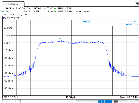
802.11ax20_5180MHz_RU_Full_Chain 0
