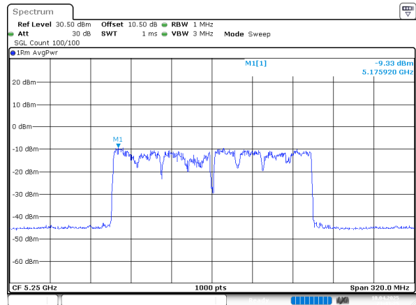
802.11ac160_5250MHz_Chain 1
