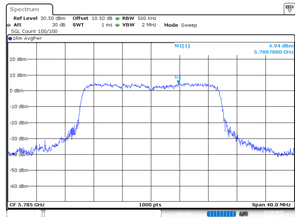
802.11ax20_5785MHz_RU_Full_Chain 0
