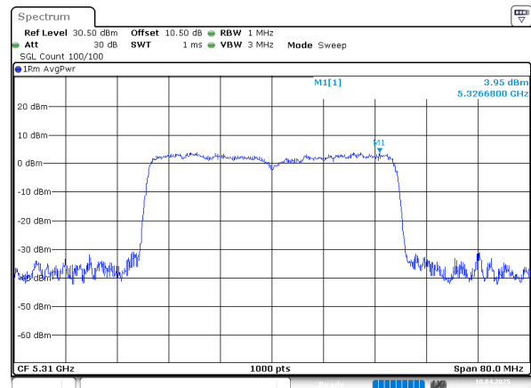
802.11ax40_5310MHz_RU_Full_Chain 2
