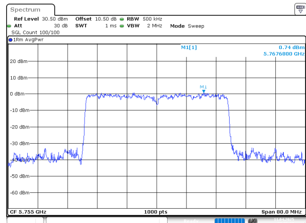
802.11ax40_5755MHz_RU_Full_Chain 2
