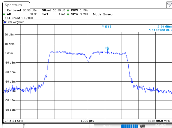
802.11ac40_5310MHz_Chain 1
