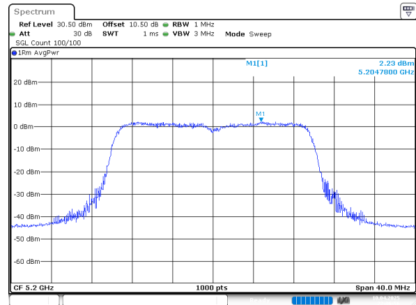
802.11ax20_5200MHz_RU_Full_Chain 0
