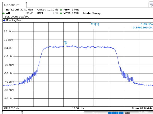
802.11ax20_5200MHz_RU_Full_Chain 1
