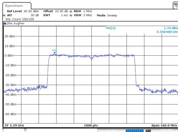
802.11ax80_5290MHz_RU_Full_Chain 0
