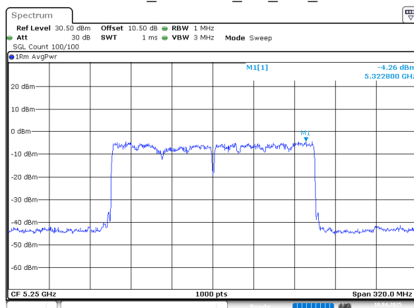
802.11ax160_5250MHz_RU_Full_Chain 1
