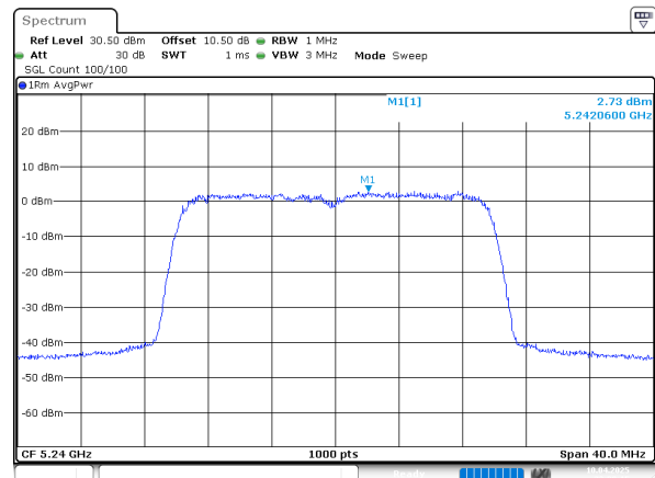
802.11ax20_5240MHz_RU_Full_Chain 1
