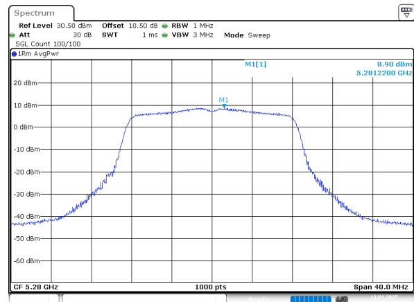
802.11a_5280MHz_Chain 2
