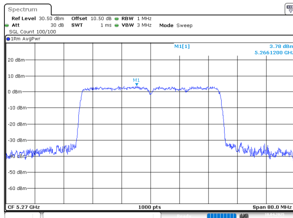
802.11ax40_5270MHz_RU_Full_Chain 2
