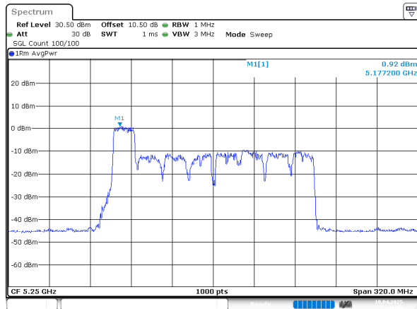
802.11ac160_5250MHz_Chain 0
