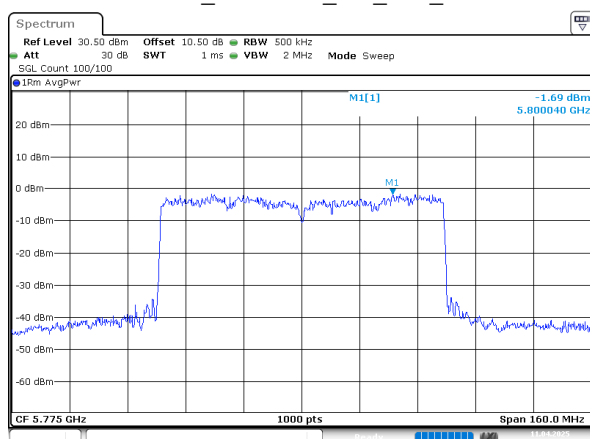
802.11ax80_5775MHz_RU_Full_Chain 1
