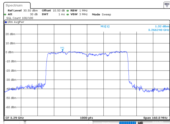
802.11ax80_5290MHz_RU_Full_Chain 1
