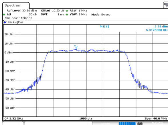
802.11ax20_5320MHz_RU_Full_Chain 1
