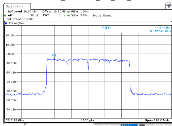
802.11ax160_5250MHz_RU_Full_Chain 2
