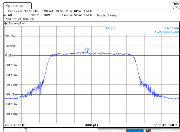
802.11ax20_5260MHz_RU_Full_Chain 0
