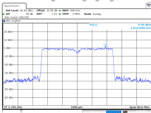
802.11ax40_5795MHz_RU_Full_Chain 2
