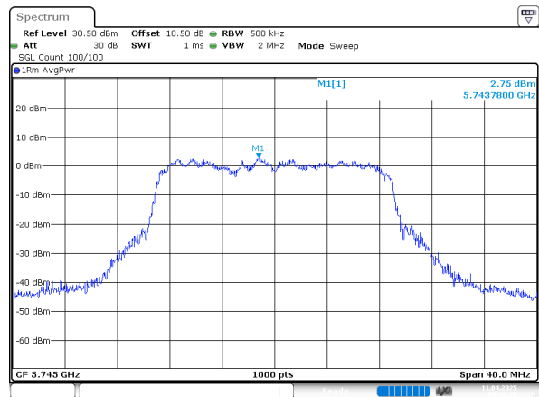
802.11ac20_5745MHz_Chain 1
