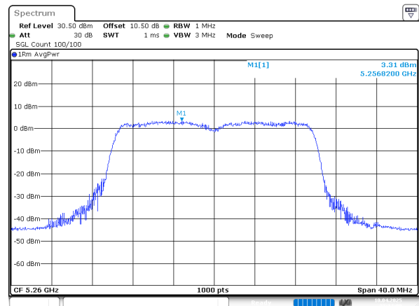
802.11ax20_5260MHz_RU_Full_Chain 2
