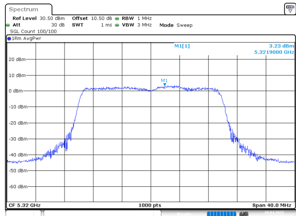
802.11ax20_5320MHz_RU_Full_Chain 0
