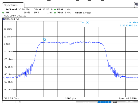
802.11ax20_5280MHz_RU_Full_Chain 2
