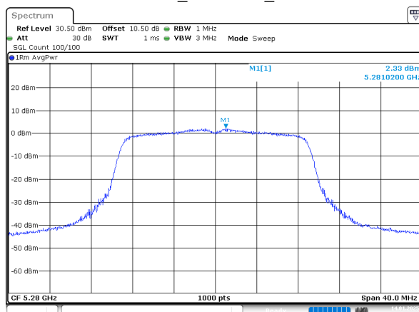
802.11n20_5280MHz_Chain 0
