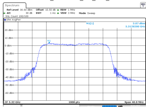
802.11ax20_5320MHz_RU_Full_Chain 2
