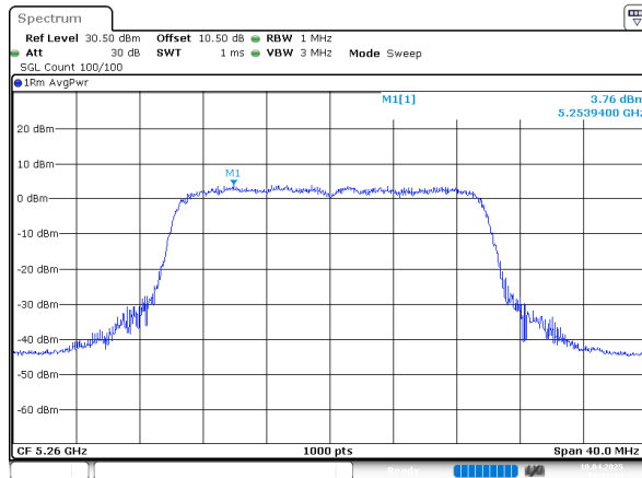
802.11ax20_5260MHz_RU_Full_Chain 1
