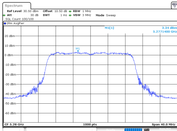
802.11ax20_5280MHz_RU_Full_Chain 0
