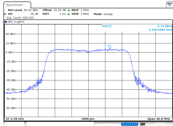
802.11ax20_5280MHz_RU_Full_Chain 1
