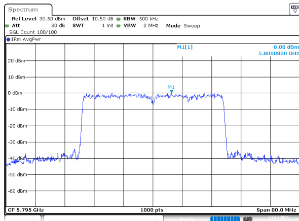
802.11ax40_5795MHz_RU_Full_Chain 1
