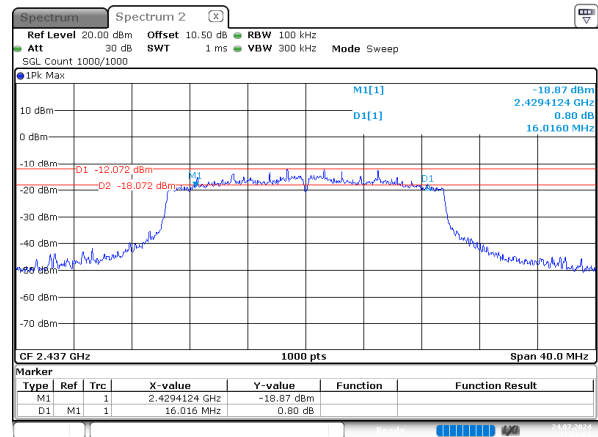
ax20_2437MHz_RU_Full_Chain 0
