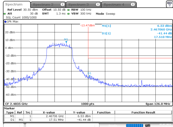
ax20_2462MHz_RU_Full_Chain 0
