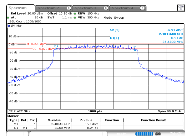
ax40_2422MHz_RU_Full_Chain 0
