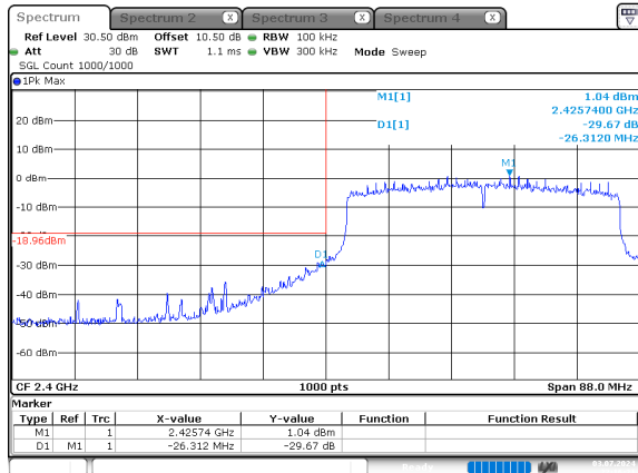
ax40_2422MHz_RU_Full_Chain 0
