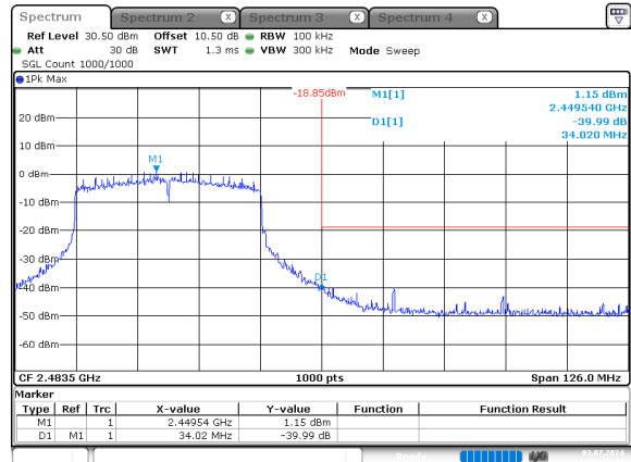
ax40_2452MHz_RU_Full_Chain 0
