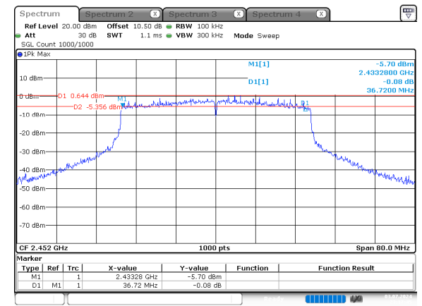
ax40_2452MHz_RU_Full_Chain 0
