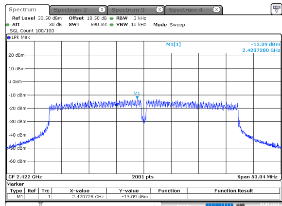
n40_2422MHz_Chain 0
