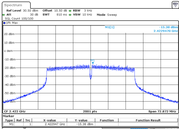
802.11n40_2422MHz
