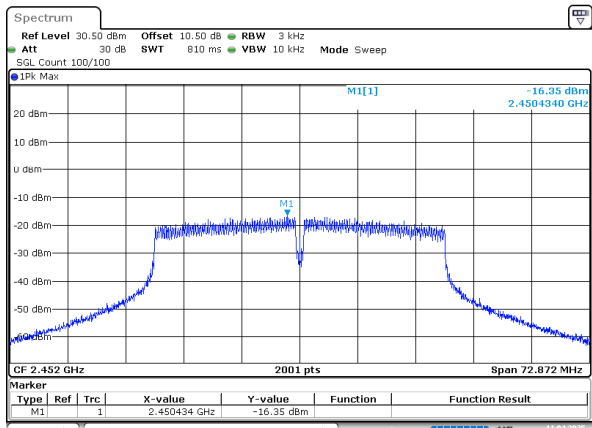
802.11n40_2452MHz
