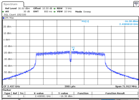
802.11n40_2437MHz
