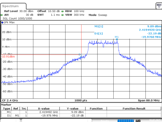
802.11g_2412MHz_Chain 0
