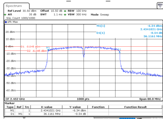
802.11n40_2452MHz_Chain 0
