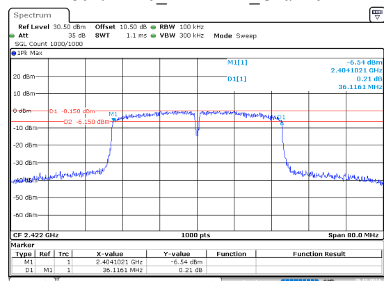
802.11n40_2422MHz_Chain 0
