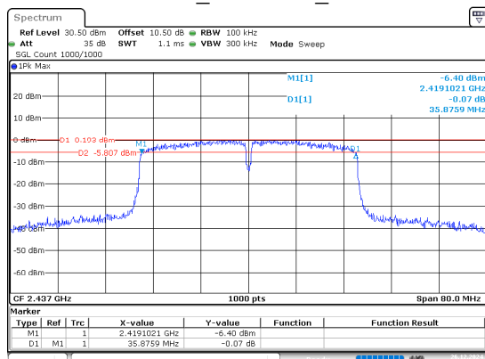
802.11n40_2437MHz_Chain 0
