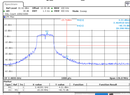
802.11g_2462MHz_Chain 1
