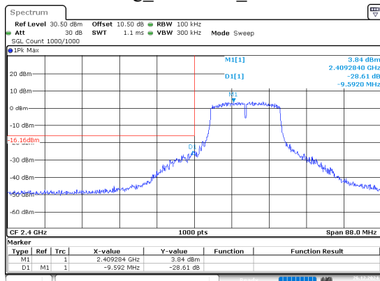
802.11g_2412MHz_Chain 0
