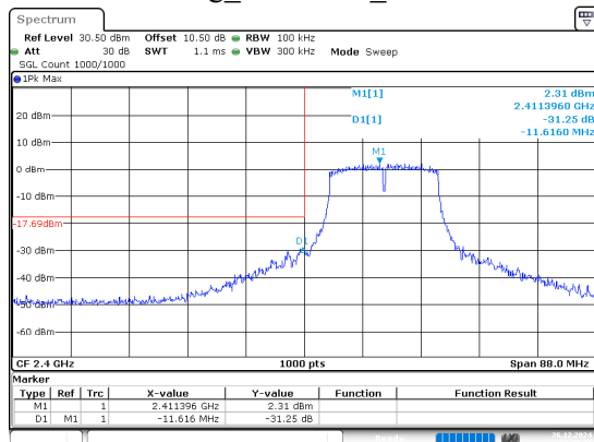
802.11g_2412MHz_Chain 1
