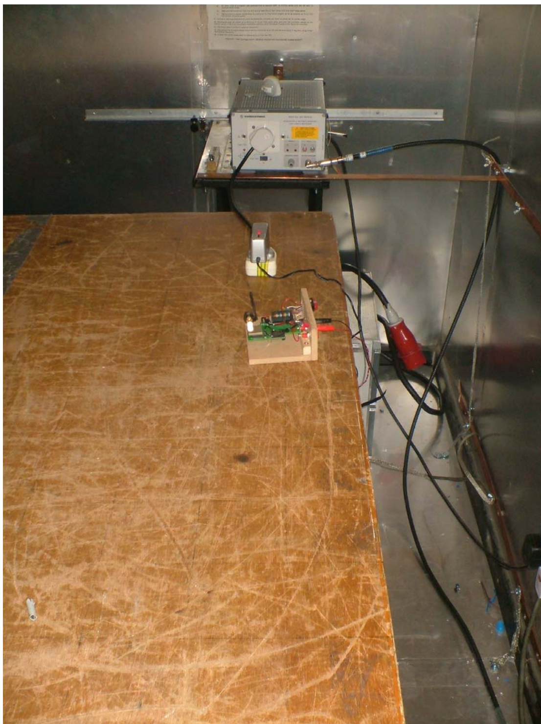
AC Powerline Conducted Emissions
