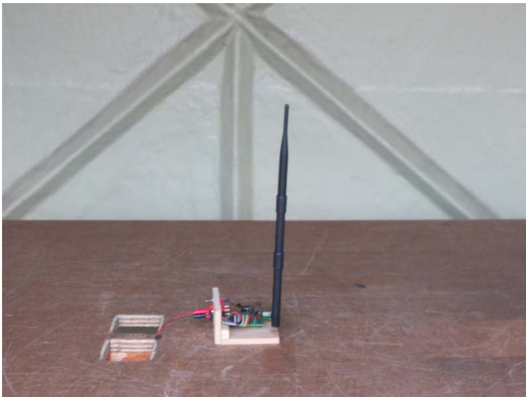
Close Up Of EUT on OATS
