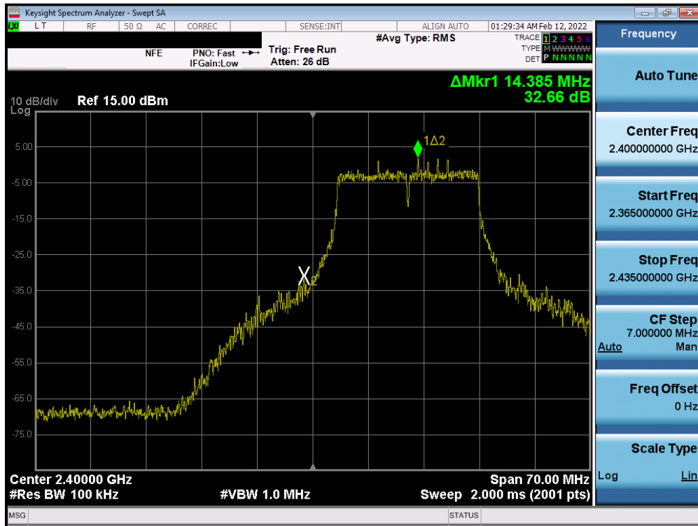
Plot 7-77. Band Edge Plot SISO ANT1 (802.11n (2.4GHz) – Ch. 1)
