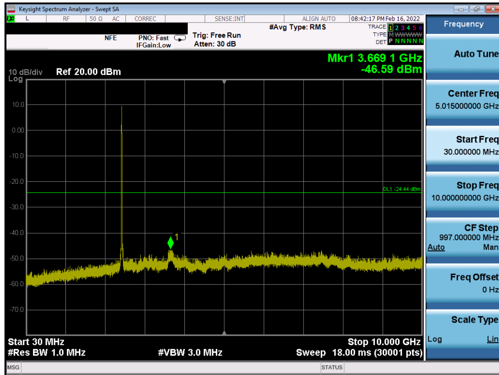
Plot 7-105. Conducted Spurious Plot SISO ANT2 (802.11b – Ch. 6)
