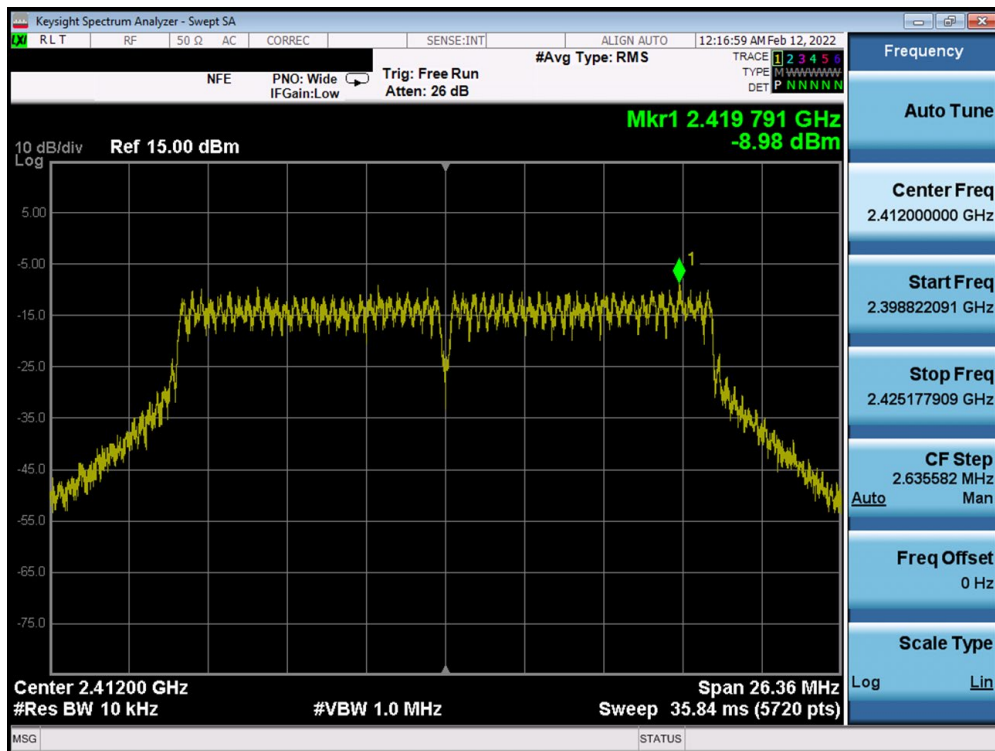
Plot 7-67. Power Spectral Density Plot MIMO ANT1 (802.11n (2.4GHz) – Ch. 1)
