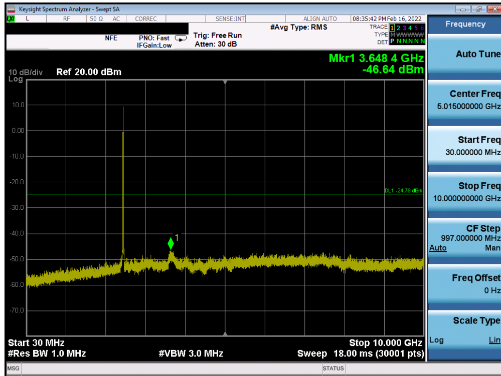
Plot 7-101. Conducted Spurious Plot SISO ANT1 (802.11b – Ch. 11)
