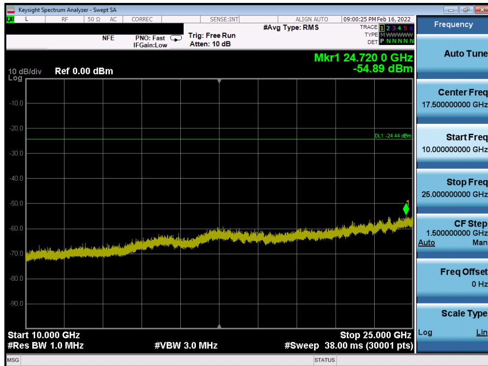
Plot 7-106. Conducted Spurious Plot SISO ANT2 (802.11b – Ch. 6)
