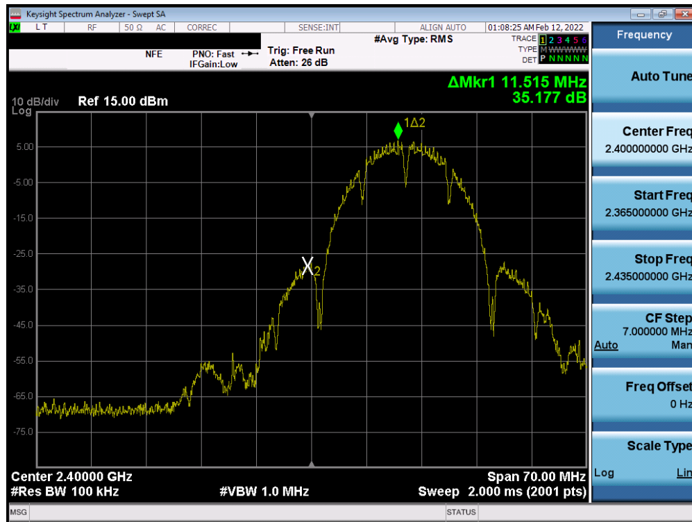
Plot 7-79. Band Edge Plot SISO ANT2 (802.11b – Ch. 1)
