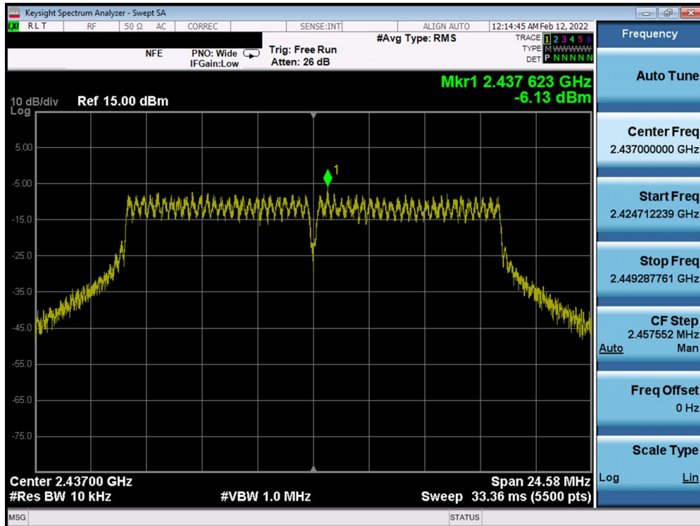
Plot 7-63. Power Spectral Density Plot MIMO ANT1 (802.11g – Ch. 6)
