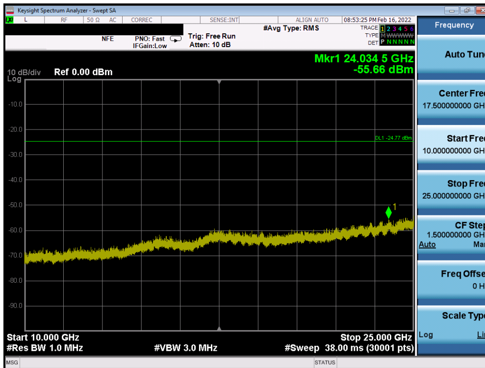
Plot 7-98. Conducted Spurious Plot SISO ANT1 (802.11b – Ch. 1)
