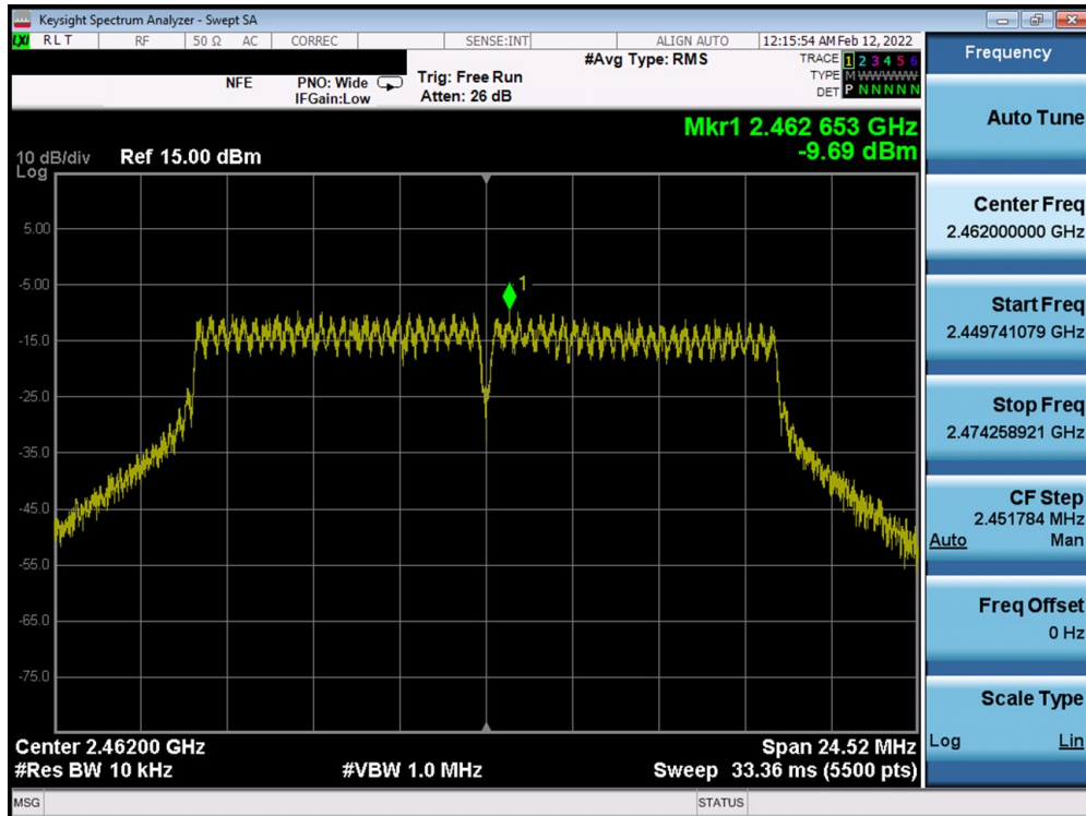
Plot 7-65. Power Spectral Density Plot MIMO ANT1 (802.11g – Ch. 11)
