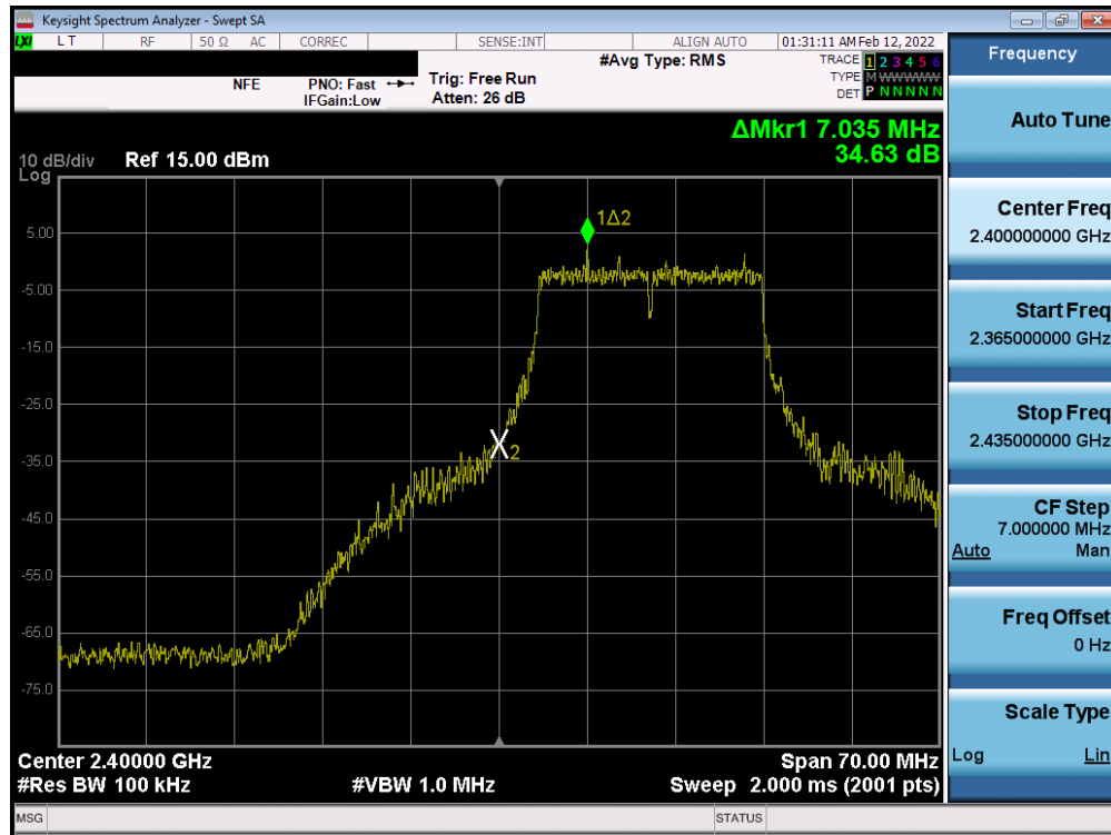
Plot 7-83. Band Edge Plot SISO ANT2 (802.11n (2.4GHz) – Ch. 1)
