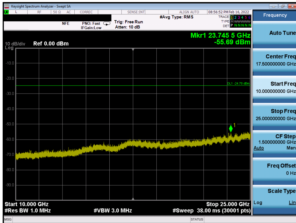
Plot 7-102. Conducted Spurious Plot SISO ANT1 (802.11b – Ch. 11)
