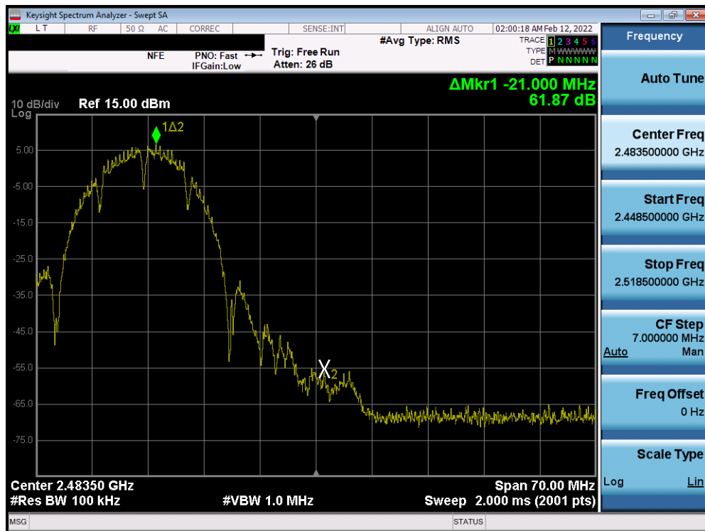
Plot 7-88. Band Edge Plot MIMO ANT2 (802.11b – Ch. 11)
