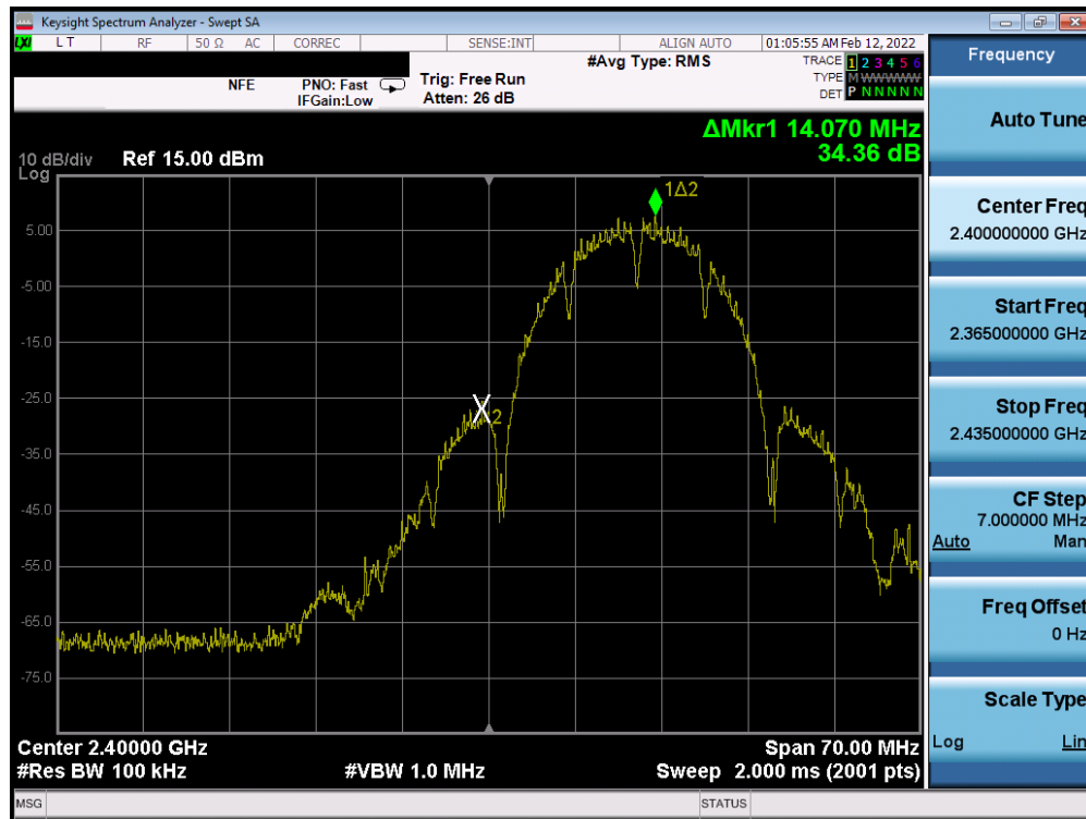
Plot 7-73. Band Edge Plot SISO ANT1 (802.11b – Ch. 1)
