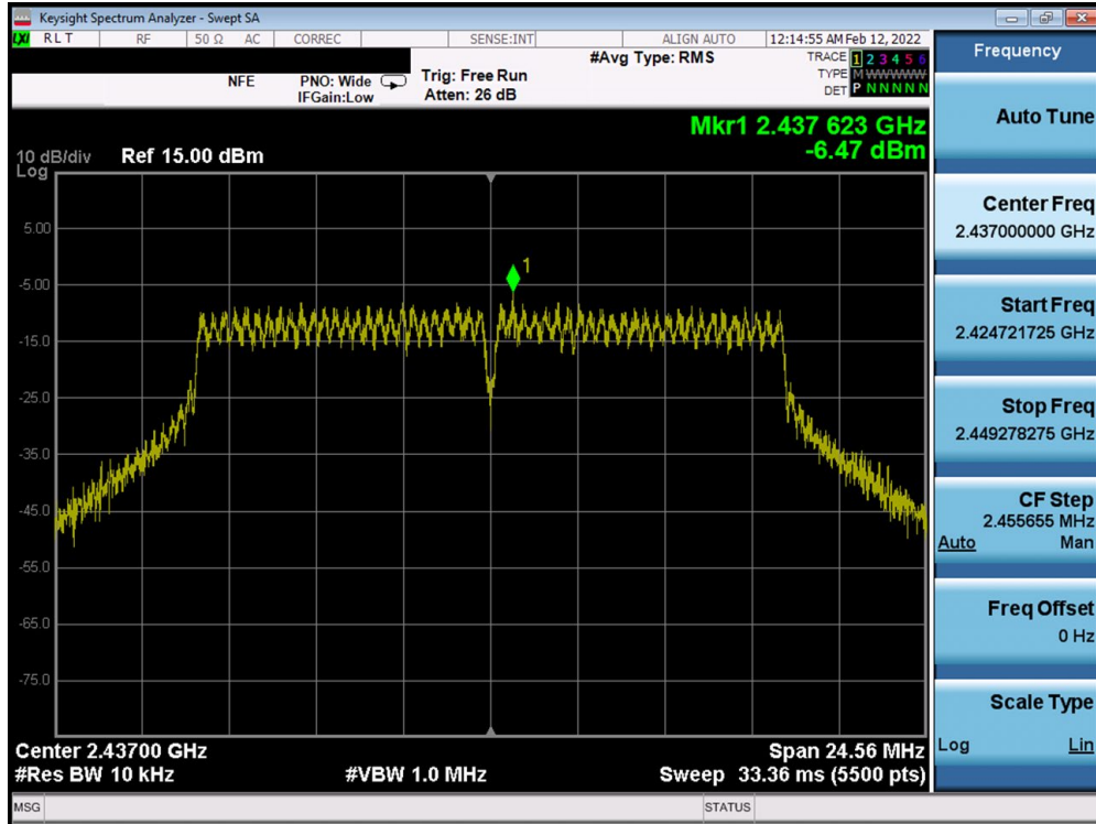
Plot 7-64. Power Spectral Density Plot MIMO ANT2 (802.11g – Ch. 6)
