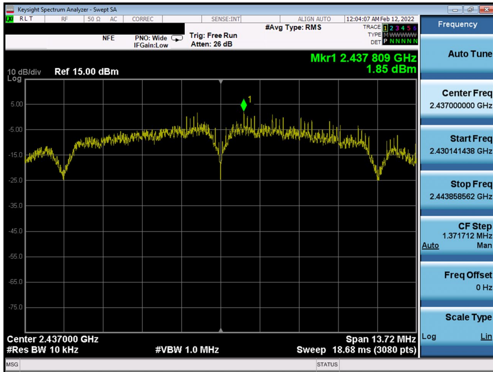
Plot 7-58. Power Spectral Density Plot MIMO ANT2 (802.11b – Ch. 6)
