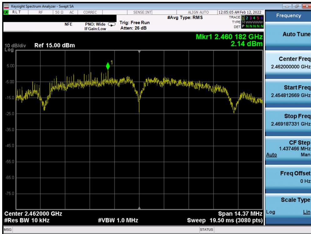
Plot 7-59. Power Spectral Density Plot MIMO ANT1 (802.11b – Ch. 11)
