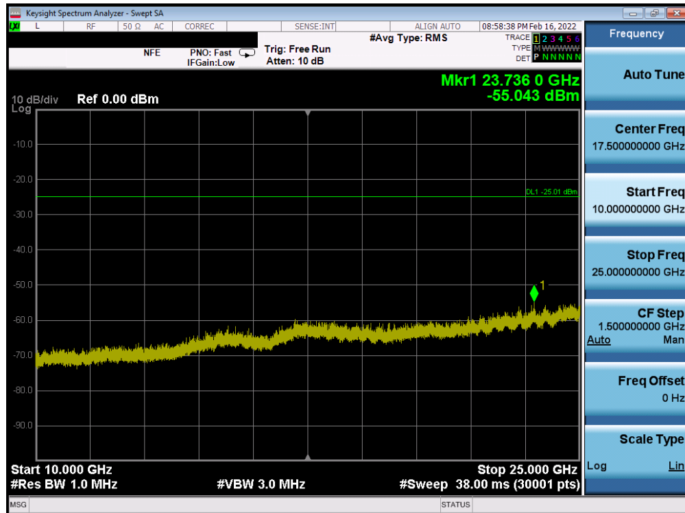
Plot 7-104. Conducted Spurious Plot SISO ANT2 (802.11b – Ch. 1)
