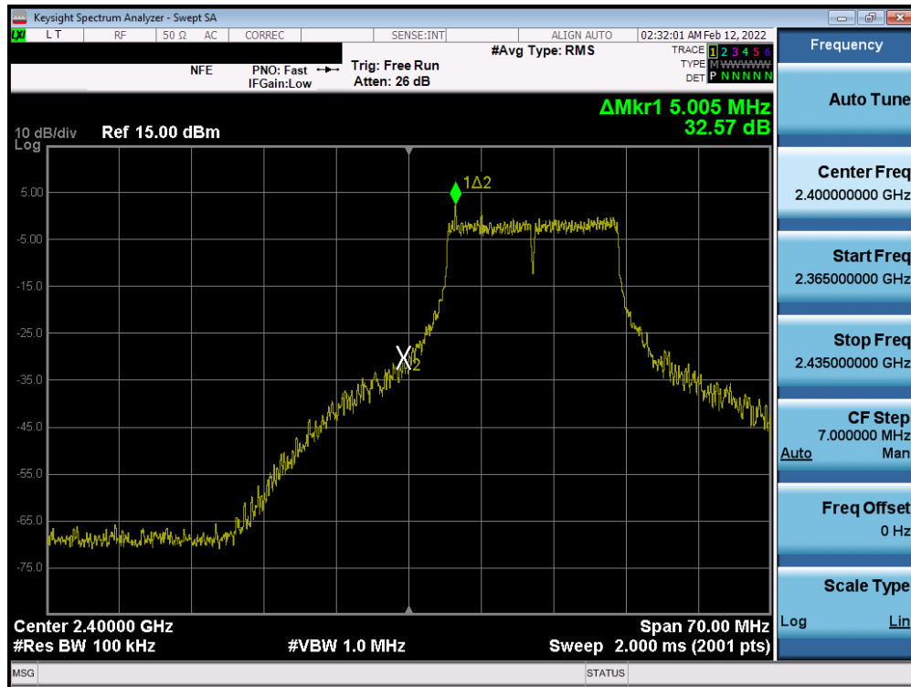
Plot 7-75. Band Edge Plot SISO ANT1 (802.11g- Ch. 1)
