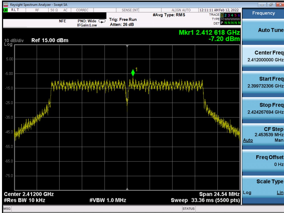
Plot 7-62. Power Spectral Density Plot MIMO ANT2 (802.11g – Ch. 1)
