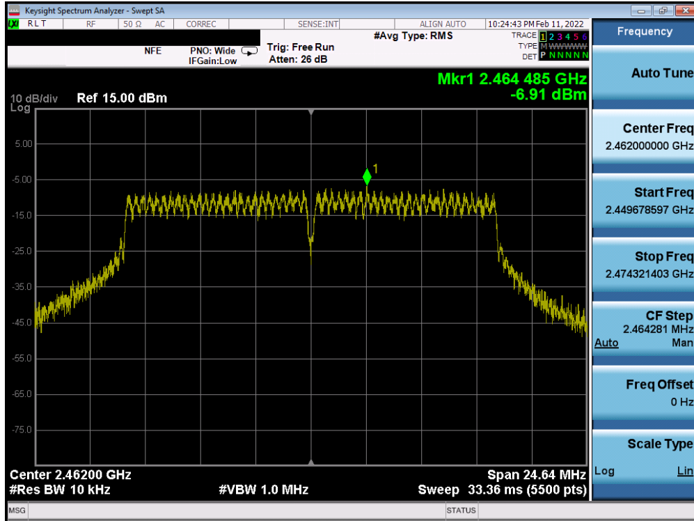
Plot 7-51. Power Spectral Density Plot SISO ANT2 (802.11g – Ch. 11)
