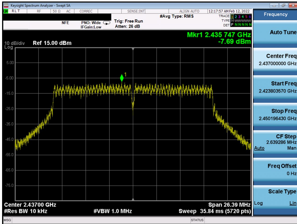
Plot 7-70. Power Spectral Density Plot MIMO ANT2 (802.11n (2.4GHz) – Ch. 6)
