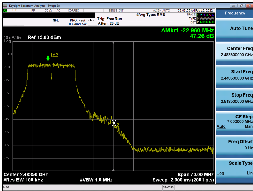
Plot 7-82. Band Edge Plot SISO ANT2 (802.11g – Ch. 11)
