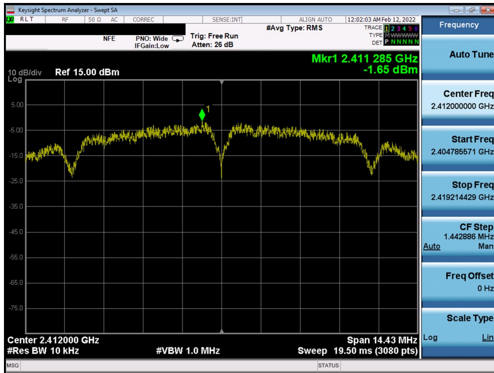
Plot 7-55. Power Spectral Density Plot MIMO ANT1 (802.11b – Ch. 1)
