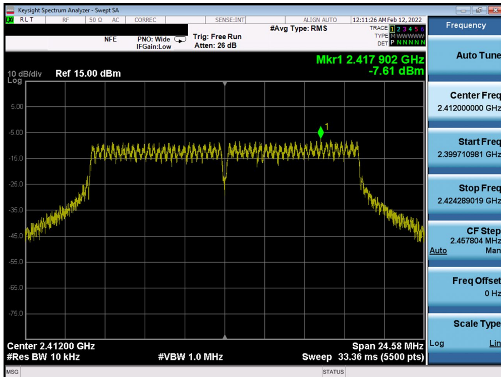
Plot 7-61. Power Spectral Density Plot MIMO ANT1 (802.11g – Ch. 1)
