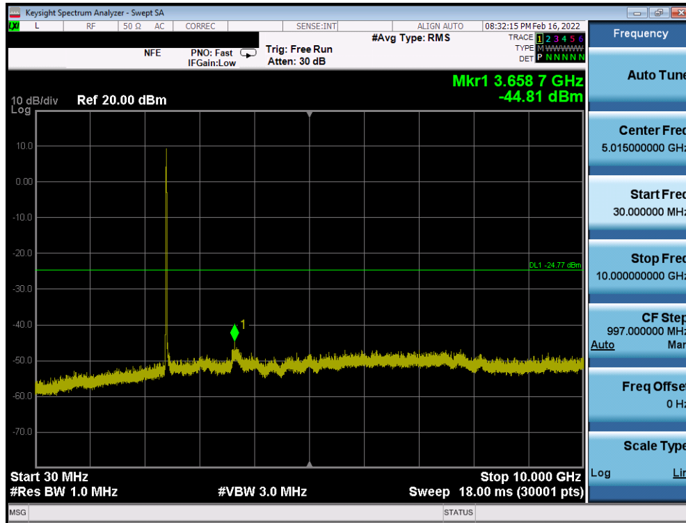
Plot 7-97. Conducted Spurious Plot SISO ANT1 (802.11b – Ch. 1)
