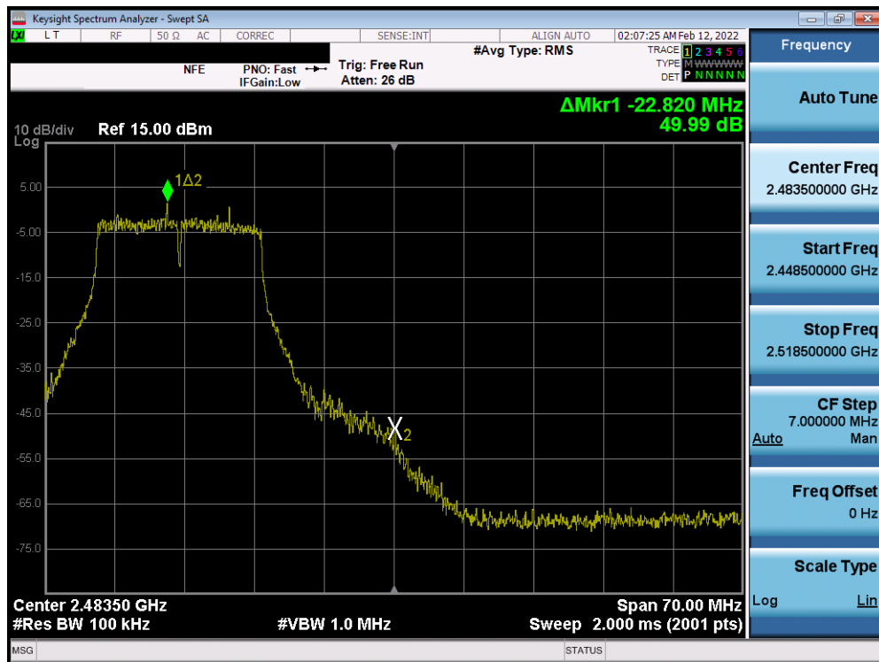
Plot 7-91. Band Edge Plot MIMO ANT1 (802.11g – Ch. 11)
