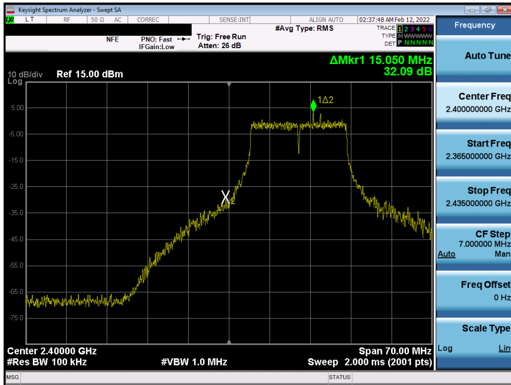
Plot 7-81. Band Edge Plot SISO ANT2 (802.11g– Ch. 1)
