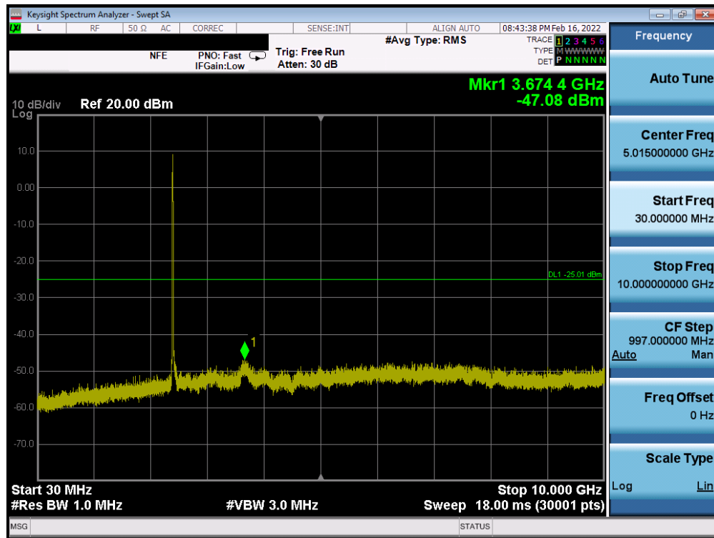
Plot 7-103. Conducted Spurious Plot SISO ANT2 (802.11b – Ch. 1)
