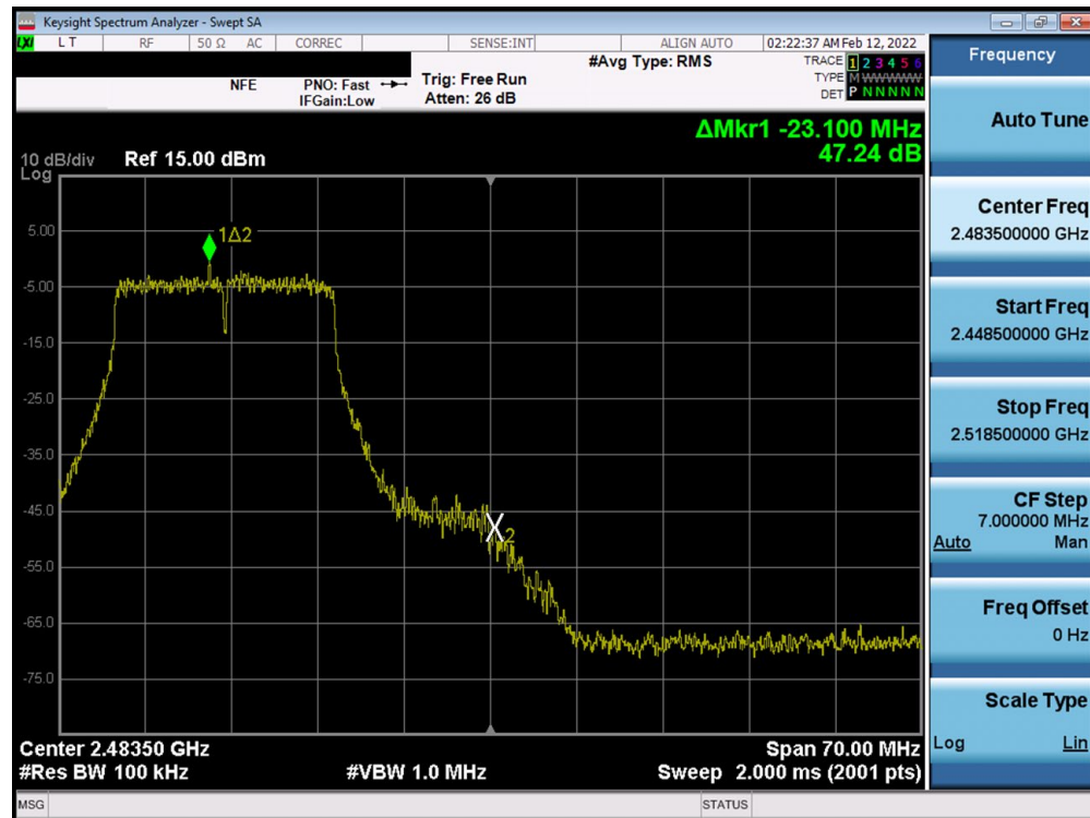
Plot 7-84. Band Edge Plot SISO ANT2 (802.11n (2.4GHz) – Ch. 11)
