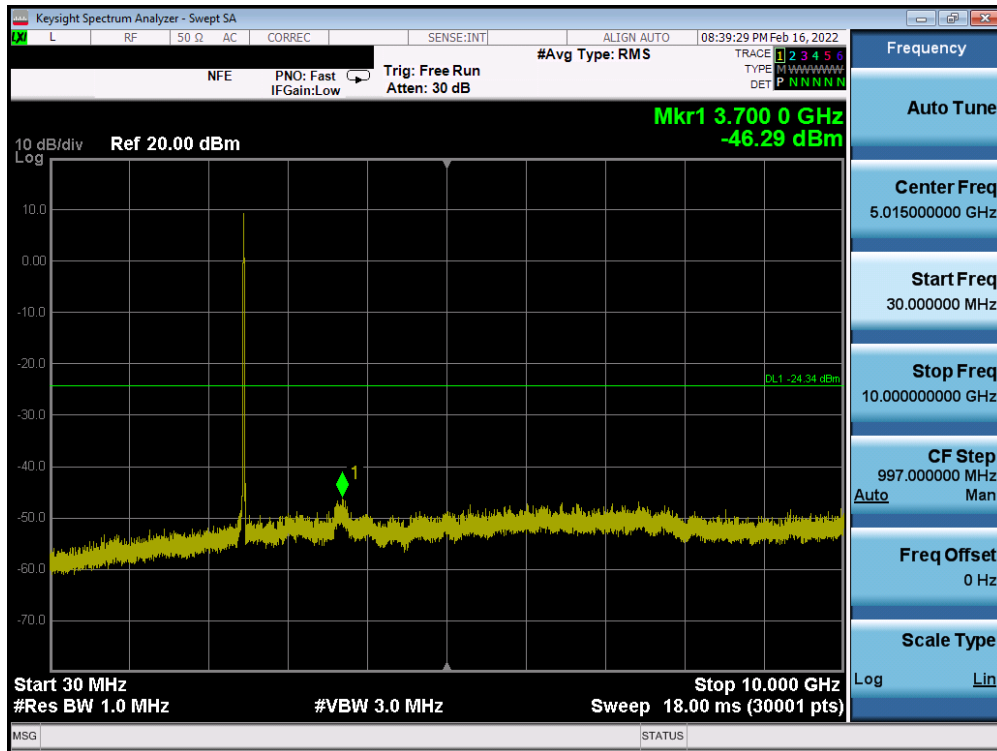
Plot 7-107. Conducted Spurious Plot SISO ANT2 (802.11b – Ch. 11)
