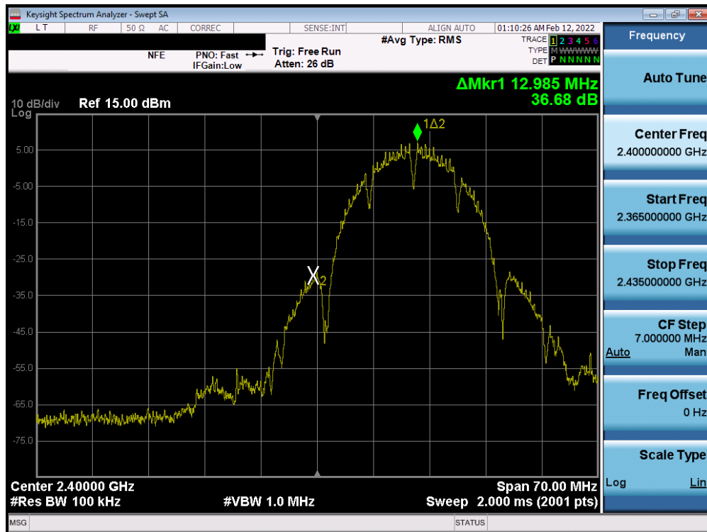
Plot 7-86. Band Edge Plot MIMO ANT2 (802.11b – Ch. 1)
