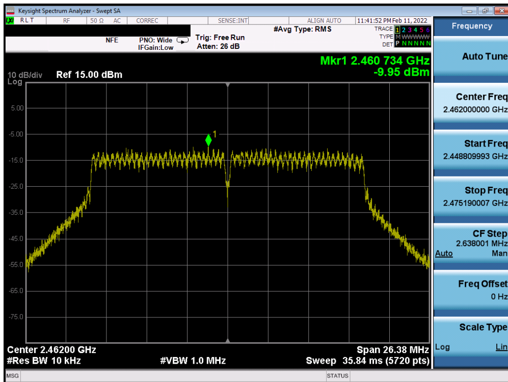
Plot 7-54. Power Spectral Density Plot SISO ANT2 (802.11n (2.4GHz) – Ch. 11)
