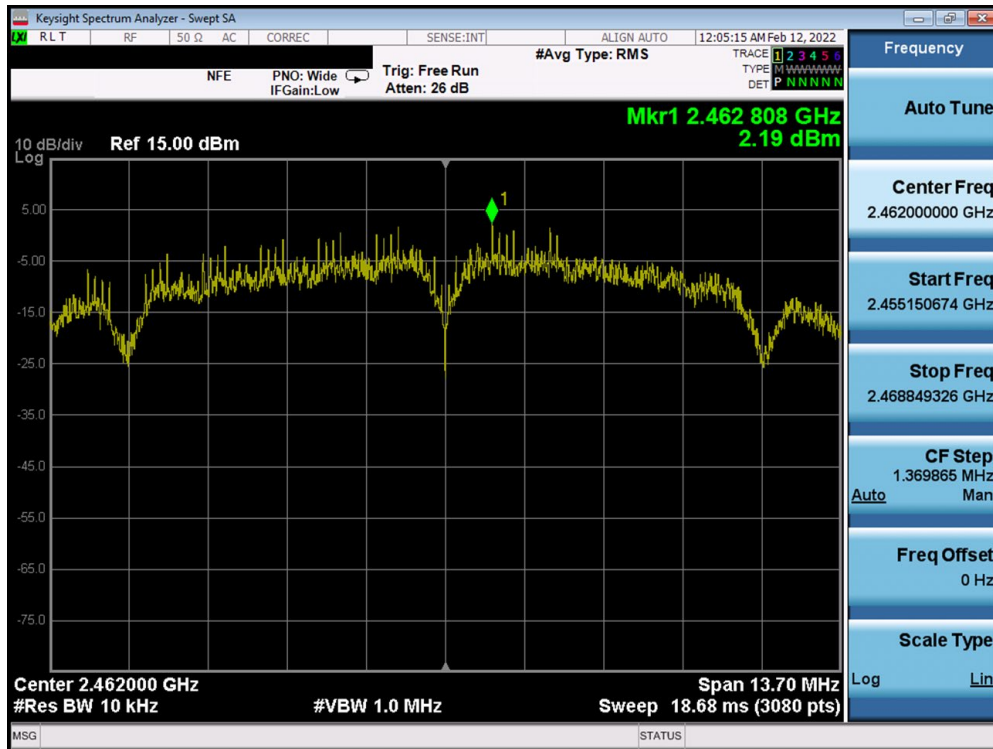
Plot 7-60. Power Spectral Density Plot MIMO ANT2 (802.11b – Ch. 11)
