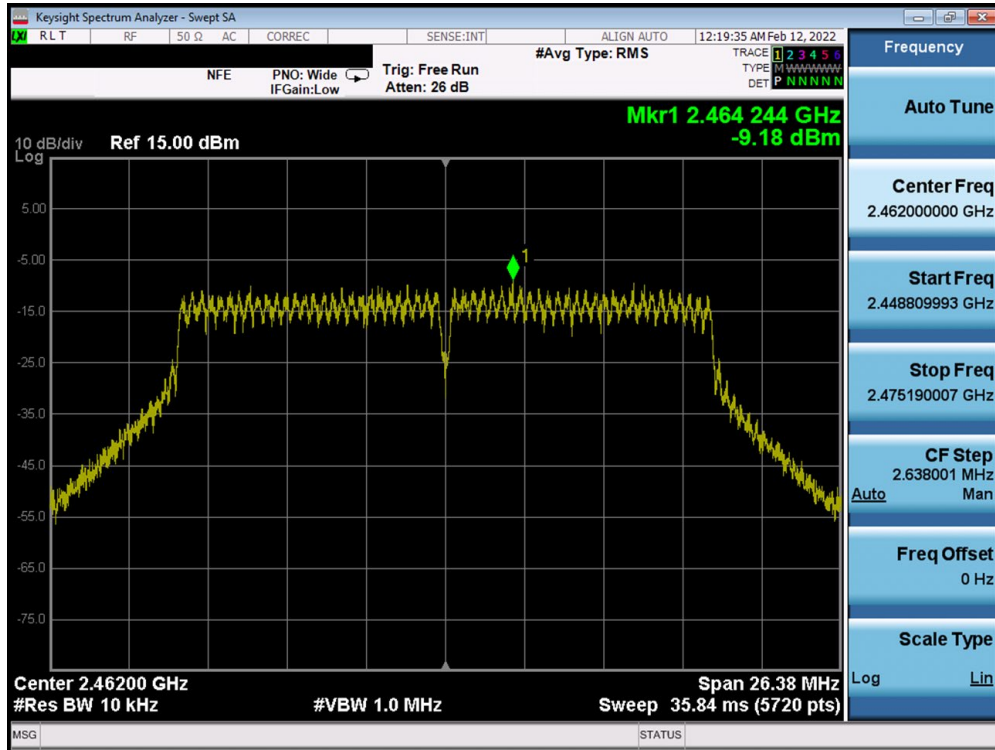
Plot 7-72. Power Spectral Density Plot MIMO ANT2 (802.11n (2.4GHz) – Ch. 11)
