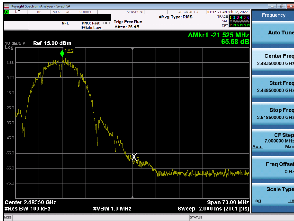
Plot 7-74. Band Edge Plot SISO ANT1 (802.11b – Ch. 11)
