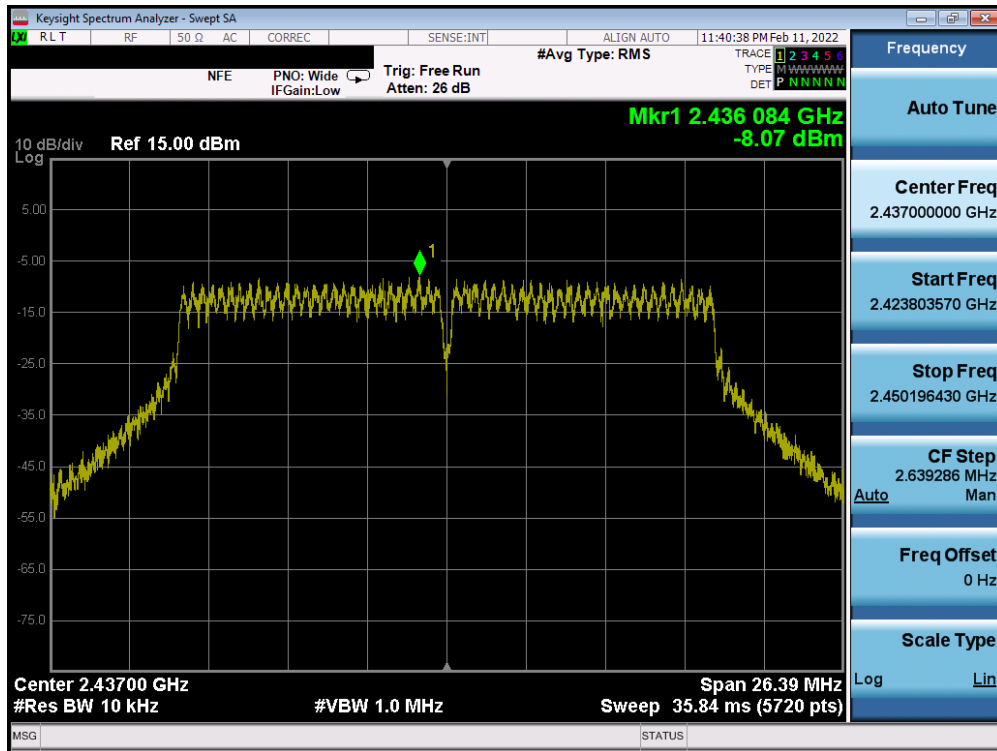
Plot 7-53. Power Spectral Density Plot SISO ANT2 (802.11n (2.4GHz) – Ch. 6)
