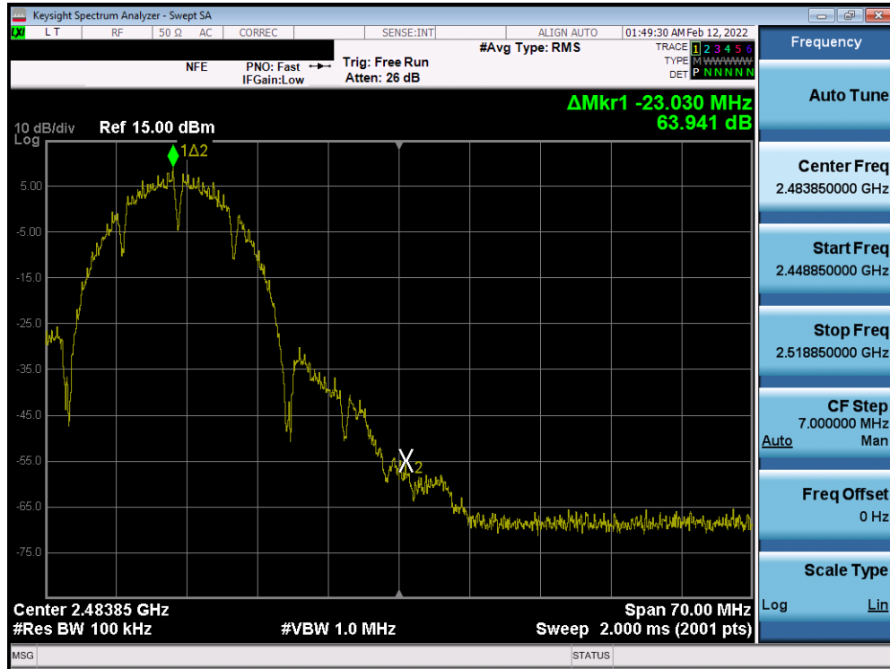
Plot 7-87. Band Edge Plot MIMO ANT1 (802.11b – Ch. 11)
