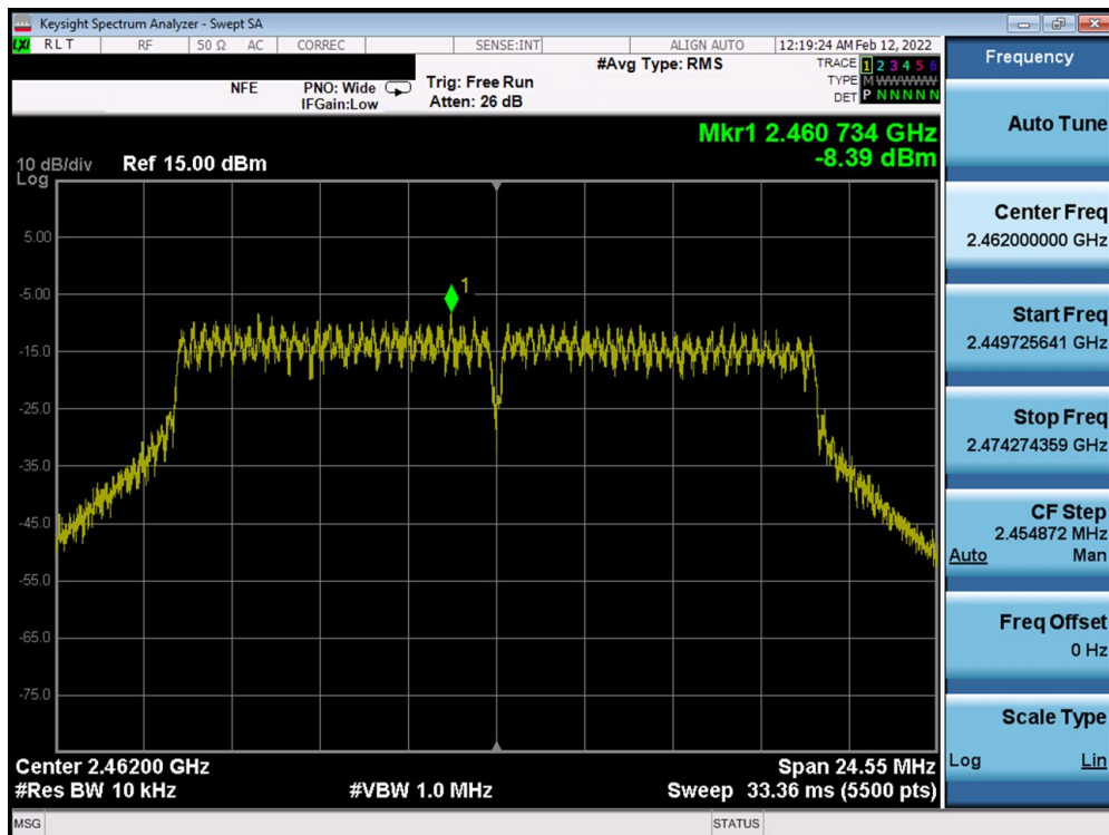
Plot 7-71. Power Spectral Density Plot MIMO ANT1 (802.11n (2.4GHz) – Ch. 11)
