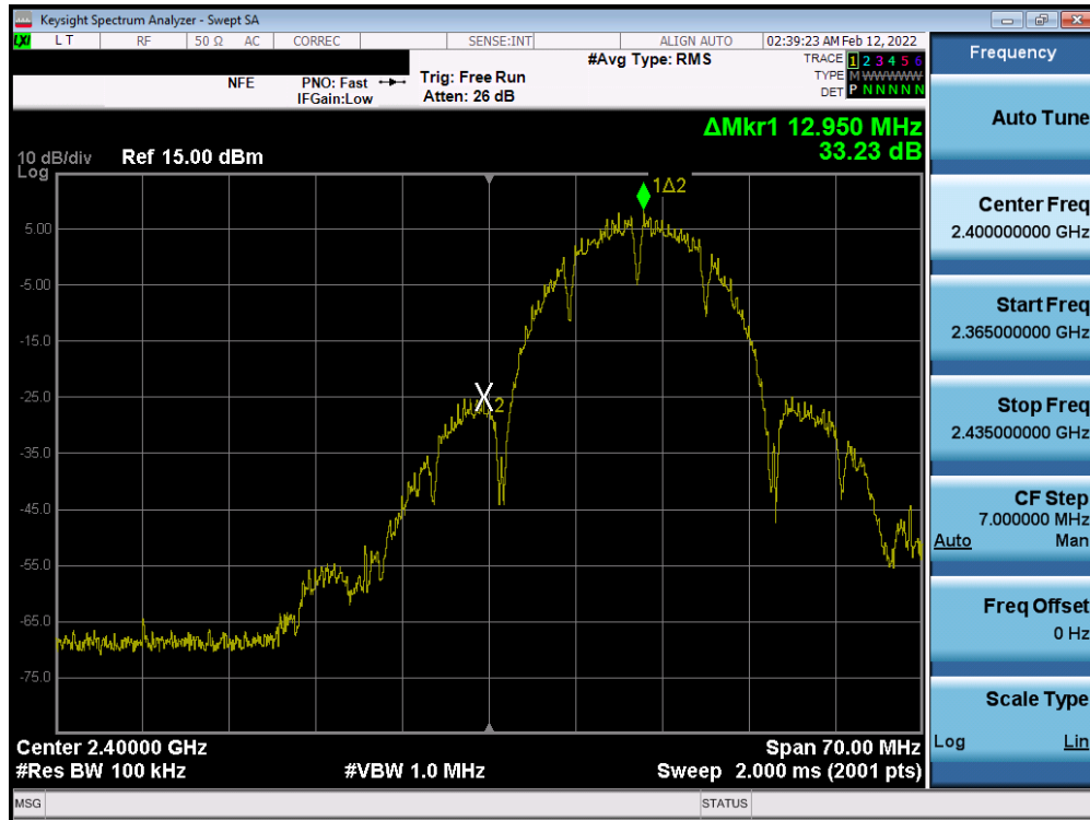
Plot 7-85. Band Edge Plot MIMO ANT1 (802.11b – Ch. 1)
