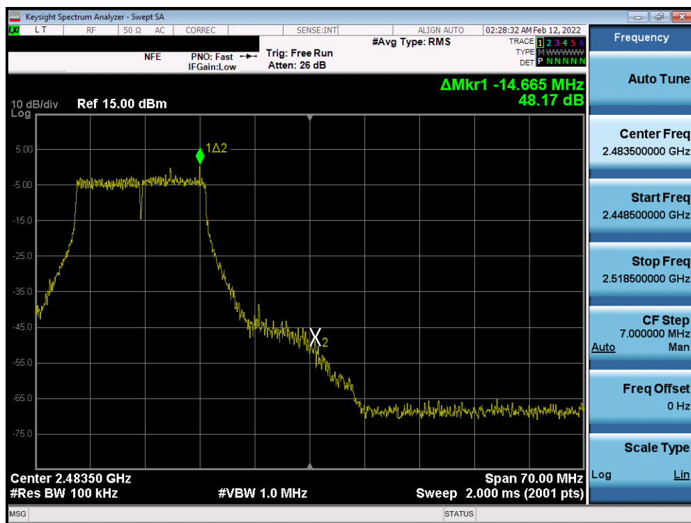
Plot 7-92. Band Edge Plot MIMO ANT2 (802.11g – Ch. 11)
