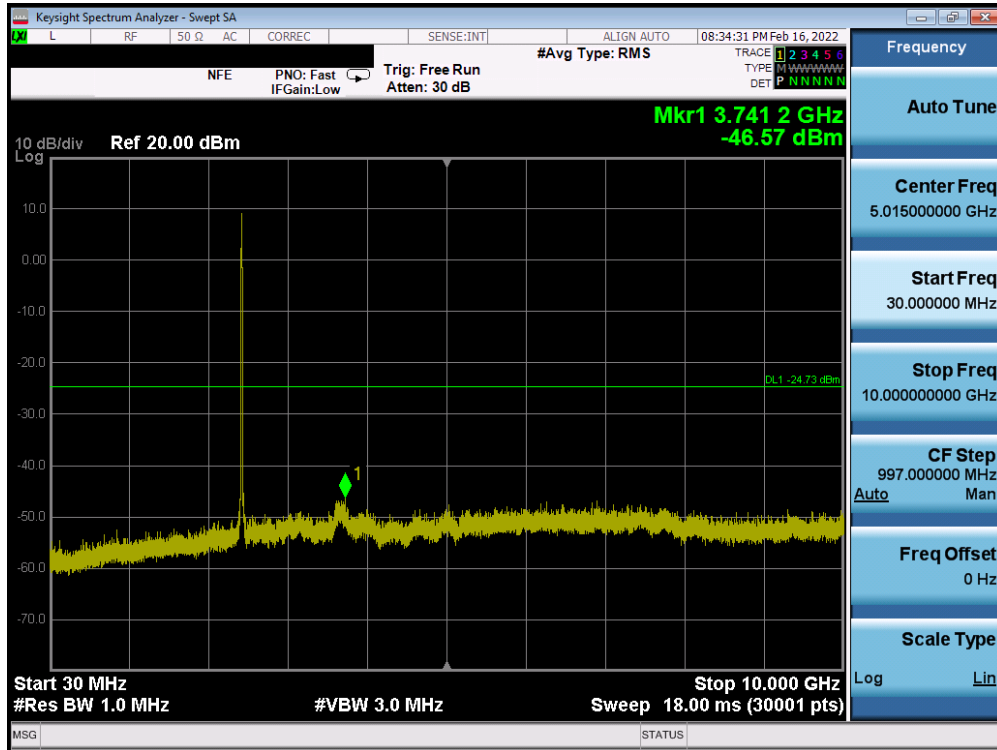
Plot 7-99. Conducted Spurious Plot SISO ANT1 (802.11b – Ch. 6)
