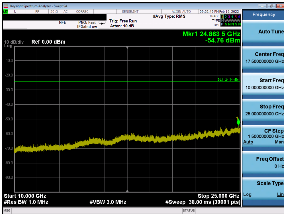
Plot 7-108. Conducted Spurious Plot SISO ANT2 (802.11b – Ch. 11)
