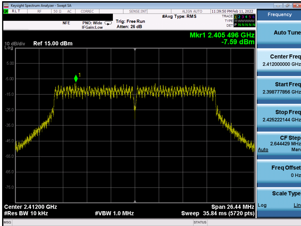
Plot 7-52. Power Spectral Density Plot SISO ANT2 (802.11n (2.4GHz) – Ch. 1)
