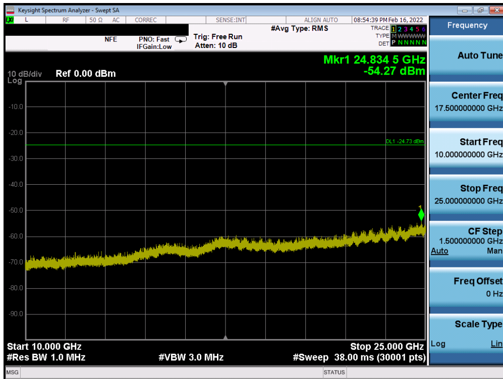
Plot 7-100. Conducted Spurious Plot SISO ANT1 (802.11b – Ch. 6)
