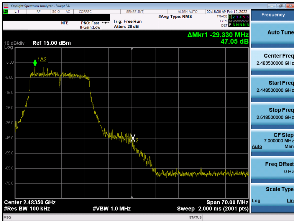
Plot 7-78. Band Edge Plot SISO ANT1 (802.11n (2.4GHz) – Ch. 11)
