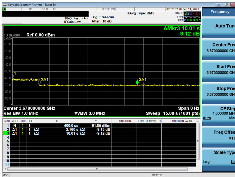
Plot 7-4. Run#2 End User Device Discontinues Operations within 10s
