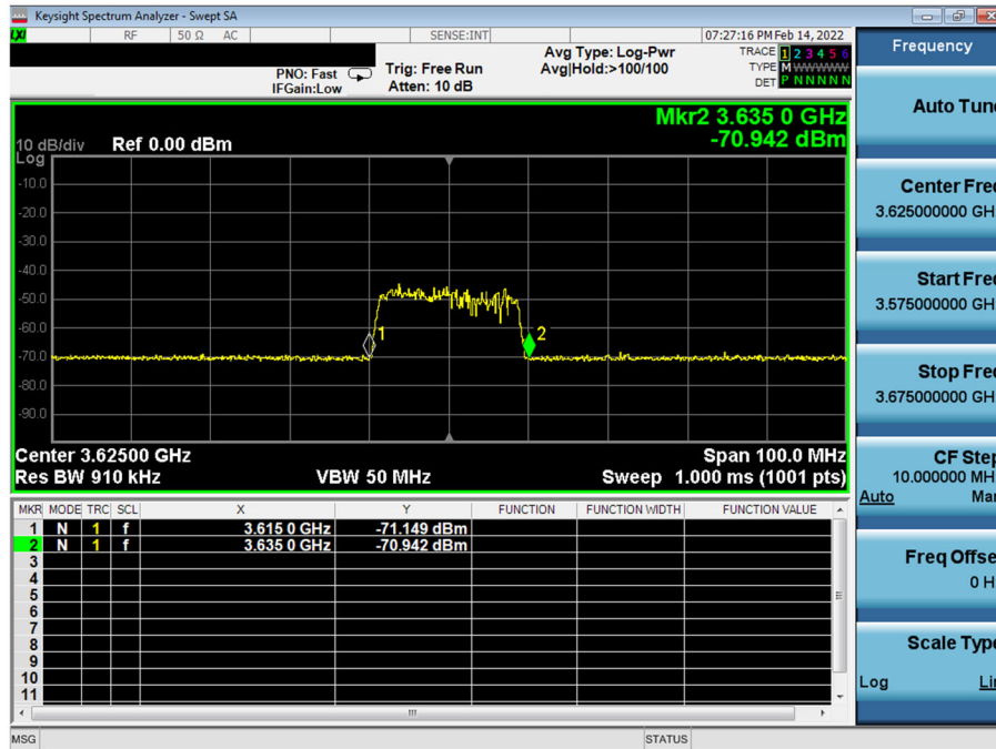
Plot 7-1. Run#1 End User Device Frequency of Operations (3625MHz)
