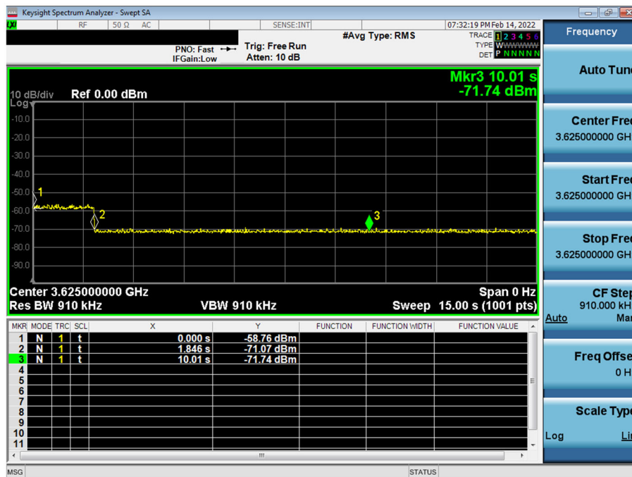
Plot 7-2. Run#1 End User Device Discontinues Operations within 10s
