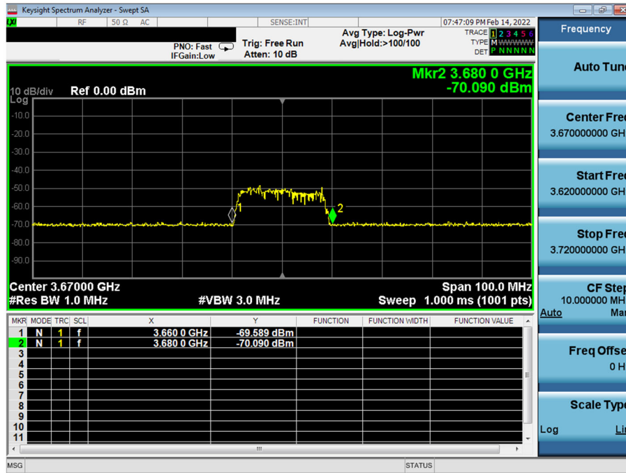
Plot 7-3. Run#2 End User Device Frequency of Operations (3670MHz)
