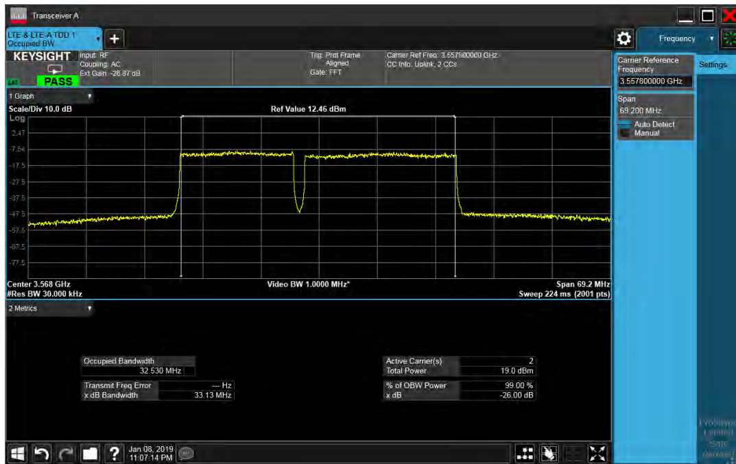
LTE CA intra-band 48 / 35(15+20) / 64QAM - RB Size 175(75+100)
