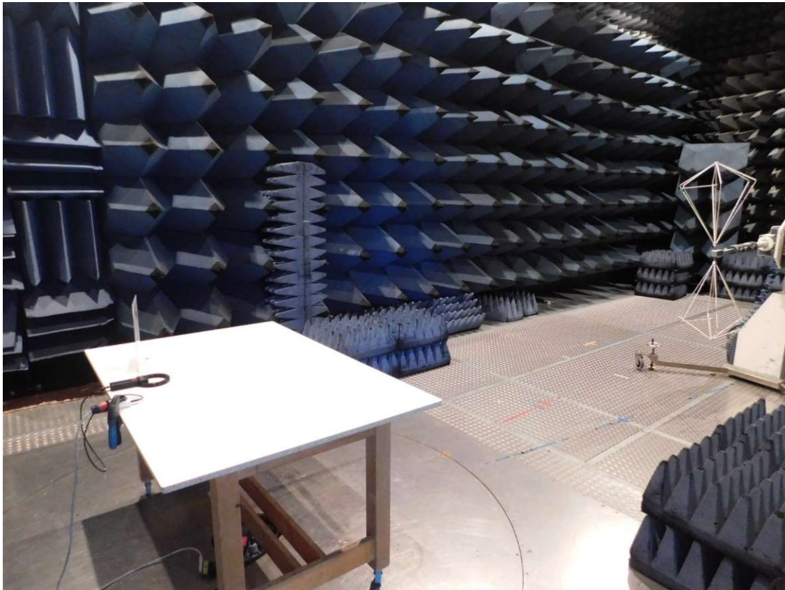
Pre-test setup
