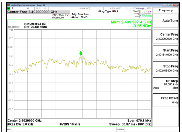
PSD_BLE 1M_LowCH00-2402MHz
