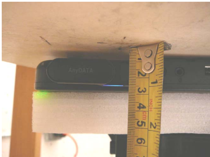
EUT Horizontal-Down with Antenna 270 Degree within 10mm Separation to Flat Phantom with Dell Laptop (Inspiron 1300) Setup Photo
