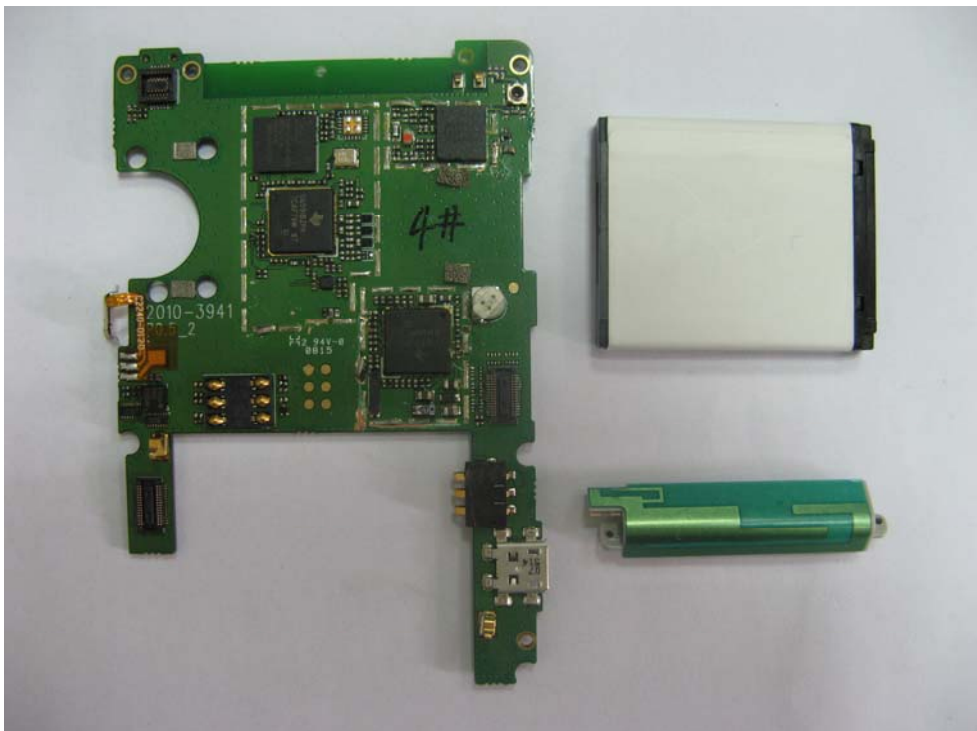
Picture 6: the sample with the assembly—antenna and battery
