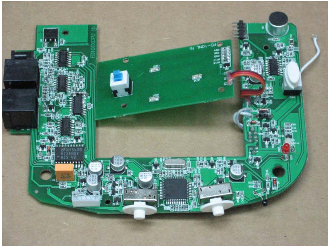
Figure 6: Component side of the FD-10RXCPU and FD-10TX NL card
