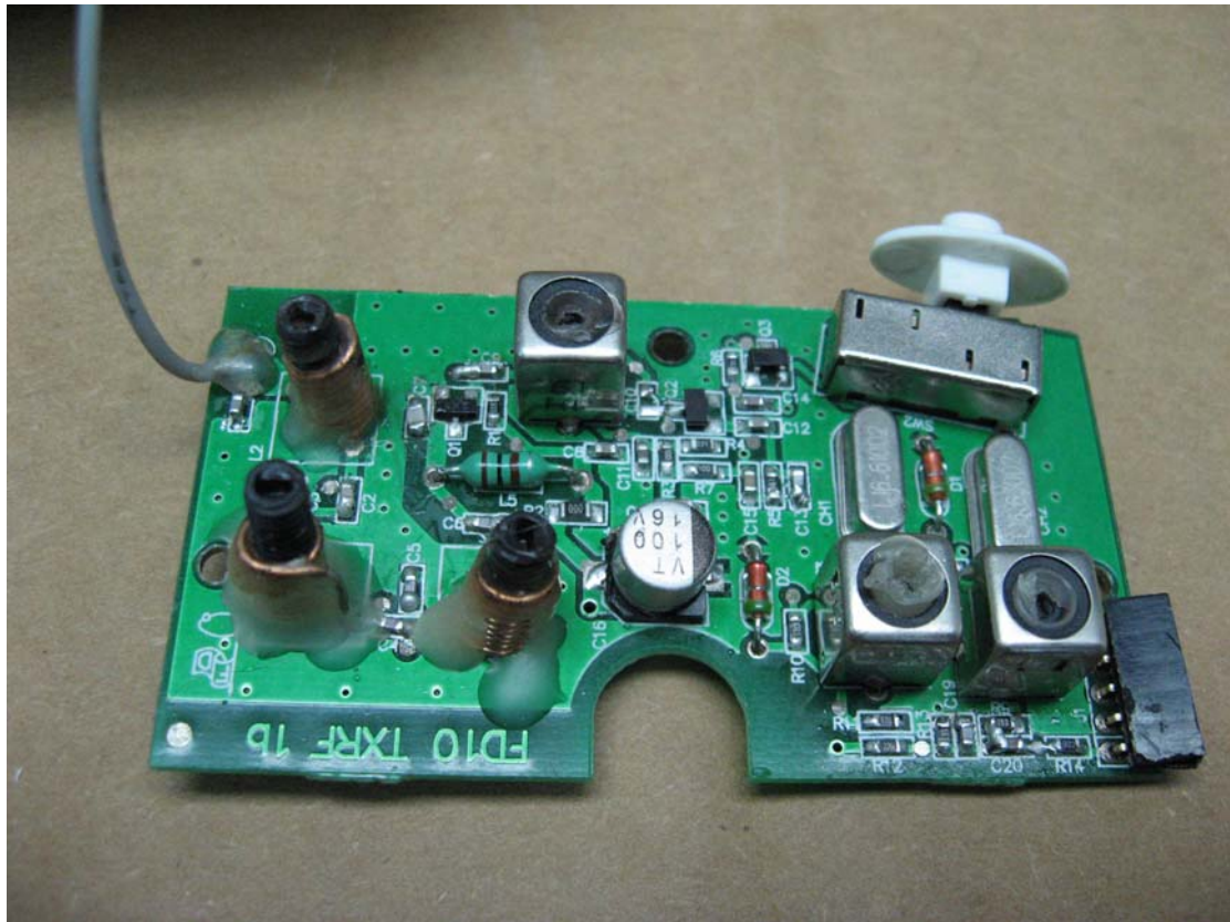
Figure 3: Component side of the FD-10TXRF card
