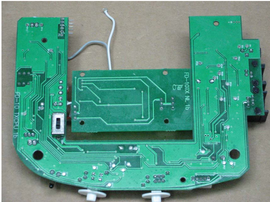
Figure 4: Bottom side of FD-10RXCPU and FD-10TX NL cards
