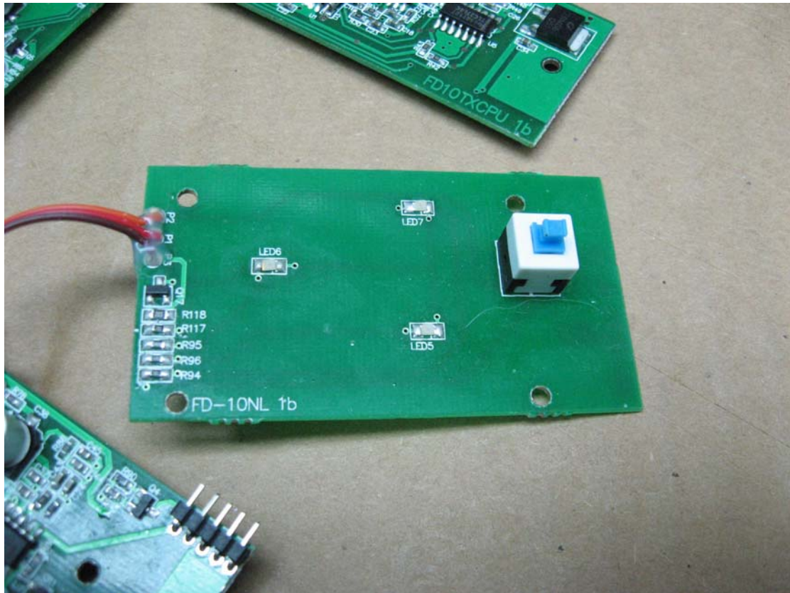
Figure 5: Component side of the FD-10TX NL card
