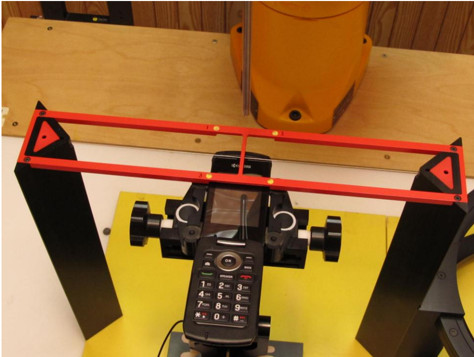
Figure 1a – HAC Tcoil Emission Test Setup
