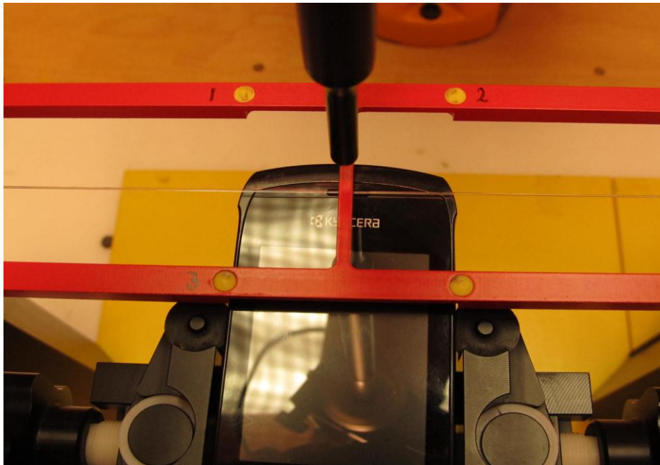
Figure 1b – HAC RF Emission Test Setup
