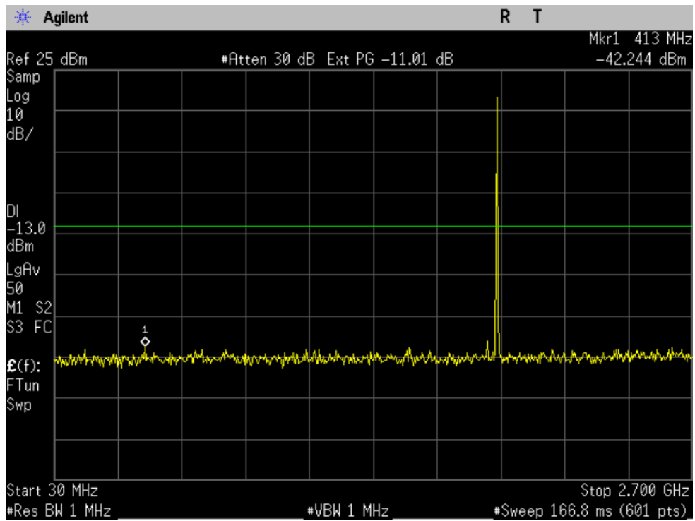
Figure 10-8a CDMA 1900 - Conducted Spurious Emission (CH 600)
