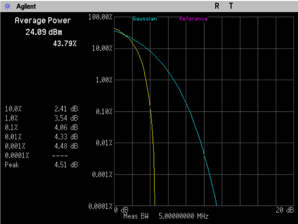
Figure 8-2 CCDF @ CH 600
