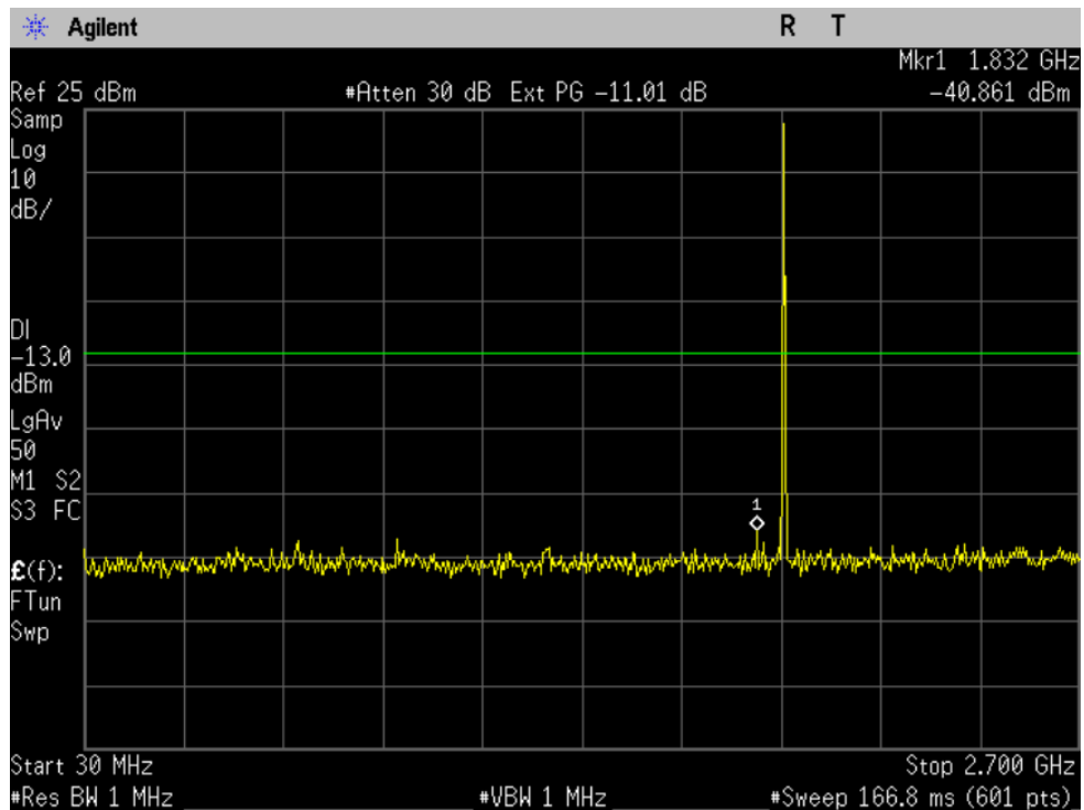
Figure 10-9a CDMA 1900 - Conducted Spurious Emission (CH 1175)
