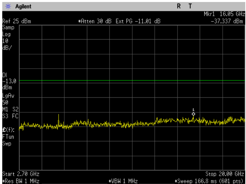
Figure 10-9b CDMA 1900 - Conducted Spurious Emission (CH 1175)
