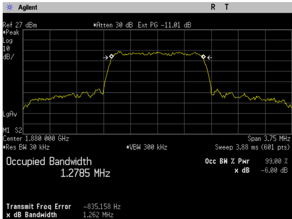
Figure 9-7 CDMA 1900 @ CH 600
