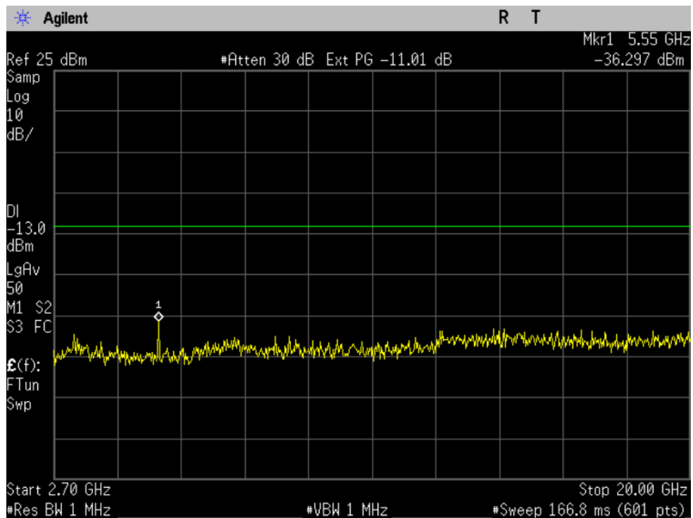
Figure 10-7b CDMA 1900 - Conducted Spurious Emission (CH 25)
