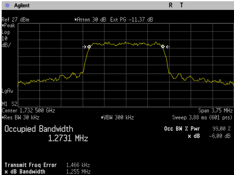
Figure 9-4 AWS 1700 @ CH 450
