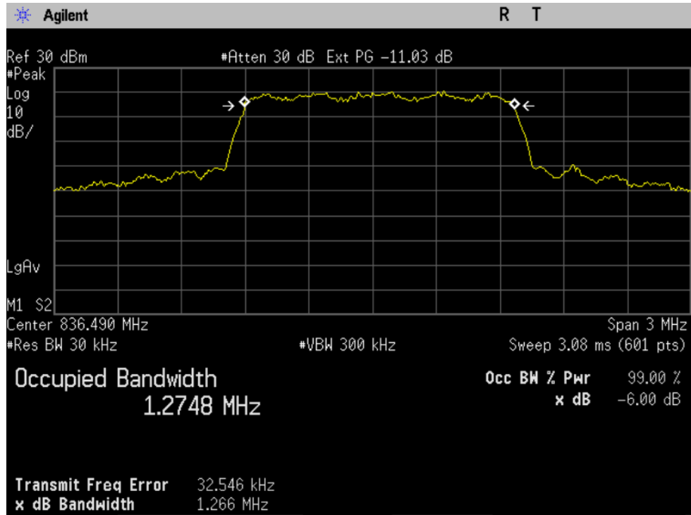
Figure 9-1 CDMA 800 @ CH 384
