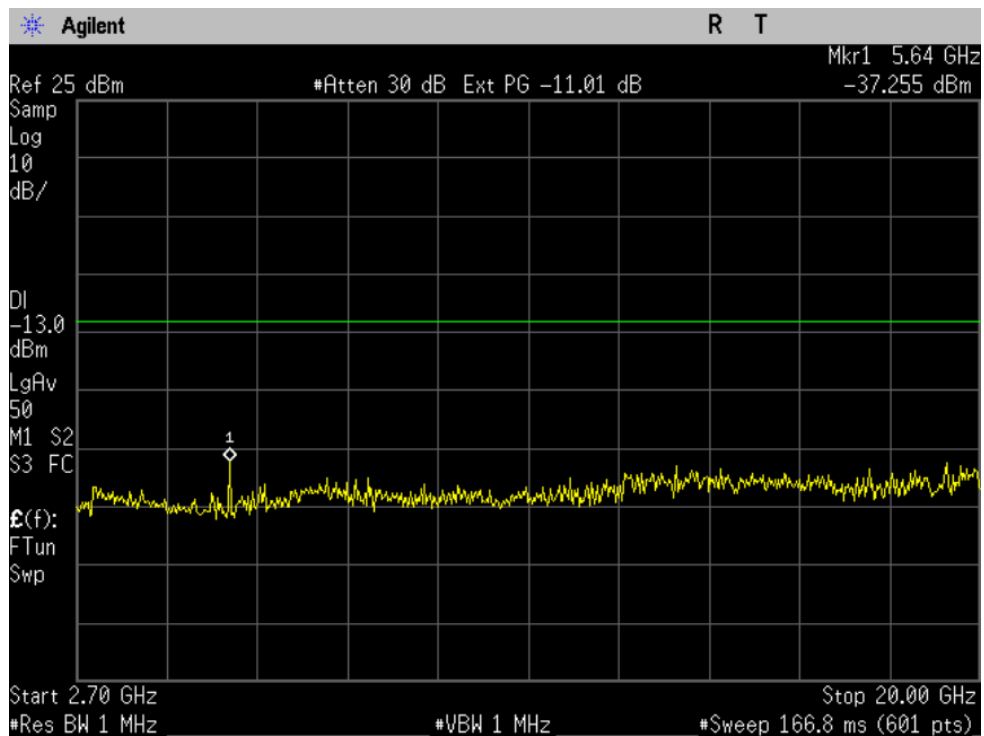
Figure 10-8b CDMA 1900 - Conducted Spurious Emission (CH 600)
