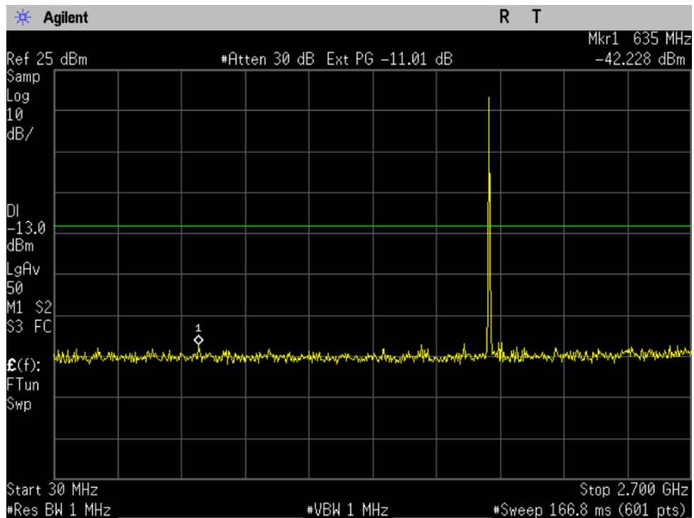
Figure 10-7a CDMA 1900 - Conducted Spurious Emission (CH 25)
