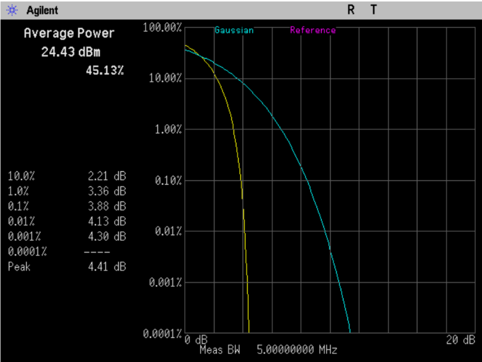
Figure 8-1 CCDF @ CH 450
