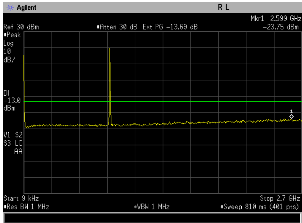
Figure 9-2a CDMA 800 – Conducted Spurious Emission (CH 383)
