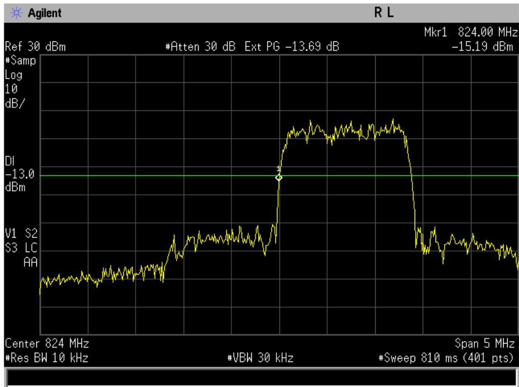
Figure 8-2 CDMA 800 Lower Band Edge @ CH 1013
