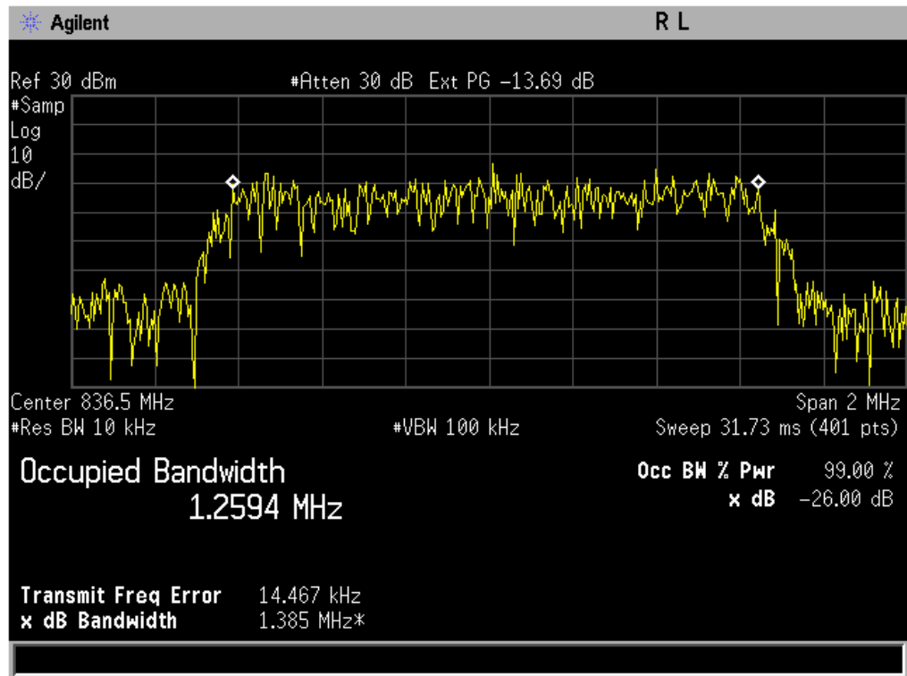
Figure 8-1 CDMA 800 @ CH 383
