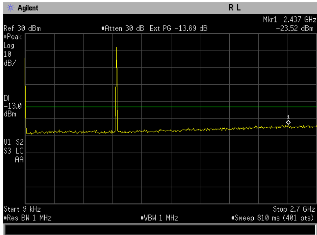
Figure 9-3a CDMA 800 – Conducted Spurious Emission (CH 777)
