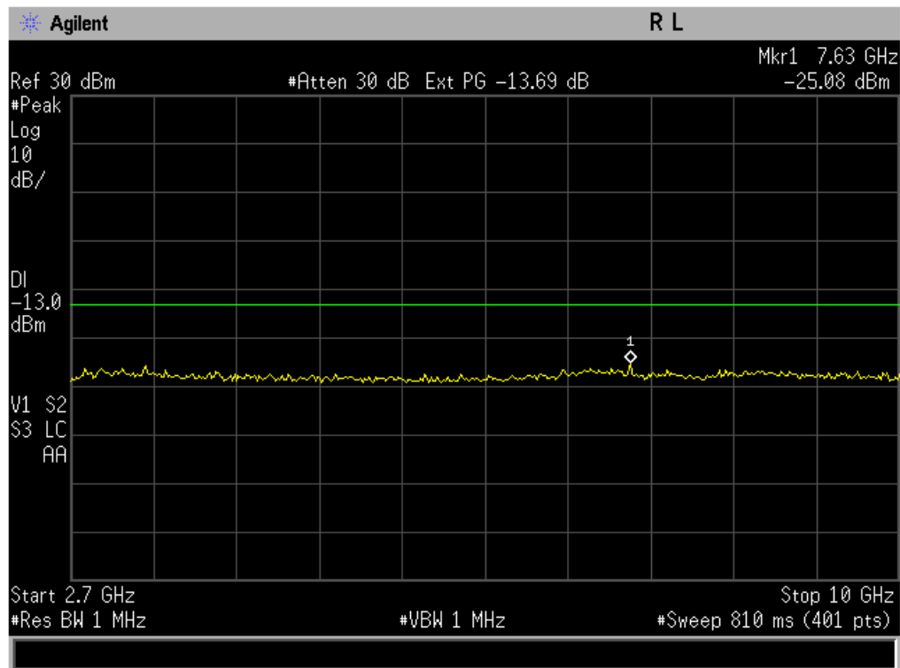
Figure 9-2b CDMA 800 – Conducted Spurious Emission (CH 383)
