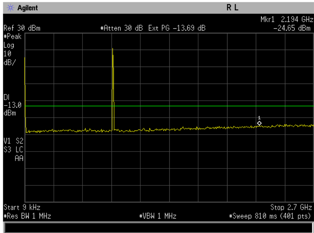
Figure 9-1a CDMA 800 – Conducted Spurious Emission (CH 1013)
