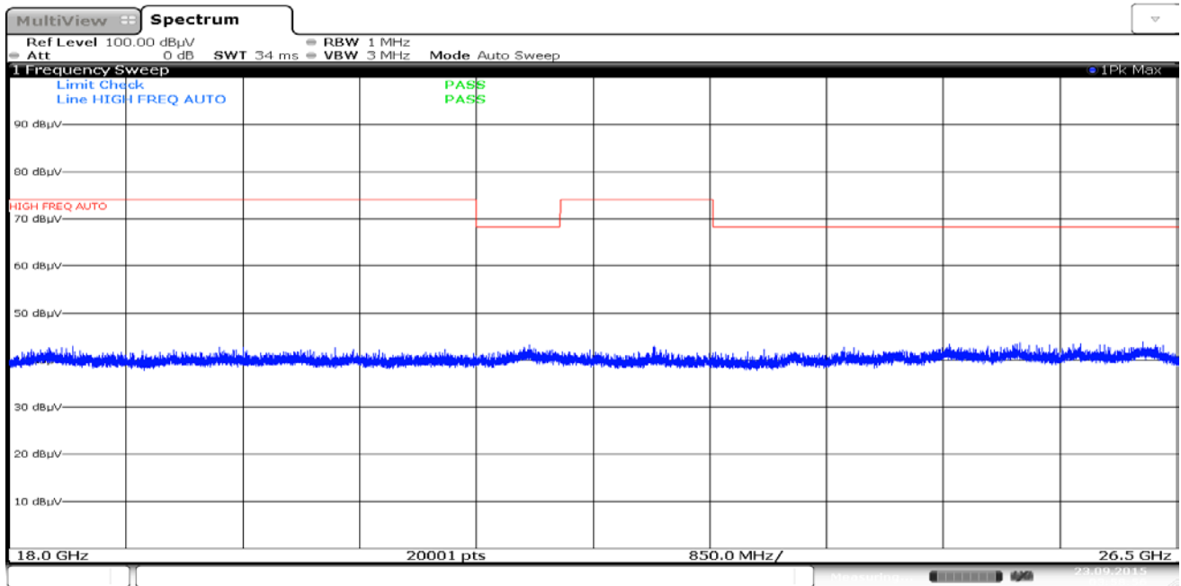
Plot 6-49. Radiated Spurious Plot above 18GHz (Pol. V)
