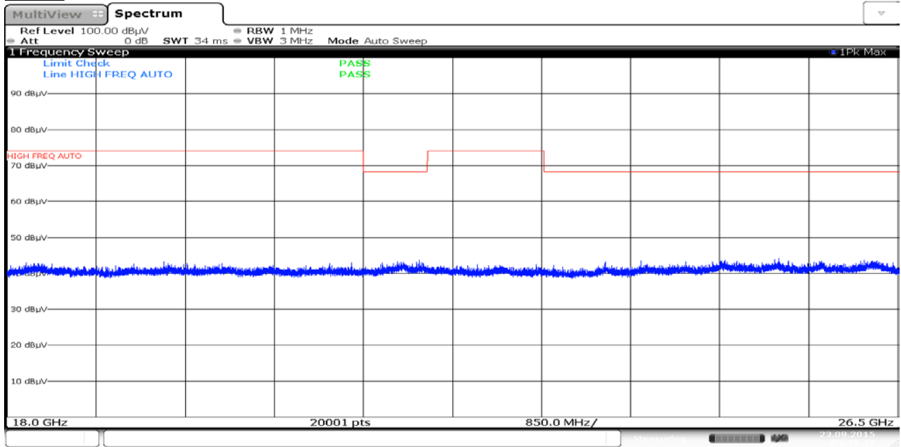
Plot 6-48. Radiated Spurious Plot above 18GHz (Pol. H)
