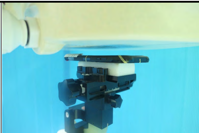
Rear Face of EUT Tested at 15 mm
