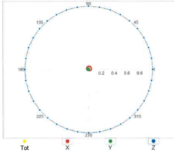
f=1800 MHz,R22,90°
