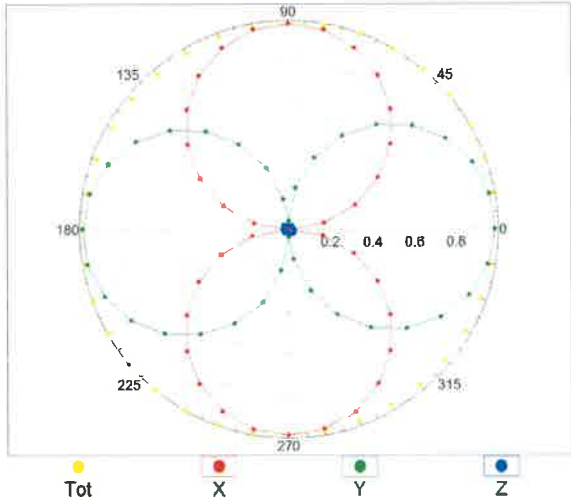
f=1800 MHz,R22,0°
